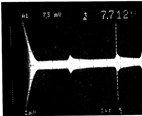
Fig. 4.2: Signals in the case of an overhead wire at 635 m and a tree at 1155 m
