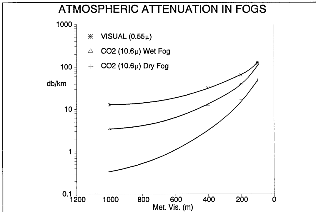
Figure 6 Fog Penetration
