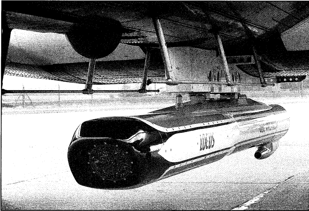
Figure 3 Locus Pod
