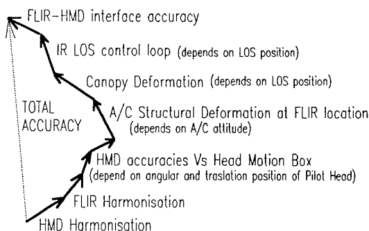
Figure 3. Graphic presentation of the HMD-IR Sensor LOS alignment error in the SIRPH mode. The total angle accuracies are the sum of many factors which are never constants.
