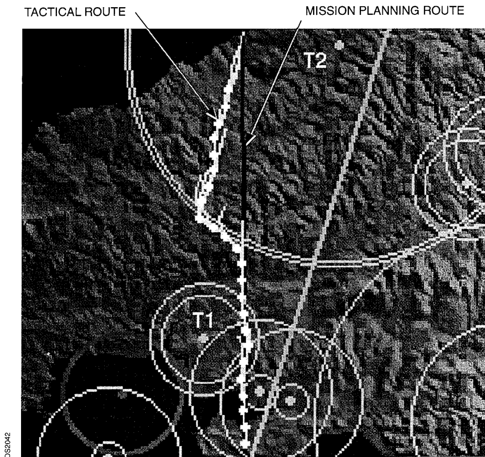
Fig. 16 Tactical route
