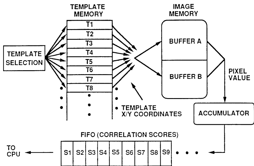
FIGURE 5. BASIC STRUCTURE OF THE CORRELATION MODULE
