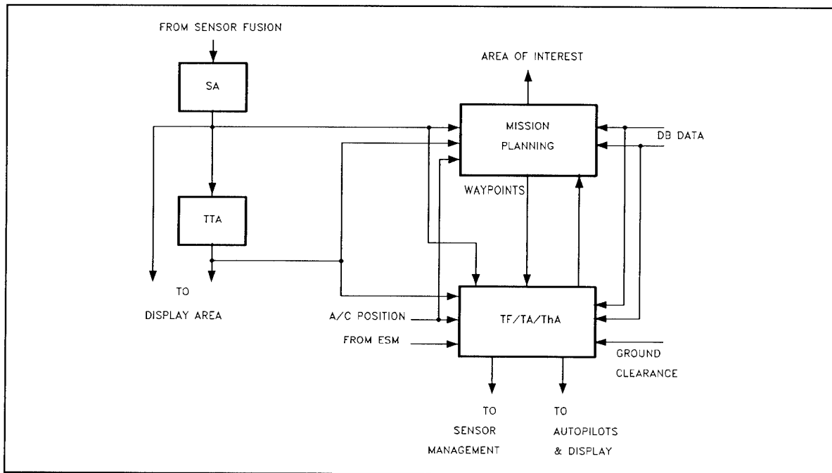
Fig. 4 - Mission Area
