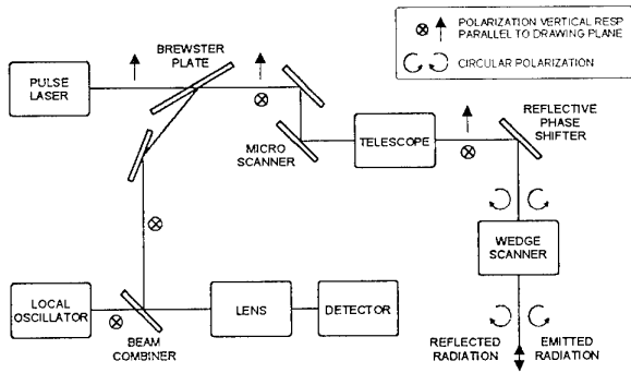
Fig. 4.1: Block diagram of the CO 2 -heterodyne laser radar
