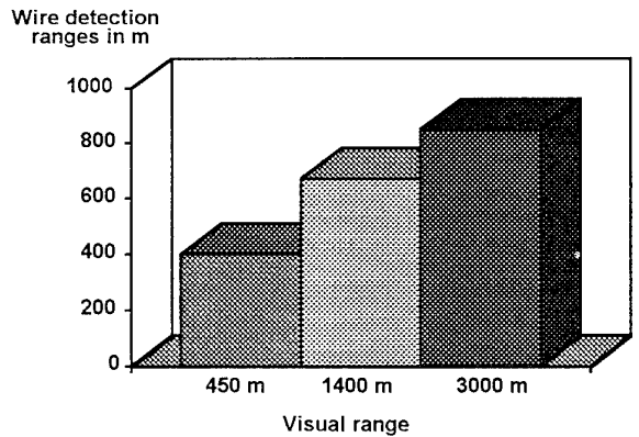
Fig. 5.4: Ranges of a hypothetical system against 5 mm wires with 10 kW pulse power for visual ranges of 450 m, 1400 m and 3000 m.
