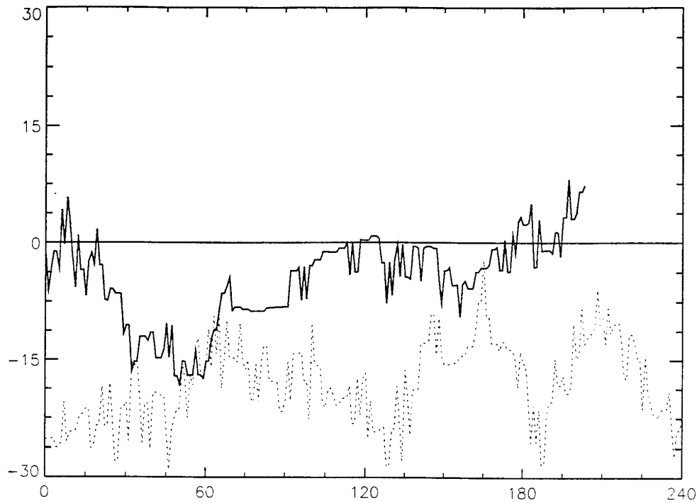
FIGURE 8. CROSSRANGE TRACKING ERROR (METERS) vs. VIDEO FRAME NUMBER
