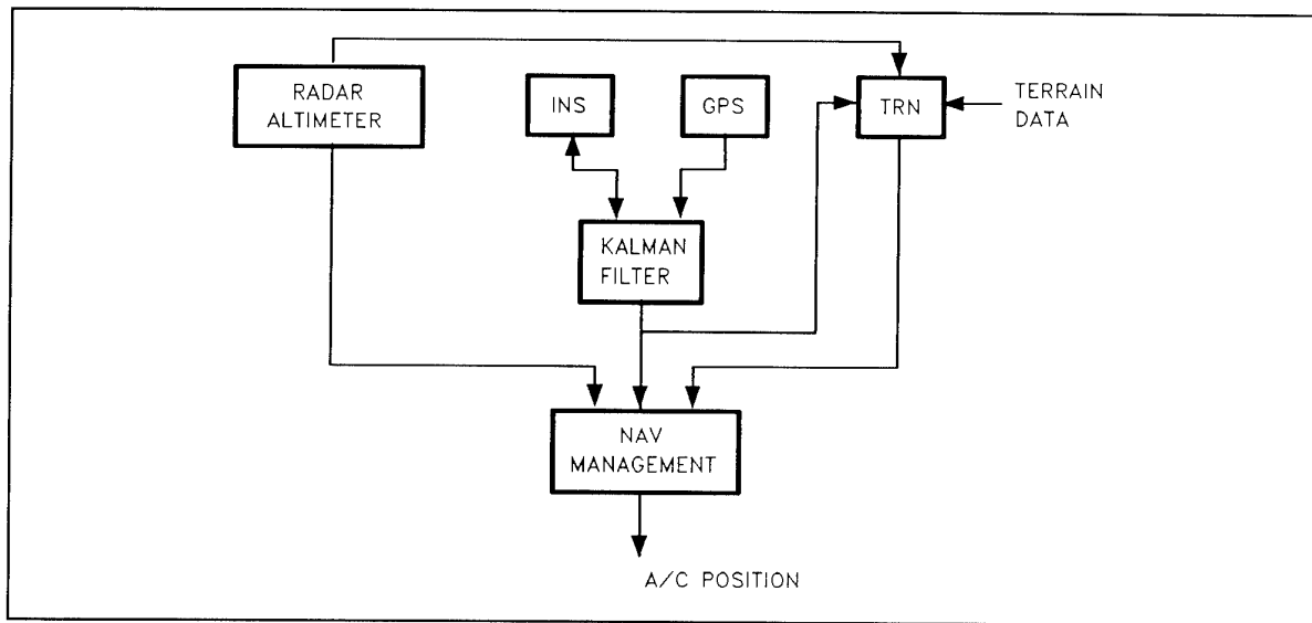
Fig. 6 - Navigation Area
