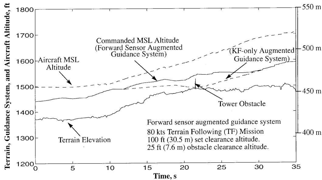
Fig.9. Flight Test Vertical Profile with Tower Obstacle.
