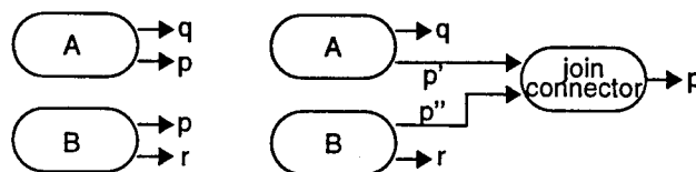
Figure 3: Joining multiple outputs into a single input
