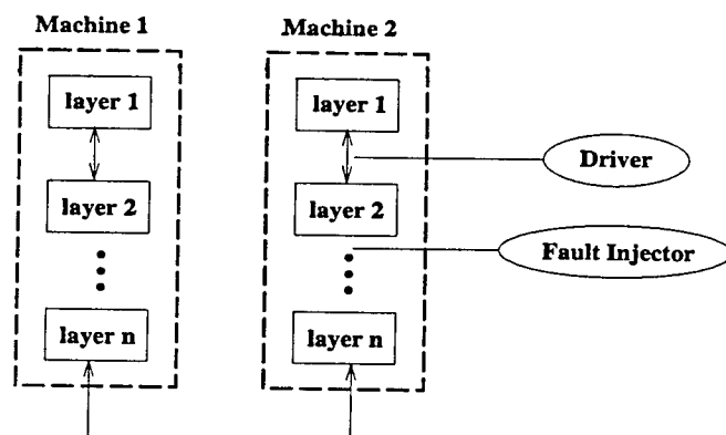
Figure 1: Protocol Stacks.
