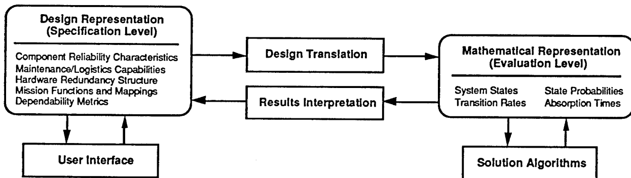
Figure 1: Multi-Level Design Assessment in SDAT
