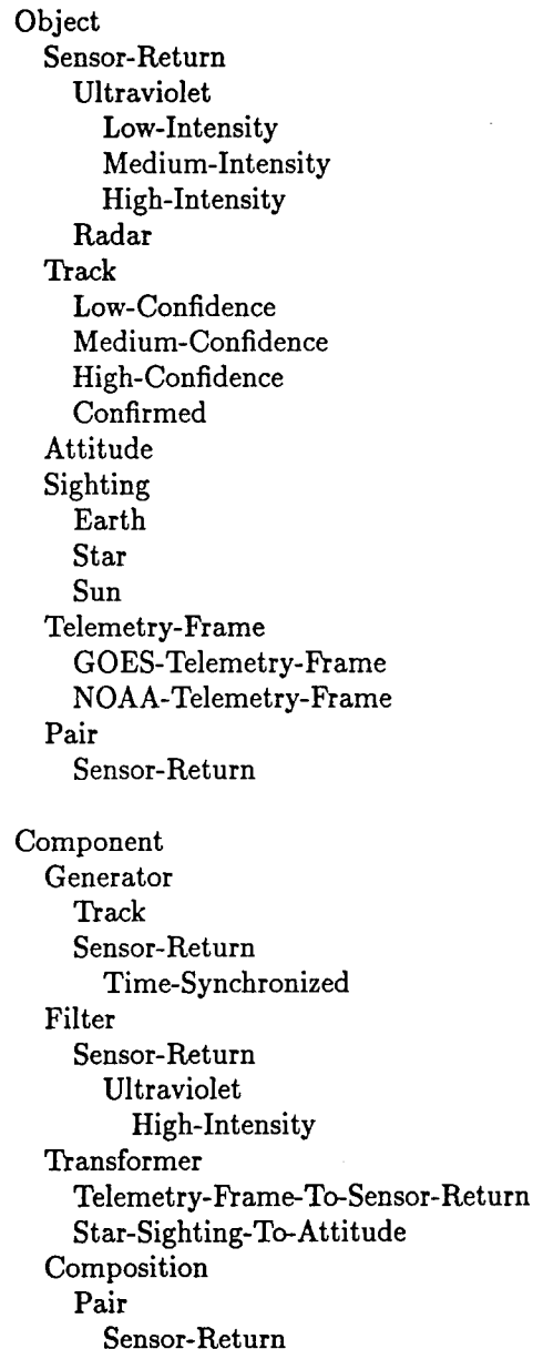
Figure 9: A Portion of the Satellite Telemetry and Tracking Domain Model for Weaves
