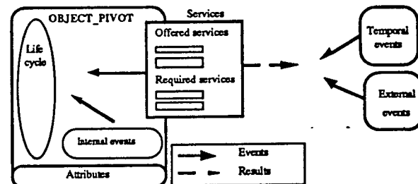
Figure 5: OBJECT_PIVOT Structure
