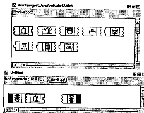
Figure 7: An example of an Onika job dictionary (above) and application workspace.
