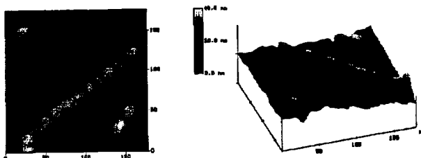
FIGURE 1. STM image of the narrowest nickel line obtained to date: 24 nm wide, 14 nm high and 200 nm long. The smaller dots near the corners are surface contamination. The writing parameters are: 18.7 V, 1.6 nA, and 500 nm/s writing speed.
