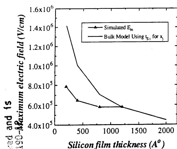
Fig. 1 The maximum channel electric field, by using t_{si} for x_j in the model for the bulk MOSFET, and by SPICES simulation.
