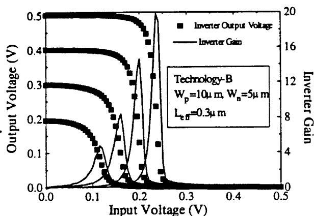
Fig. 6 Inverter DC transfer characteristics. PMOS and NMOS devices forming the inverter are VT MOS.
