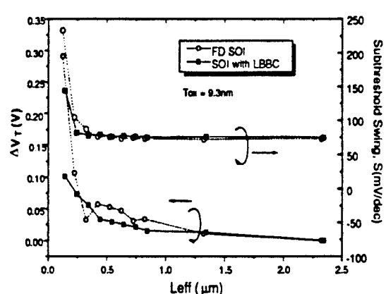
Fig. 12: PMOSFET threshold voltage shift ( \Delta V_T ) and subthreshold swing (S) versus effect channel length at V_{ds} = -0.05V
