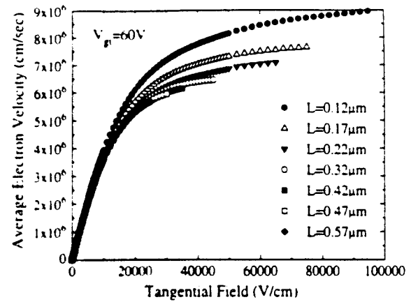
Fig. 3. Measured electron drift velocity versus applied tangential field. Device channel length is used as a parameter. V_g = V_{fg} - V_{bg} = 60 \text{ V} .
