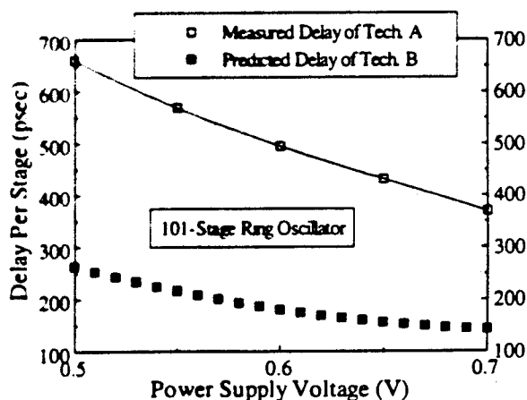
Fig. 5 Delay of a 101-stage ring oscillator. The PMOS and NMOS devices in the ring are VT MOS with T_{ox}=10\text{nm} , and L_{eff}=0.3\mu\text{m} , V_{t0}=0.6\text{V} . Solid Squares show the predicted delay for a ring oscillator based on Tech-B with L_{eff}=0.3\mu\text{m} .
