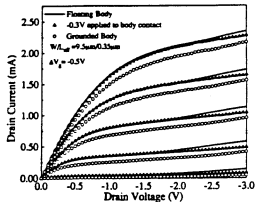
Fig. 6. I - V characteristics of a four-terminal device that has body contact. Solid lines show I - V when body is floating. Circles are used for the grounded body, and solid triangles are used when -0.3 V is applied to body contact. Each V_g step is -0.5 V.
