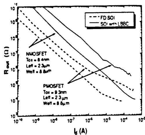
Fig. 5: Comparison of output resistance between SOI with Low-Barrier Body-Contact and fully-depleted SOI
