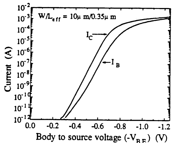
Fig. 12 A four terminal SOI PMOSFET operated as a PNP transistor. Current gain > 30.
