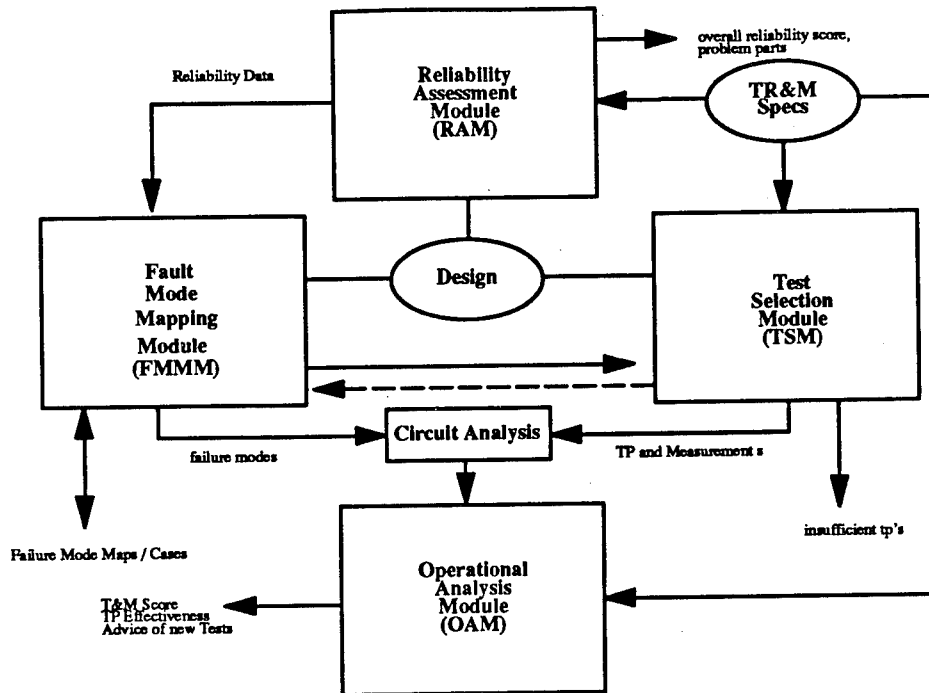
Figure 13 System concept.
