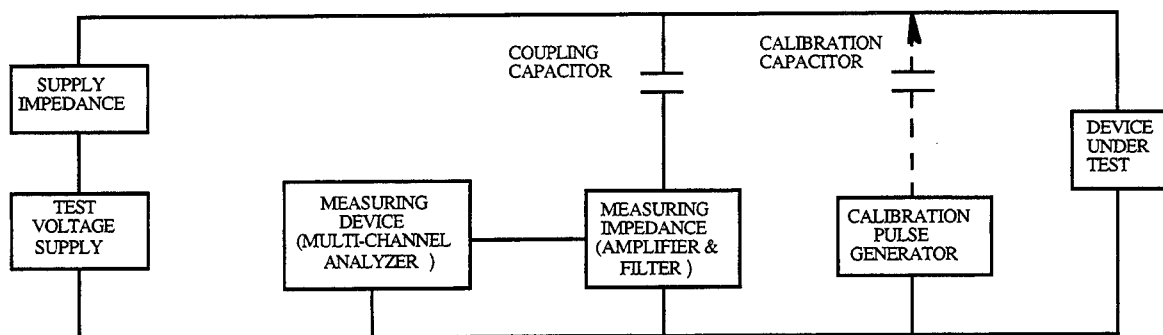
Figure 3. Test Schematic
