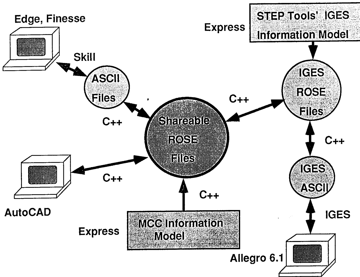
Figure 1. Architecture of the MOST system.
