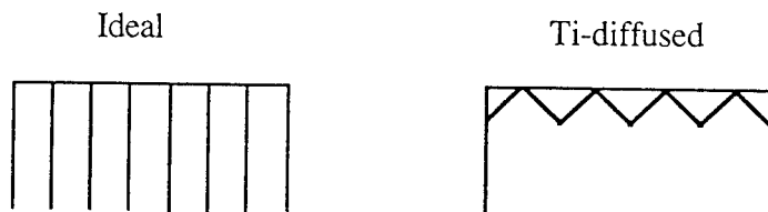
Figure 8. Schematic diagram comparing ideal and titanium diffused domain inversion gratings. The domain angle commonly achieved with the "standard" diffusion process is between 90^\circ and 120^\circ .
