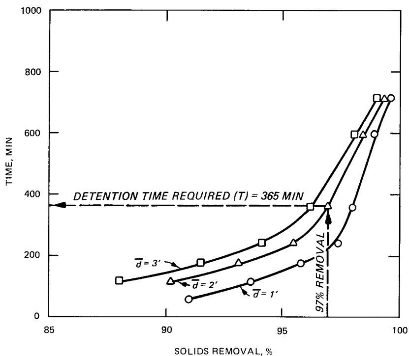
Figure 2. Settling data for dredged material
