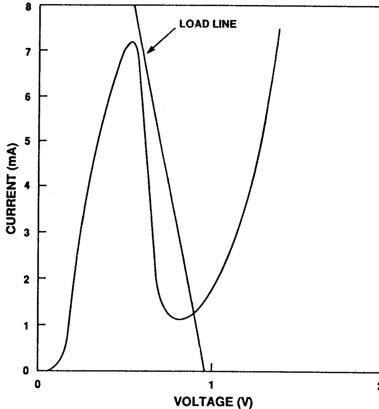
Fig. 8. Current-voltage characteristic of RTD modeled as relaxation oscillator. The straight line shows the dc load line presented to the RTD after the application of the start-up ramp.
