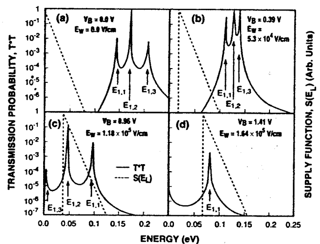
FIG. 3. Transmission probability (solid curve) and supply function (dashed curve) for the triple-well RTD at specific bias voltages across the active region of the device. (a) V_B=0.0 , (b) V_B=0.39 V, (c) V_B=0.96 V, and (d) V_B=1.41 V. A uniform electric field E_W was assumed to exist across the triple-well structure.
