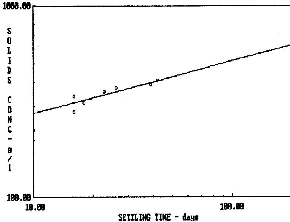
Figure 2. Example plot of compression settling data
