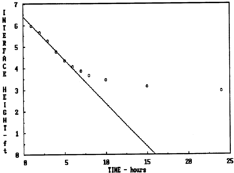
Figure 4. Example plot of zone settling data
