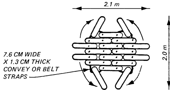
PLAN SCHEMATIC OF ONE FTB MODULE
