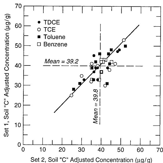
Figure 2. Youden two-sample plot for four analytes in soil C as reported by 10 laboratories (laboratories 3 and 12 excluded). Concentrations of the 10 pairs of results for TCE and Tol were adjusted to 39.5 µg/g (both TDCE and Ben had this mean) by subtracting 16.7 and 24.0 µg/g, respectively.
