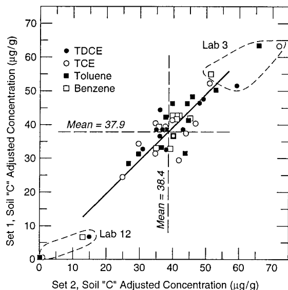
Figure 1. Youden two-sample plot for four analytes in soil C as reported by 12 laboratories. Concentrations of the 12 pairs of results for TDCE, TCE and Tol were adjusted to the same mean as Ben by subtracting 0.3, 18.4 and 23.4 µg/g, respectively, to permit plotting on a single graph.
