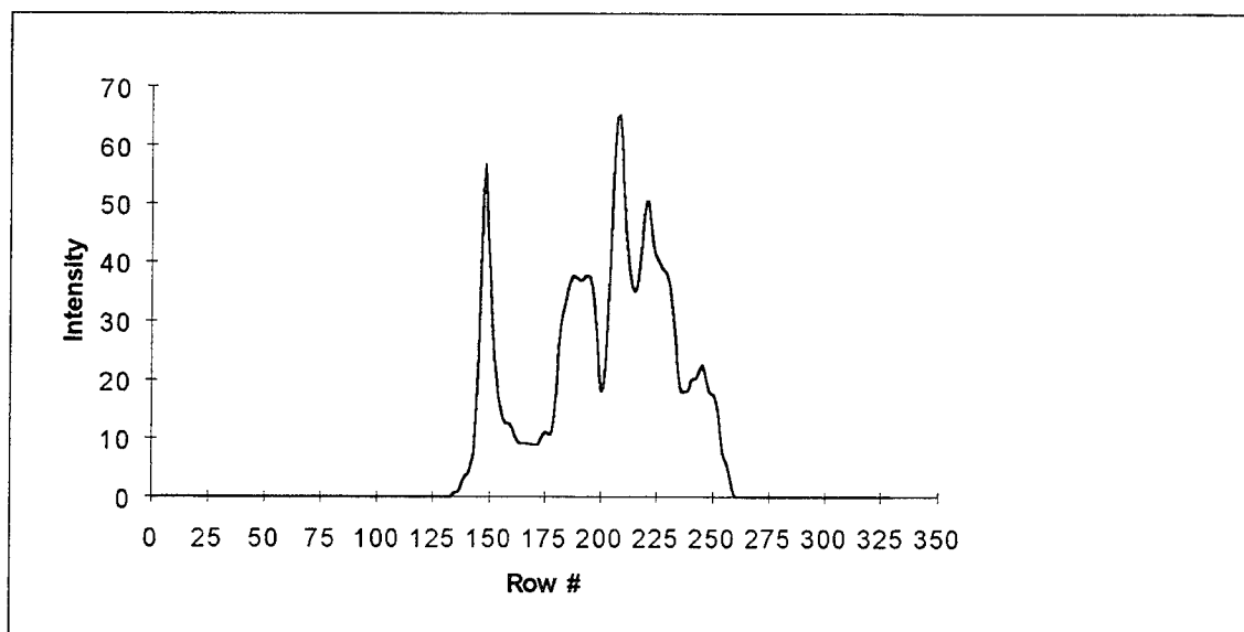
Fig. C-29. Complement of H2 squashed to preserve vertical sequences
