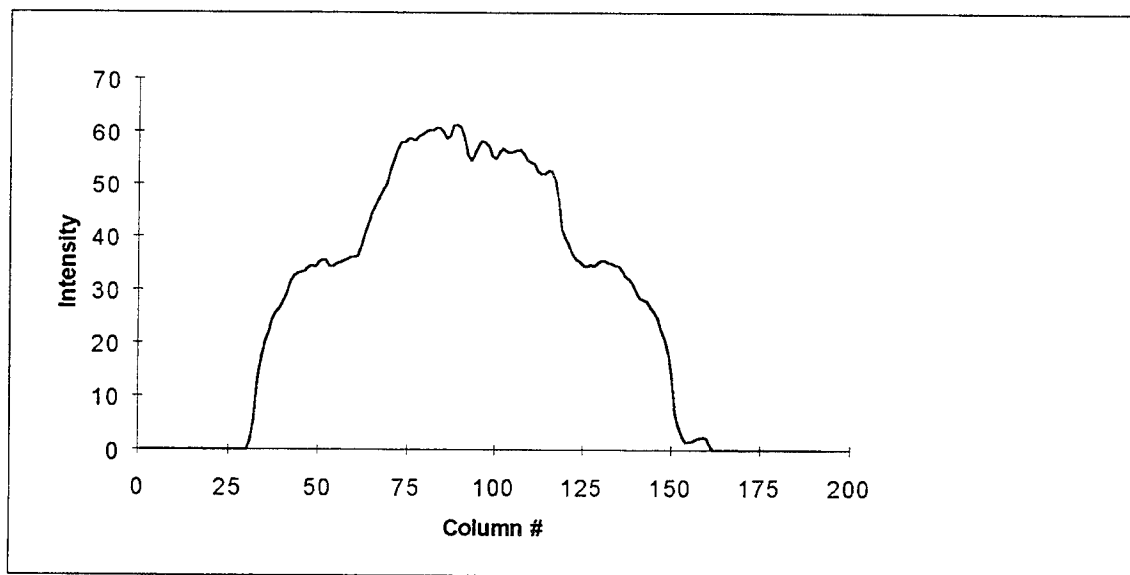
Fig. D-89. Complement of T7 squashed to preserve horizontal sequences
