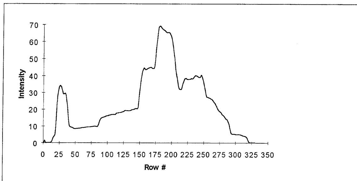
Fig. C-84. Complemented reflection of H5 squashed to preserve vertical sequences
