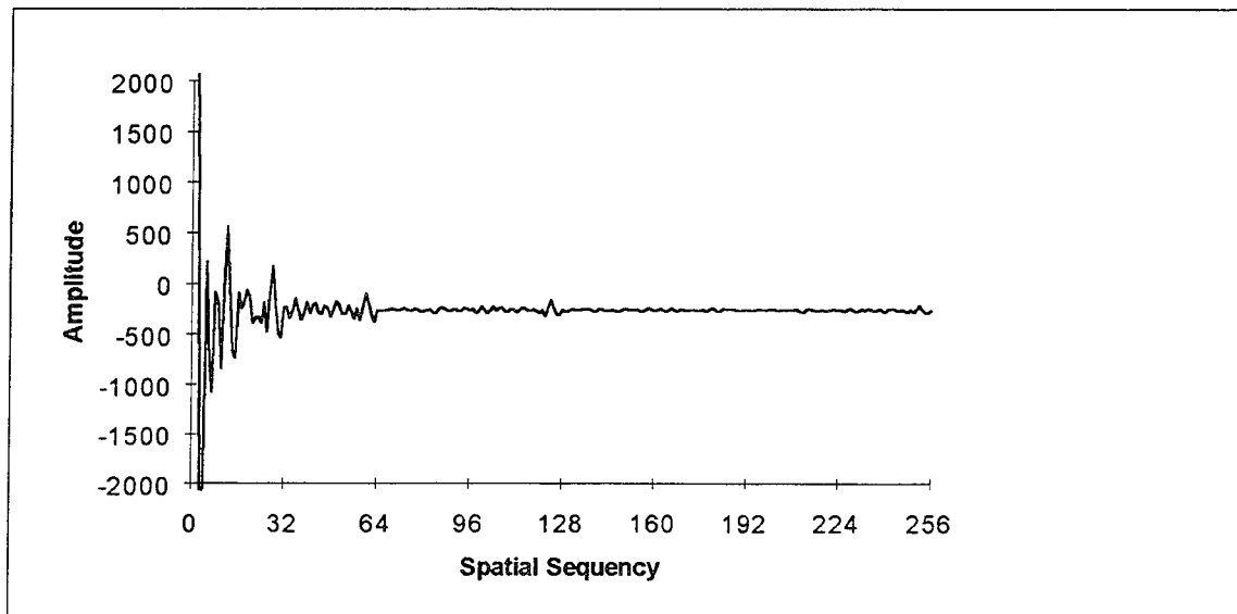
Fig. D-179. Walsh transform of Fig. D-178
