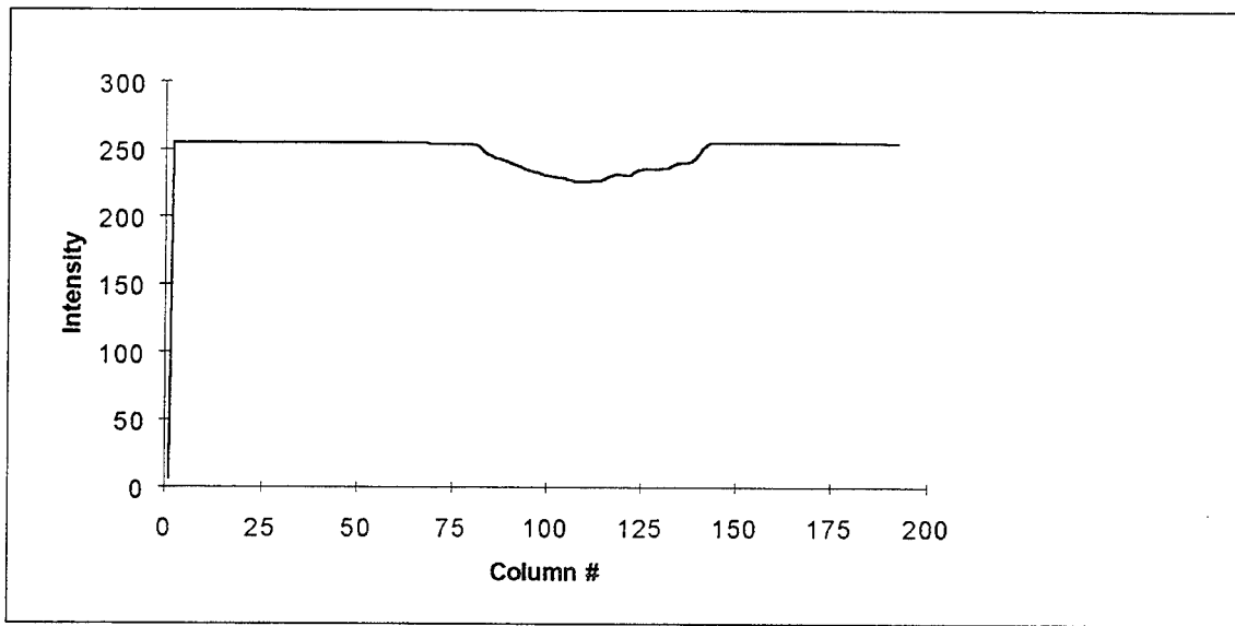
Fig. D-210. Reflection of T15 squashed to preserve horizontal sequencies
