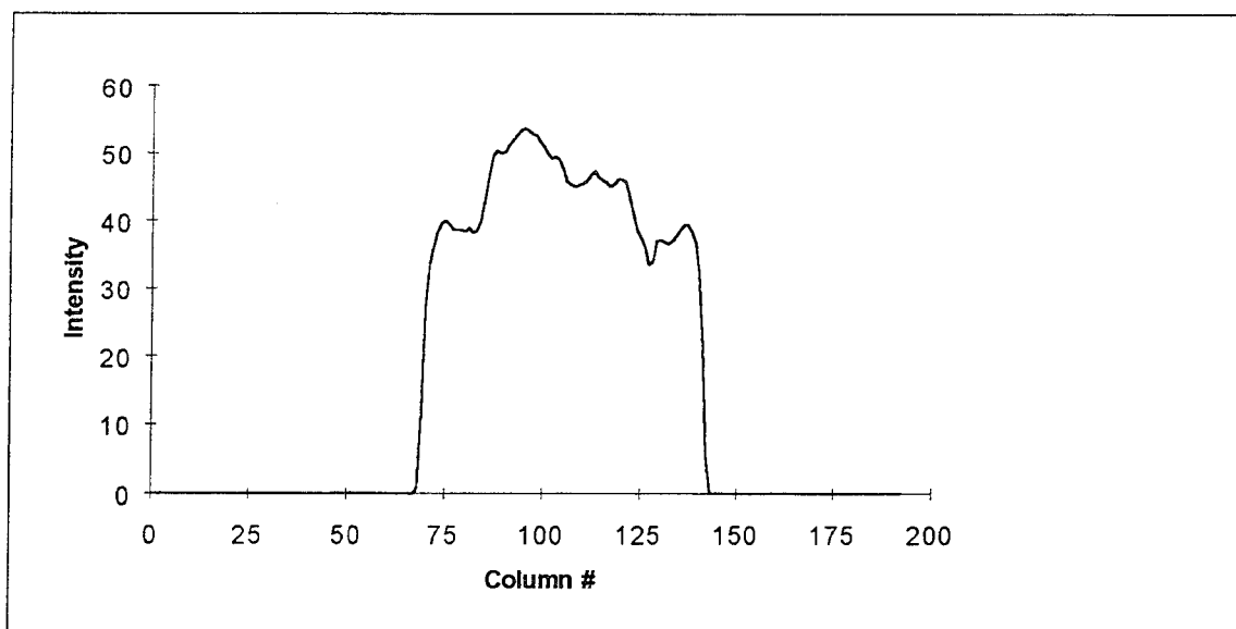
Fig. D-42. Complemented reflection of T4 squashed to preserve horizontal sequences
