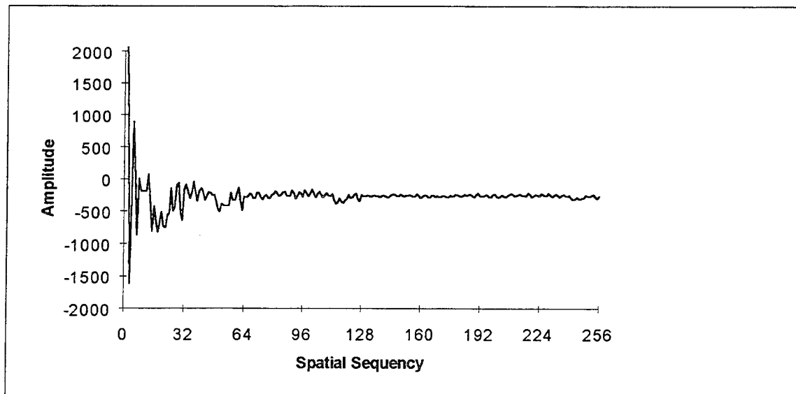
Fig. C-43. Walsh transform of Fig. C-42
