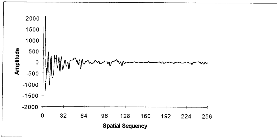
Fig. C-5. Walsh transform of Fig. C-4
