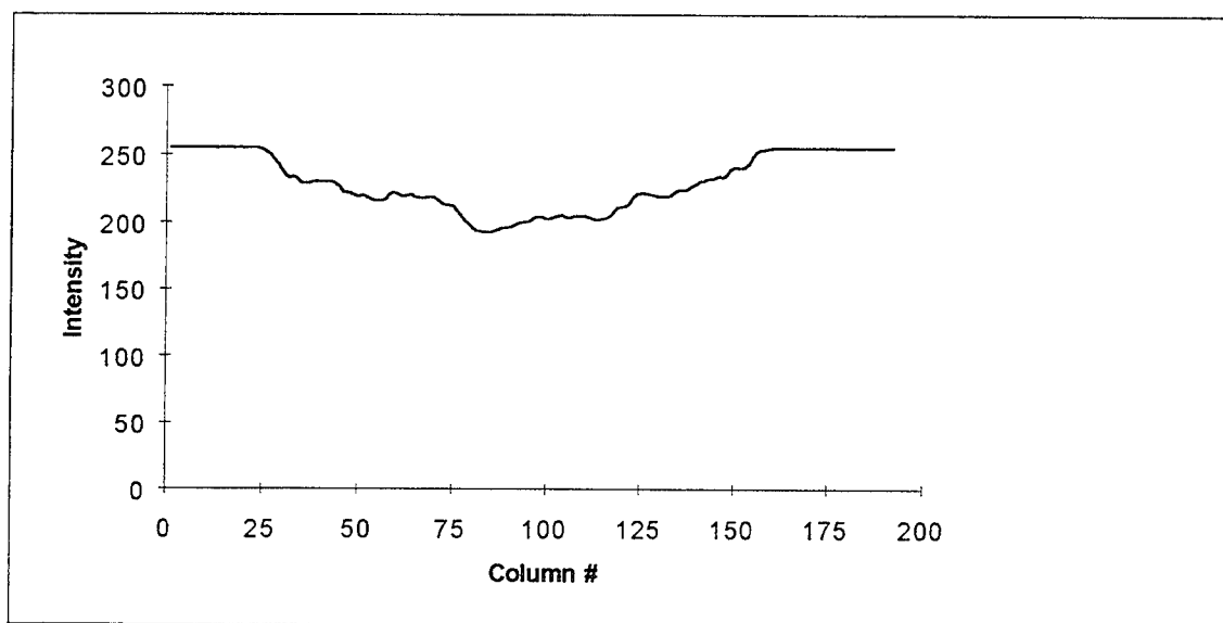
Fig. D-104. T8 squashed to preserve horizontal sequencies
