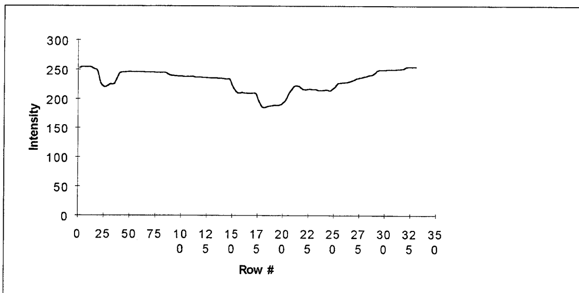
Fig. C-82. Reflection of H5 squashed to preserve vertical sequencies
