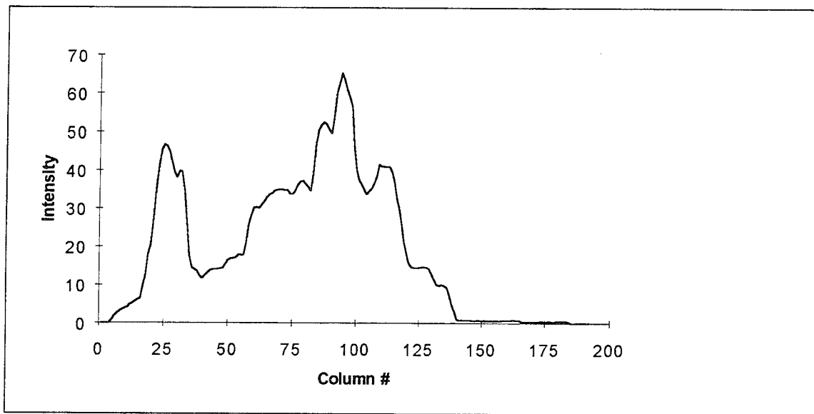
Fig. C-4. Complement of H1 squashed to preserve horizontal sequences
