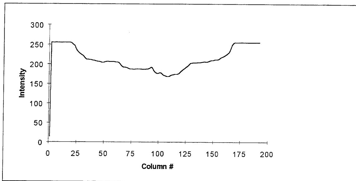
Fig. D-57. Reflection of T5 squashed to preserve horizontal sequences
