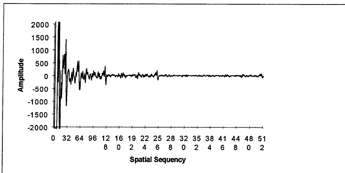
Fig. B-13. Walsh transform of Fig. B-12
