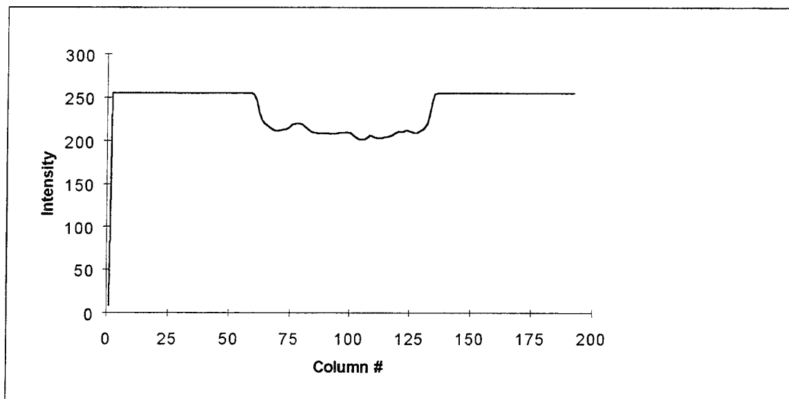
Fig. D-23. Reflection of T3 squashed to preserve horizontal sequencies
