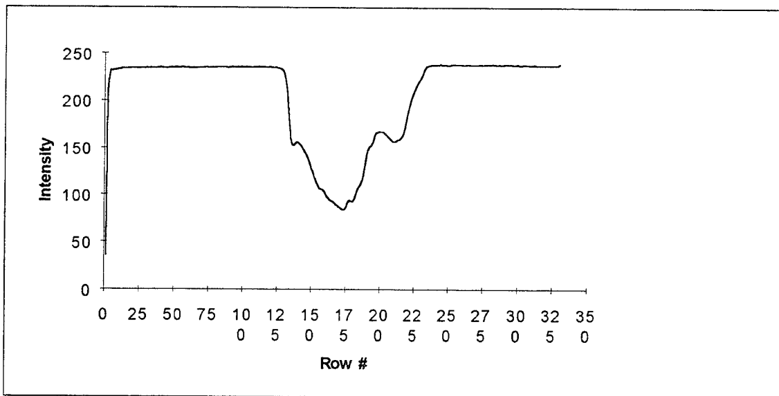
Fig. D-14. Reflection of T1 squashed to preserve vertical sequences
