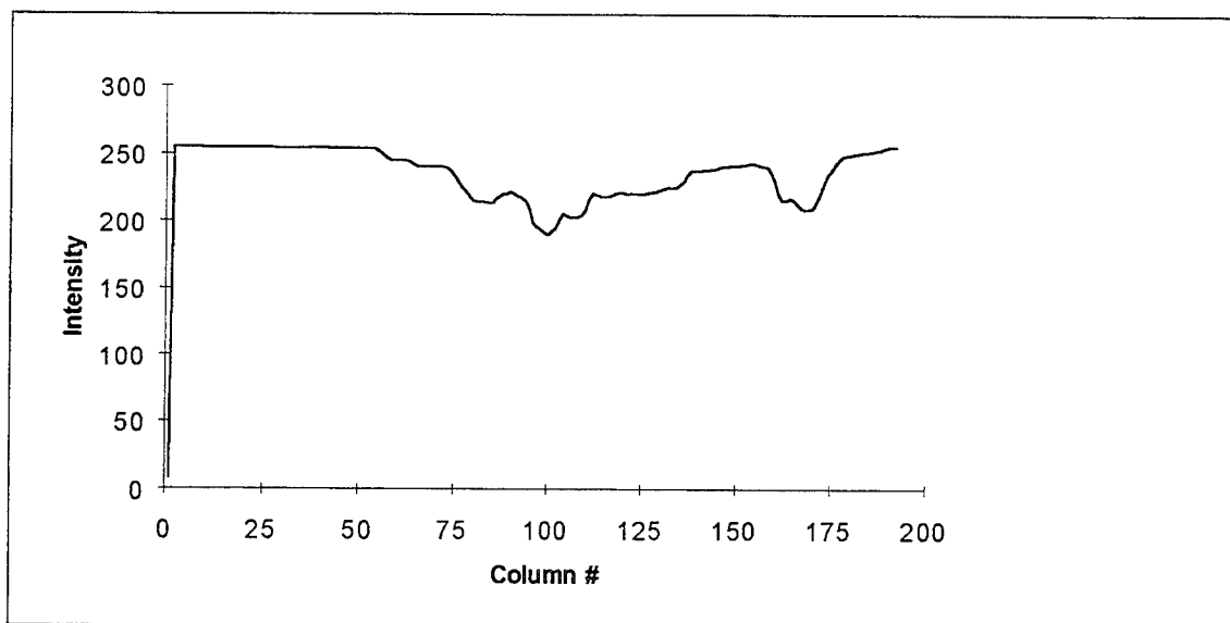
Fig. C-6. Reflection of H-1 squashed to preserve horizontal sequences
