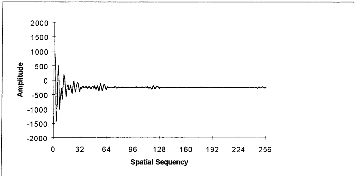
Fig. D-213. Walsh transform of Fig. D-212
