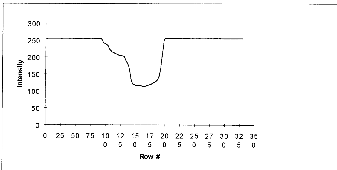
Fig. D-78. T6 squashed to preserve vertical sequences
