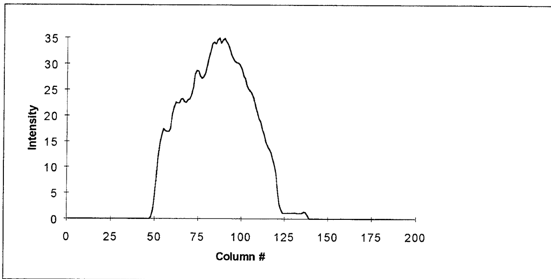
Fig. D-191. Complement of T14 squashed to preserve horizontal sequences
