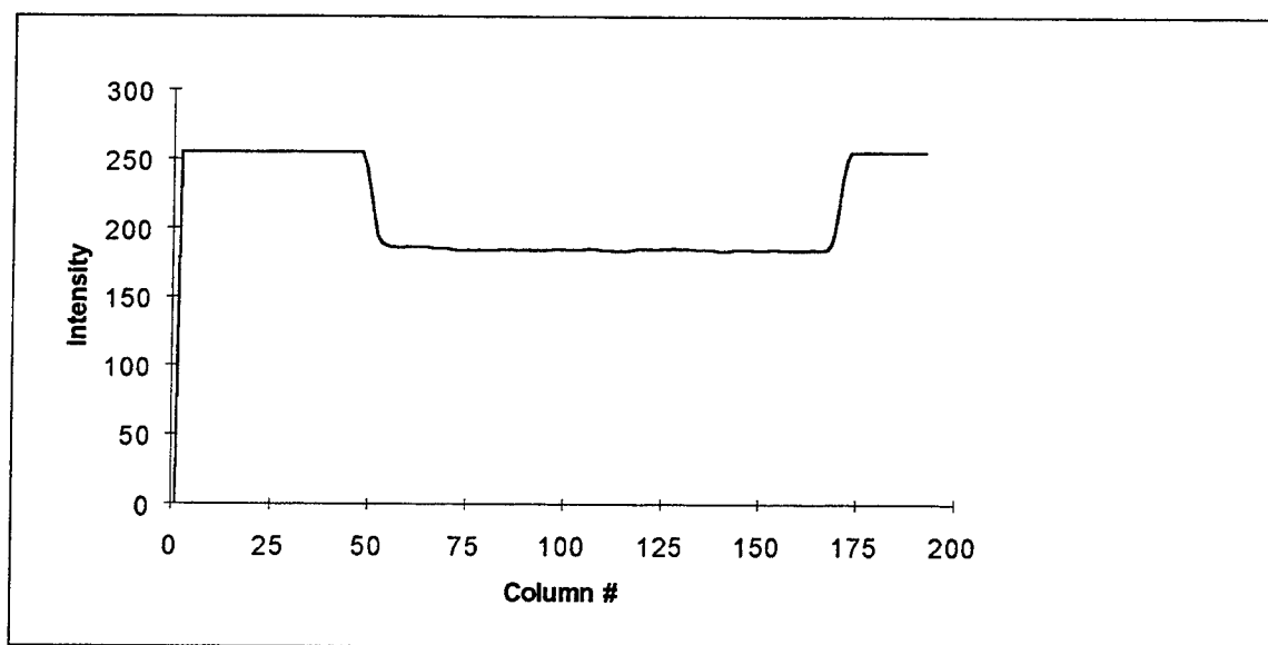
Fig. B-23. Reflection of A2 squashed to preserve horizontal sequences
