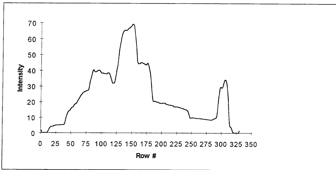
Fig. C-80. Complement of H5 squashed to preserve vertical sequences
