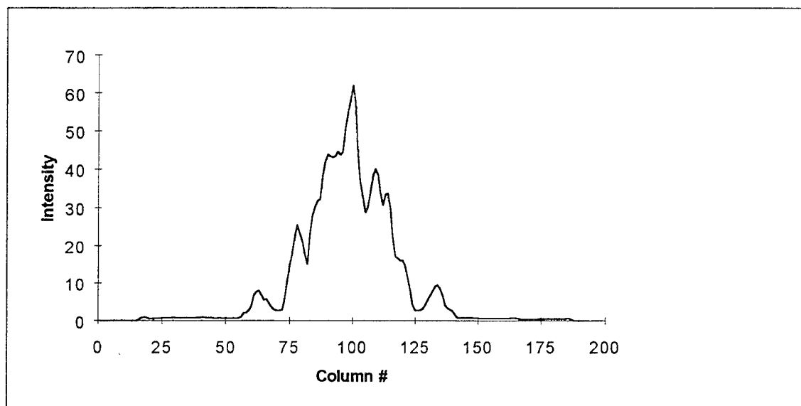
Fig. C-21. Complement of H2 squashed to preserve horizontal sequencies
