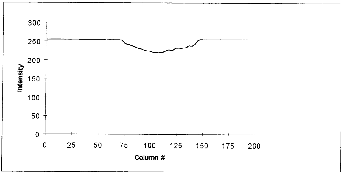
Fig. D-193. Reflection of T14 squashed to preserve horizontal sequences
