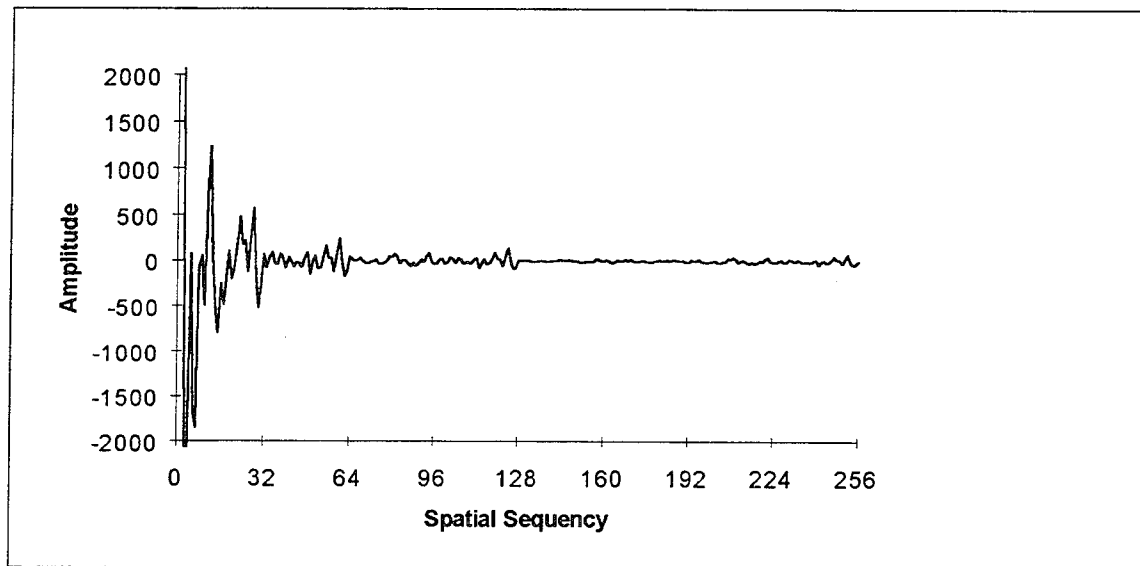
Fig. D-73. Walsh transform of Fig. D-72
