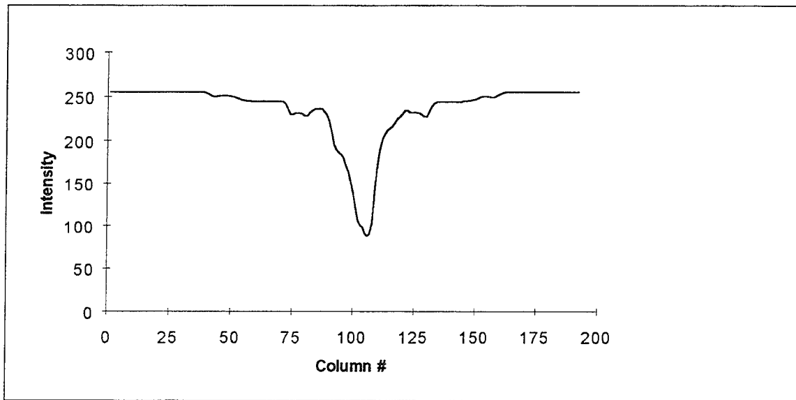
Fig. C-57. Reflection of H4 squashed to preserve horizontal sequences
