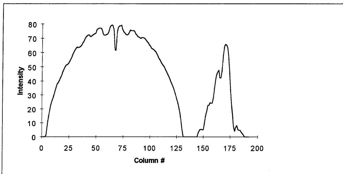
Fig. B-4. Complement of A1 squashed to preserve horizontal sequencies
