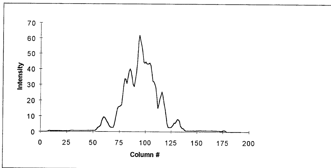
Fig. C-25. Complemented reflection of H2 squashed to preserve horizontal sequences
