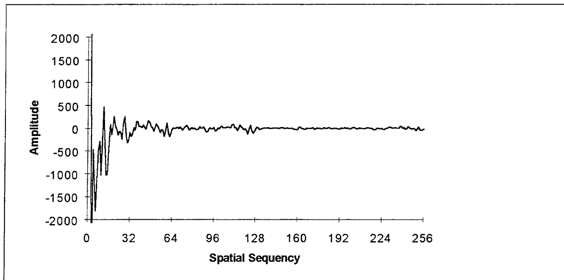
Fig. D-5. Walsh transform of Fig. D-4
