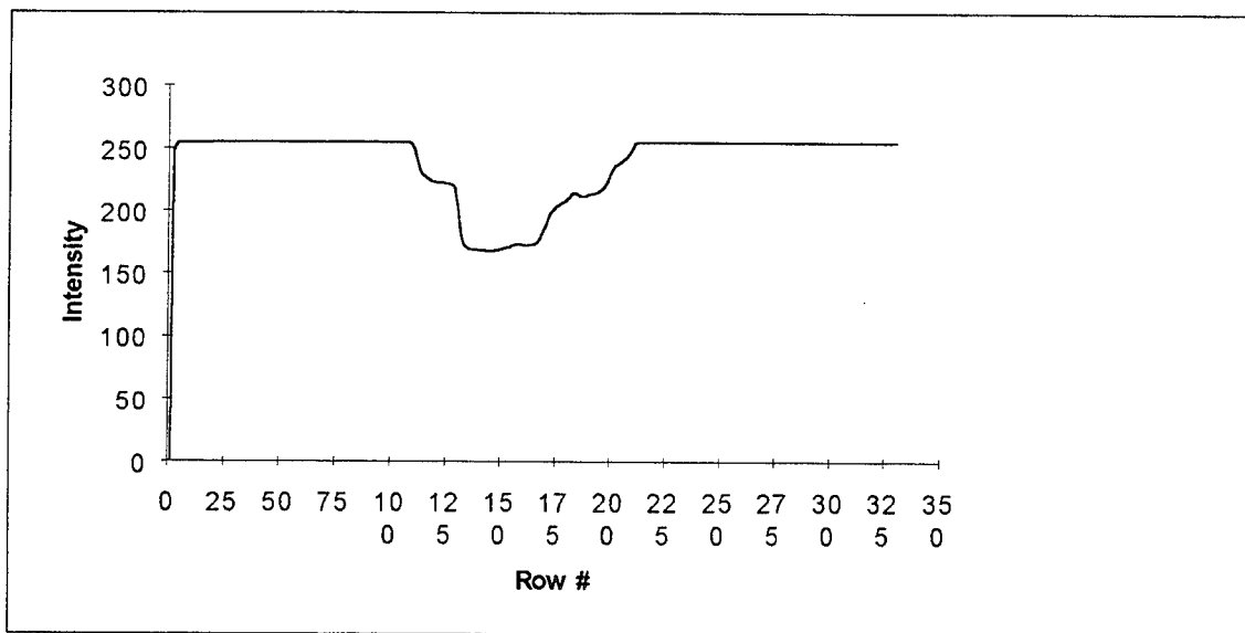
Fig. D-48. Reflection of T4 squashed to preserve vertical sequences
