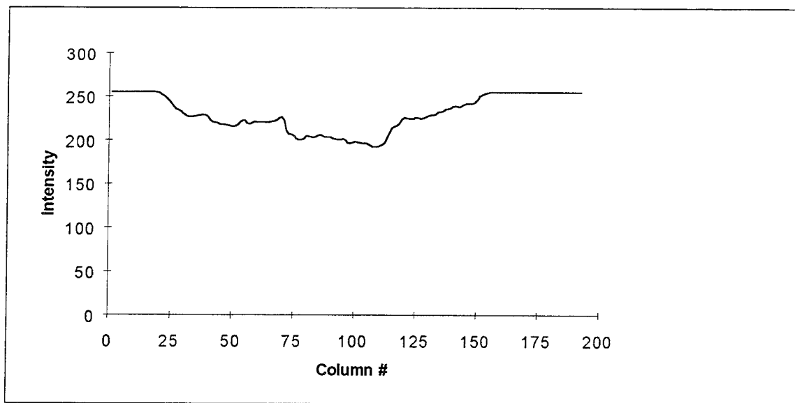
Fig. D-121. T9 squashed to preserve horizontal sequences
