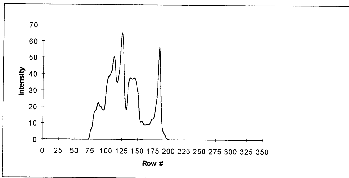
Fig. C-33. Complemented reflection of H2 squashed to preserve vertical sequences
