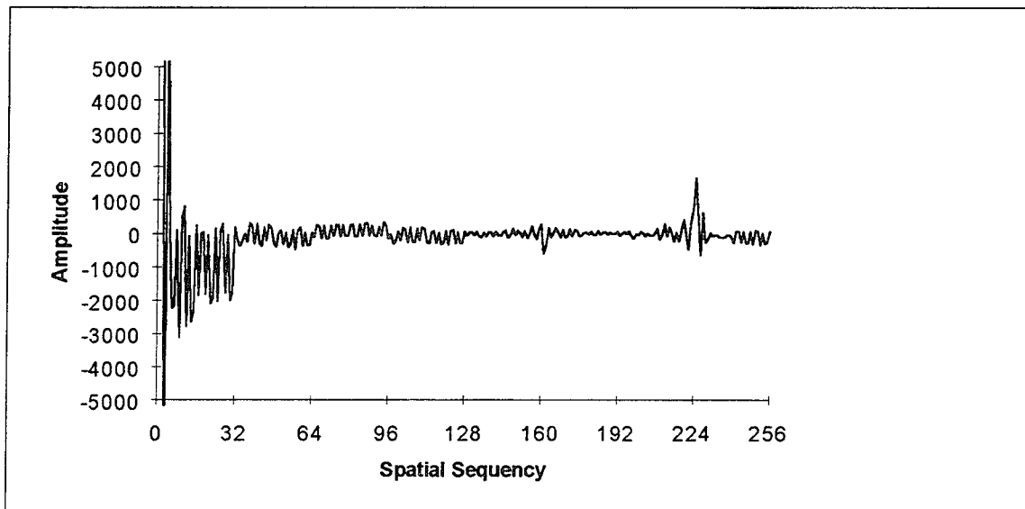
Fig. B-39. Walsh transform of Fig. B-38
