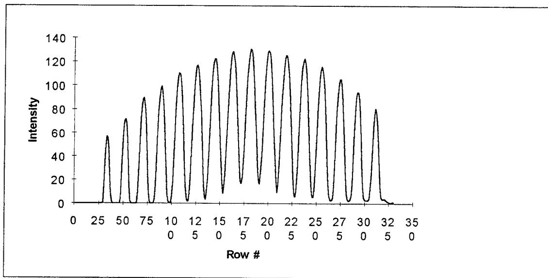
Fig. B-67 Complemented reflection of R2 squashed to preserve vertical sequences
