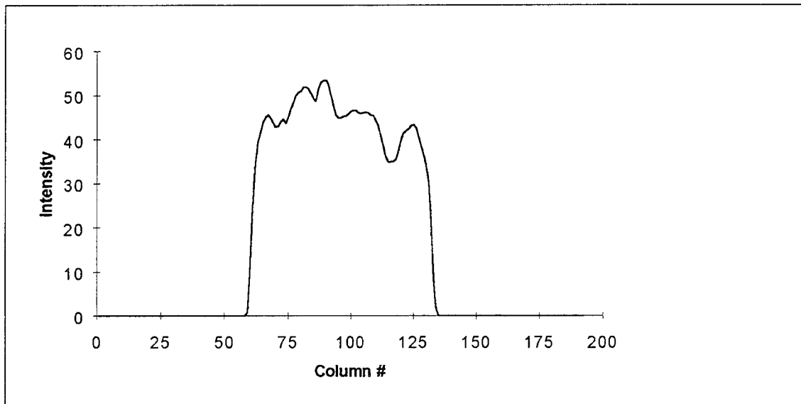
Fig. D-21. Complement of T3 squashed to preserve horizontal sequences
