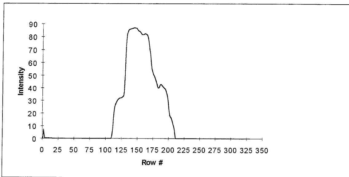
Fig. D-50. Complemented reflection of T4 squashed to preserve vertical sequences
