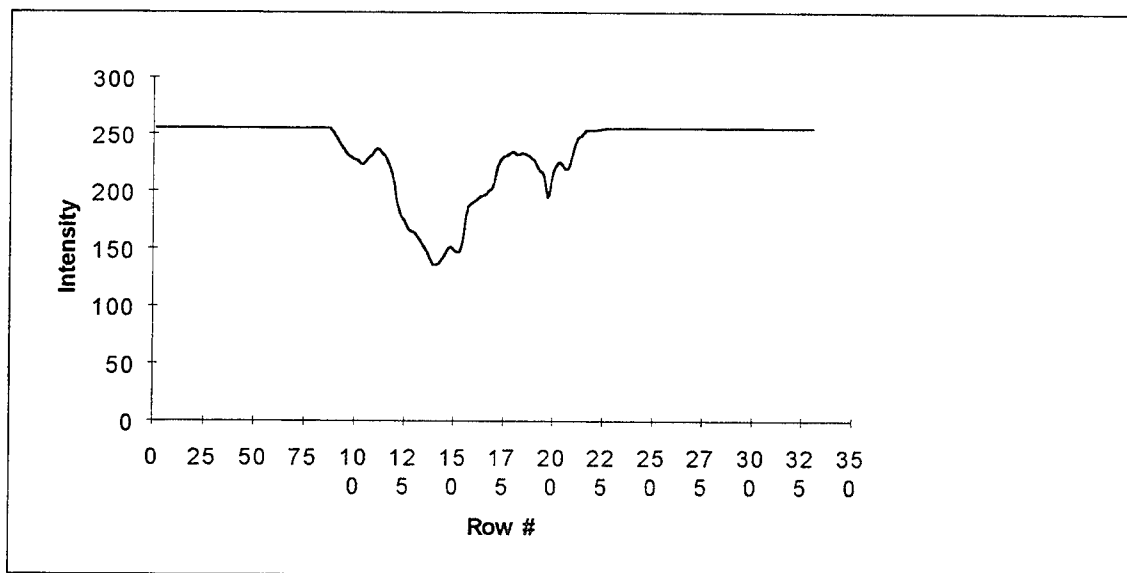
Fig. C-14. Reflection of H1 squashed to preserve vertical sequences
