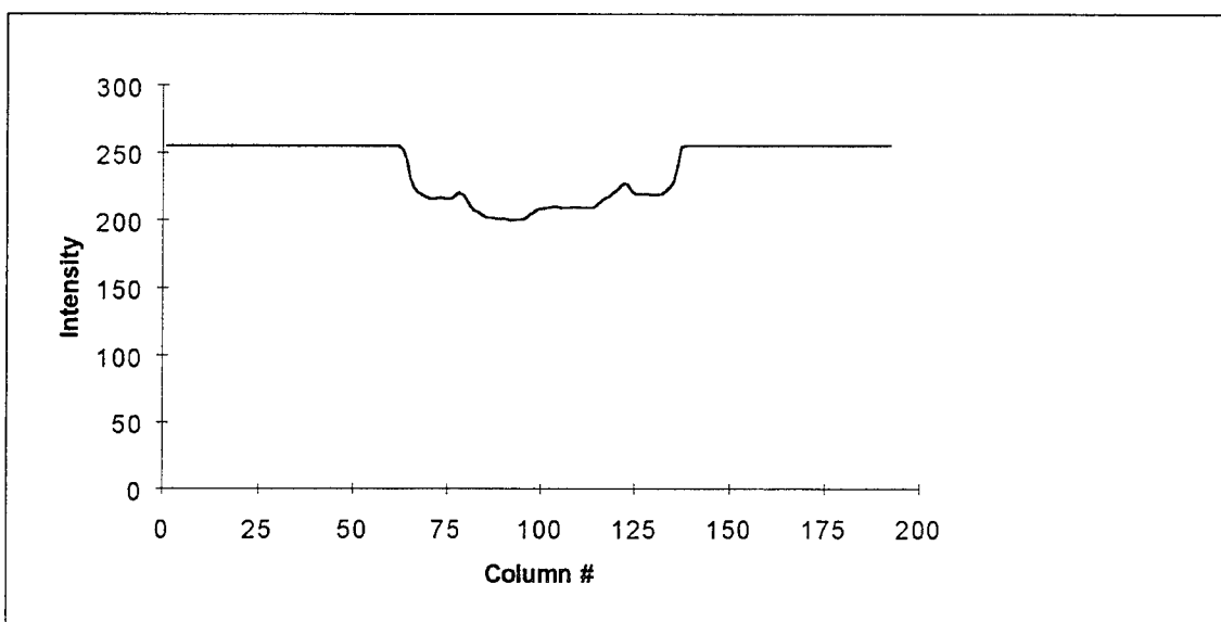
Fig. D-138. T10 squashed to preserve horizontal sequencies
