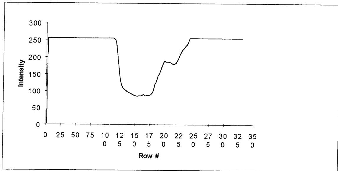
Fig. D-65. Reflection of T5 squashed to preserve vertical sequences
