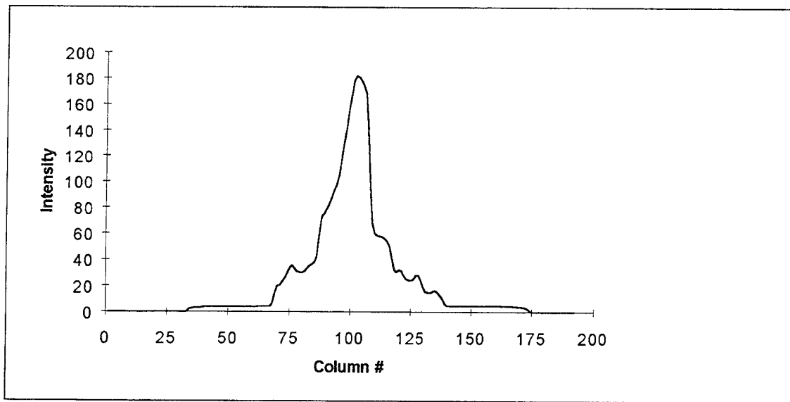
Fig. C-76. Complemented reflection of H5 squashed to preserve horizontal sequences
