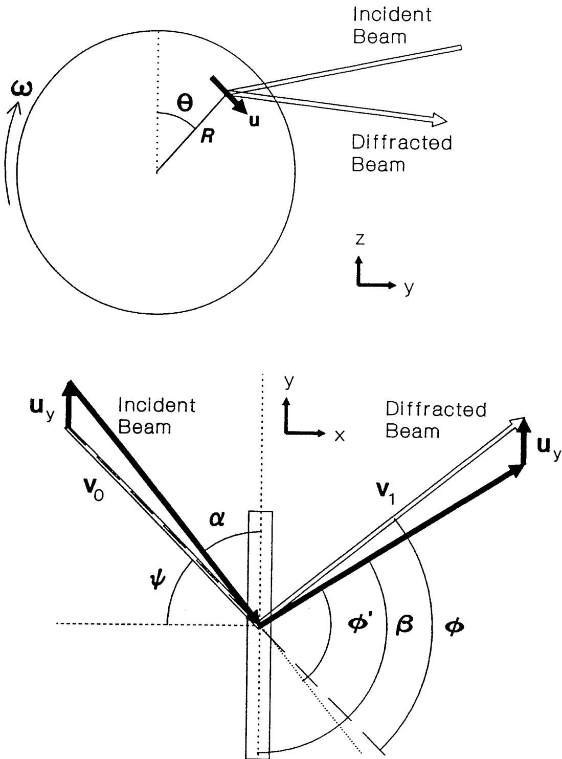
Fig. 3.10 Definition of coordinates and angles for a calculation of the Doppler effect in a spinning disc.
