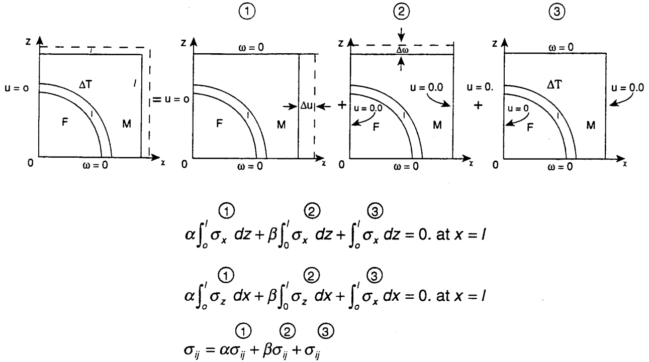
Figure 23. Micromechanical Model for Thermal Stress Analysis.
