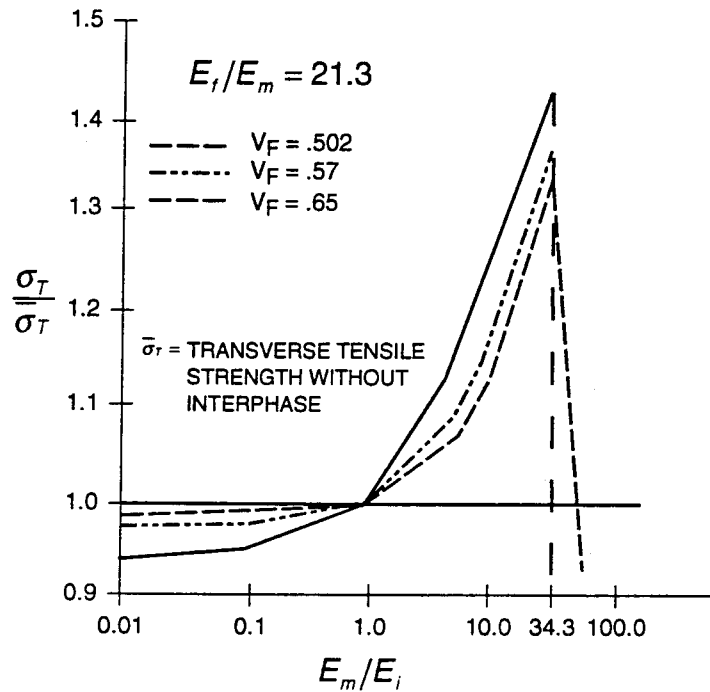
Figure 19. Effect of Interphase Moduli on the Transverse Tensile Strength of Composite Material.
