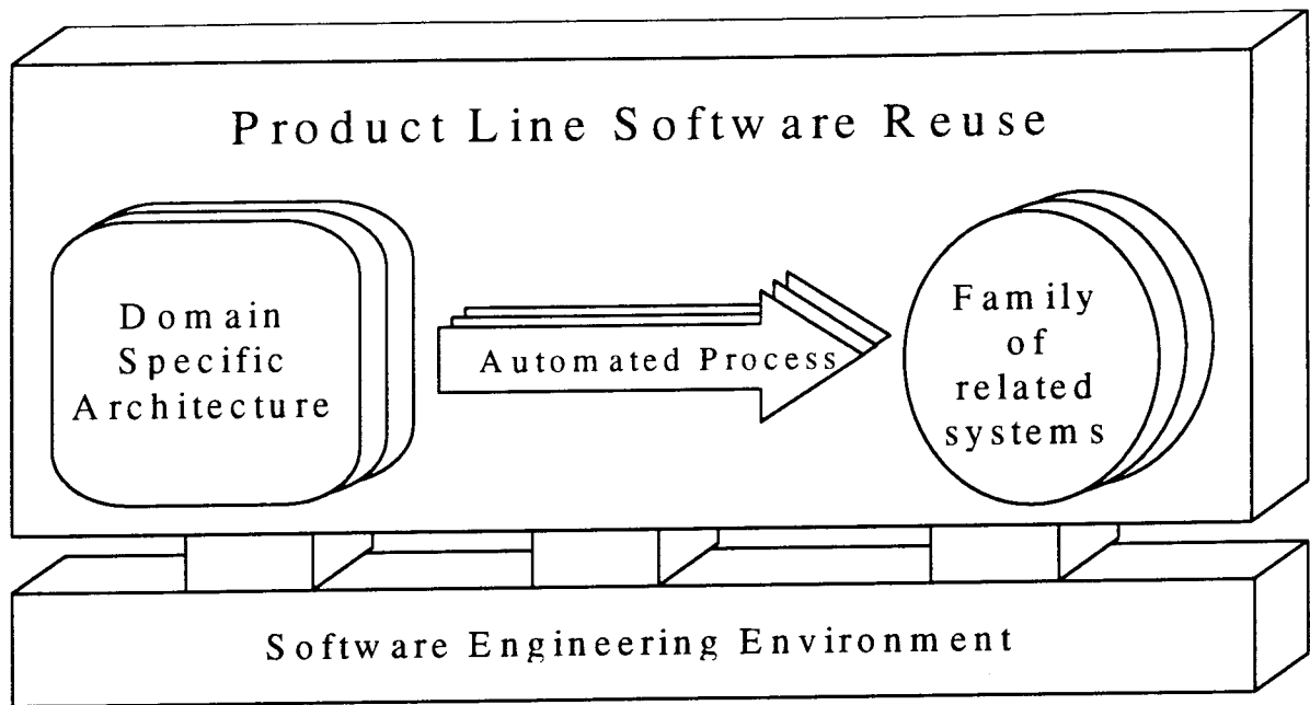
Figure 1. SCAI Megaprogramming
