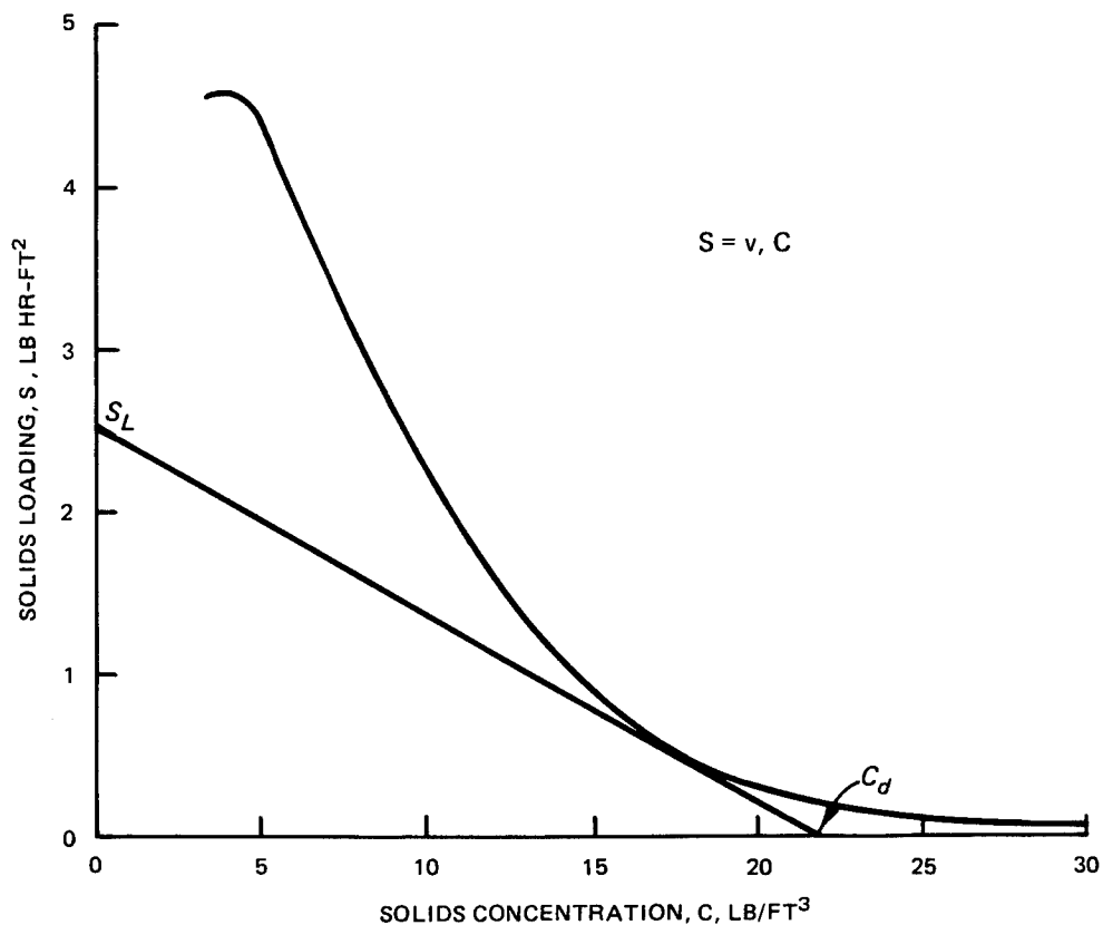
Figure 3. Typical solids loading curve for dredged material
