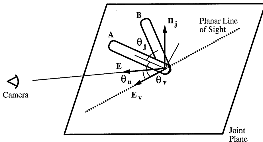
Figure 5: Occlusion properties of two links connected by a revolute joint.
