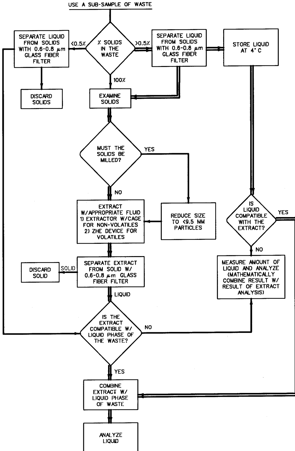
Figure 4. TCLP flowchart
