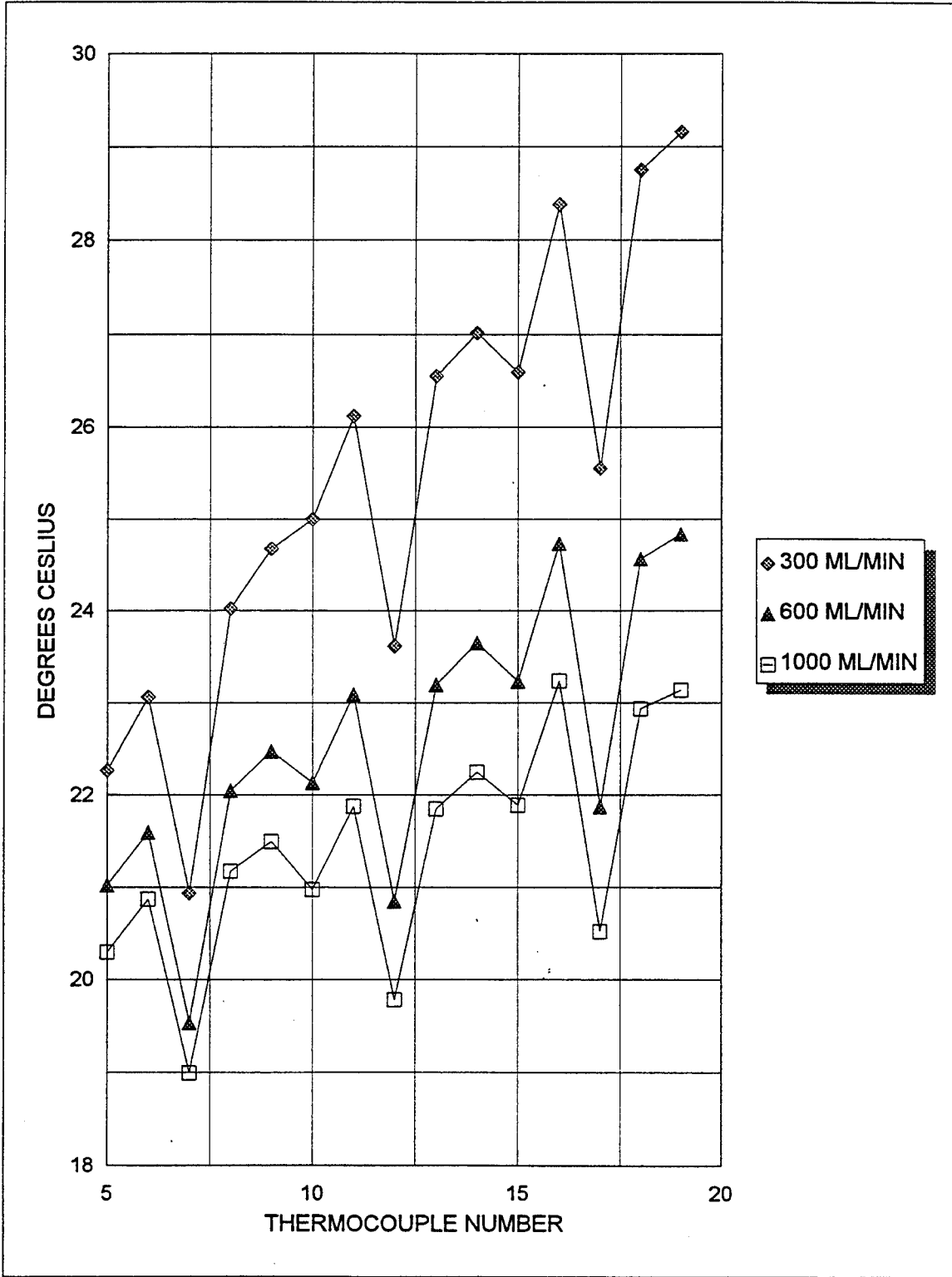
Figure 15. Module surface temperatures at power setting 9.
