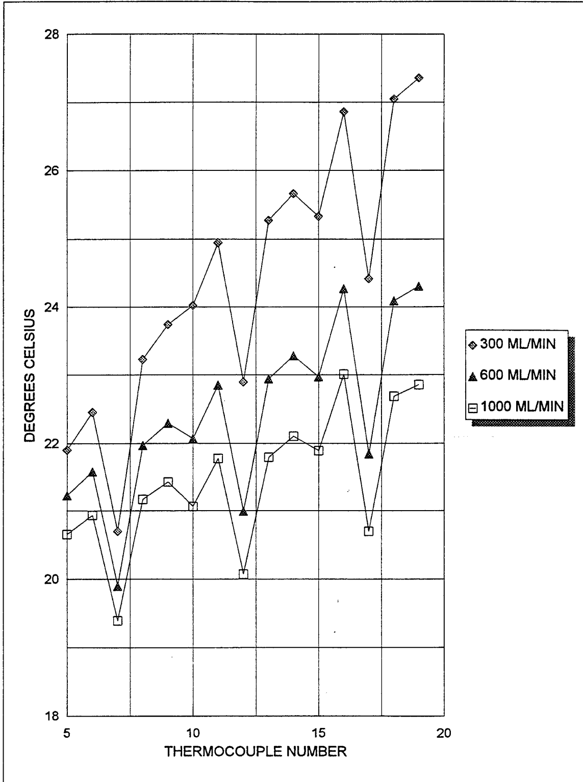
Figure 13. Module surface temperatures at power setting 7.
