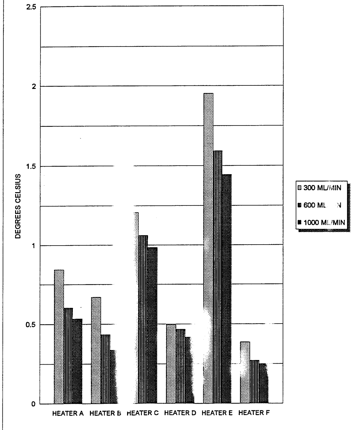
Figure 30. Temp rise across heaters at power setting 10.
