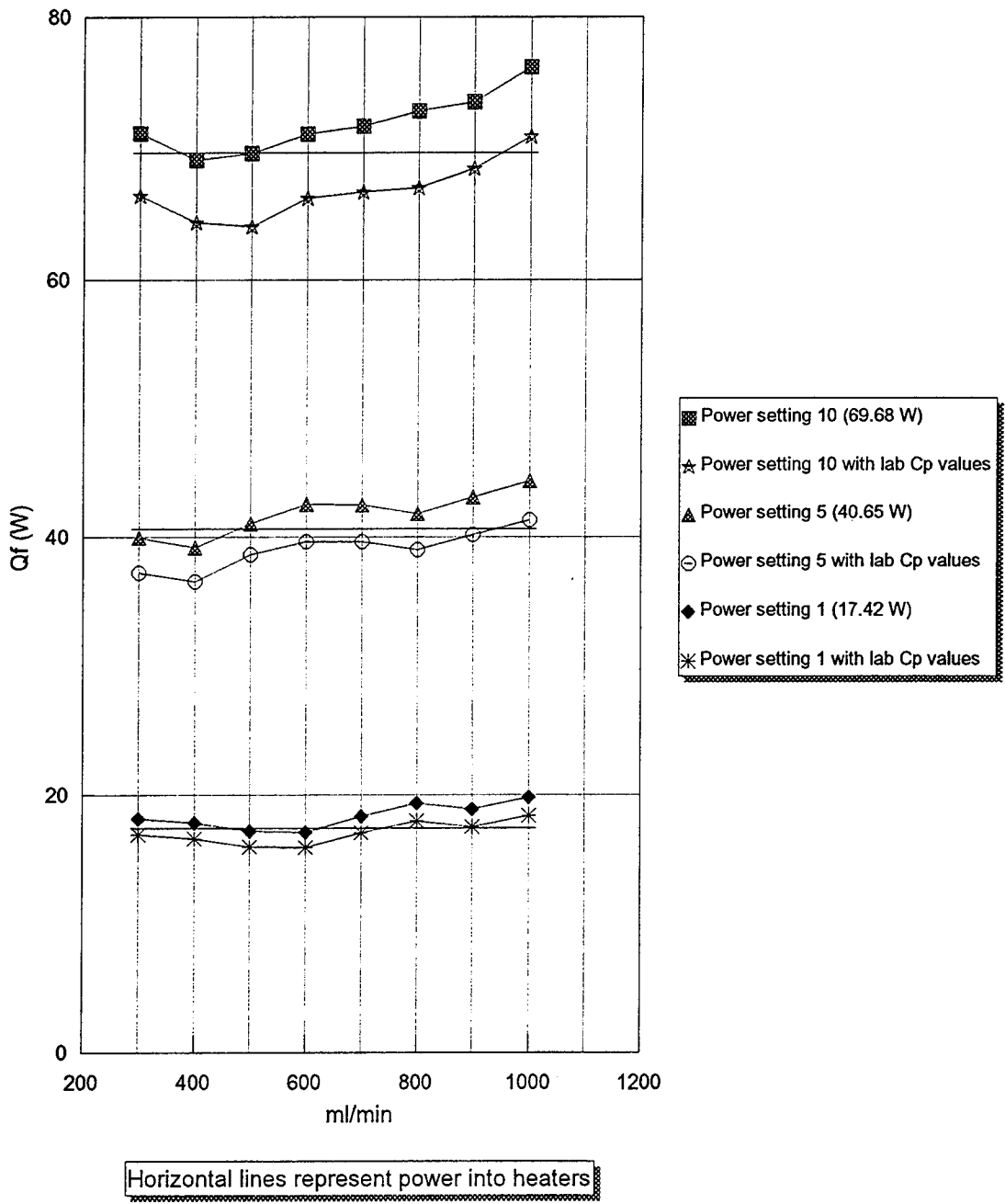
Figure 20. Revised Q_f calculations based on lab data.
