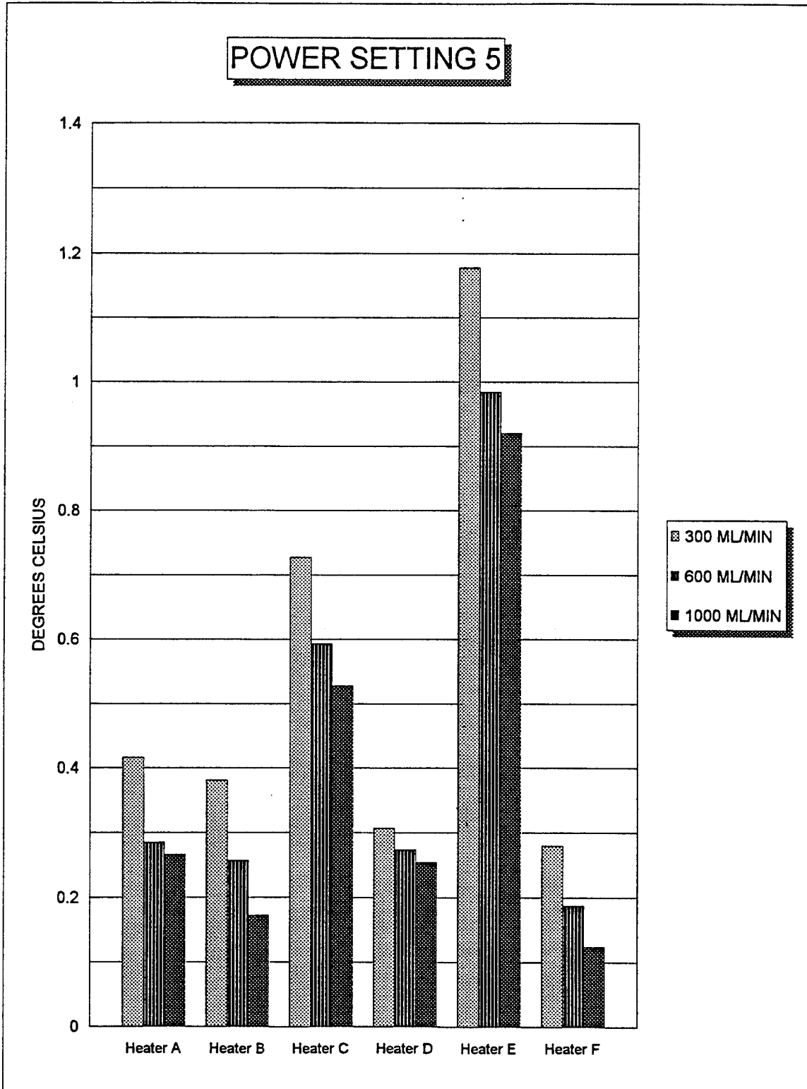
Figure 25. Temp rise across heaters at power setting 5.
