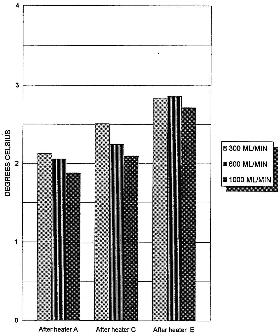
Figure 39. Mid-channel temp drops at power setting 9.
