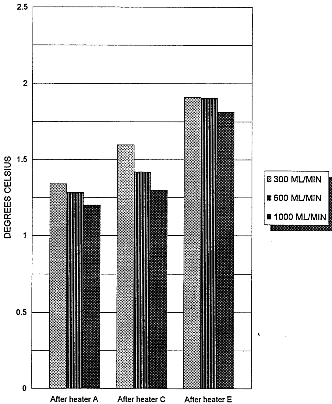
Figure 35. Mid-channel temp drops at power setting 5.
