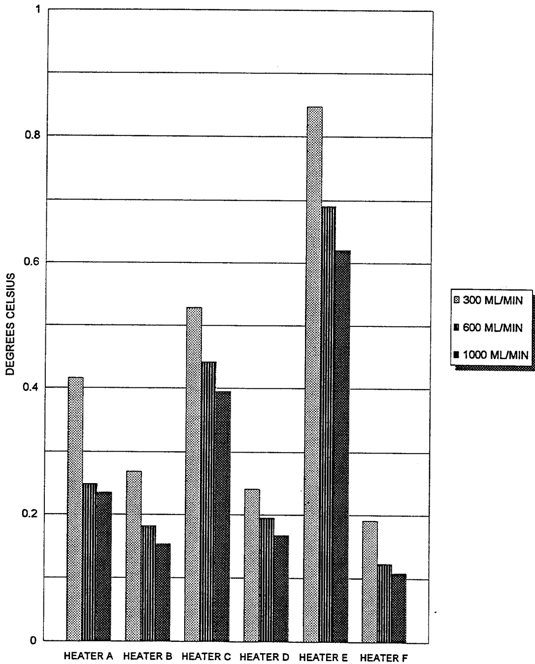
Figure 23. Temp rise across heaters at power setting 3.
