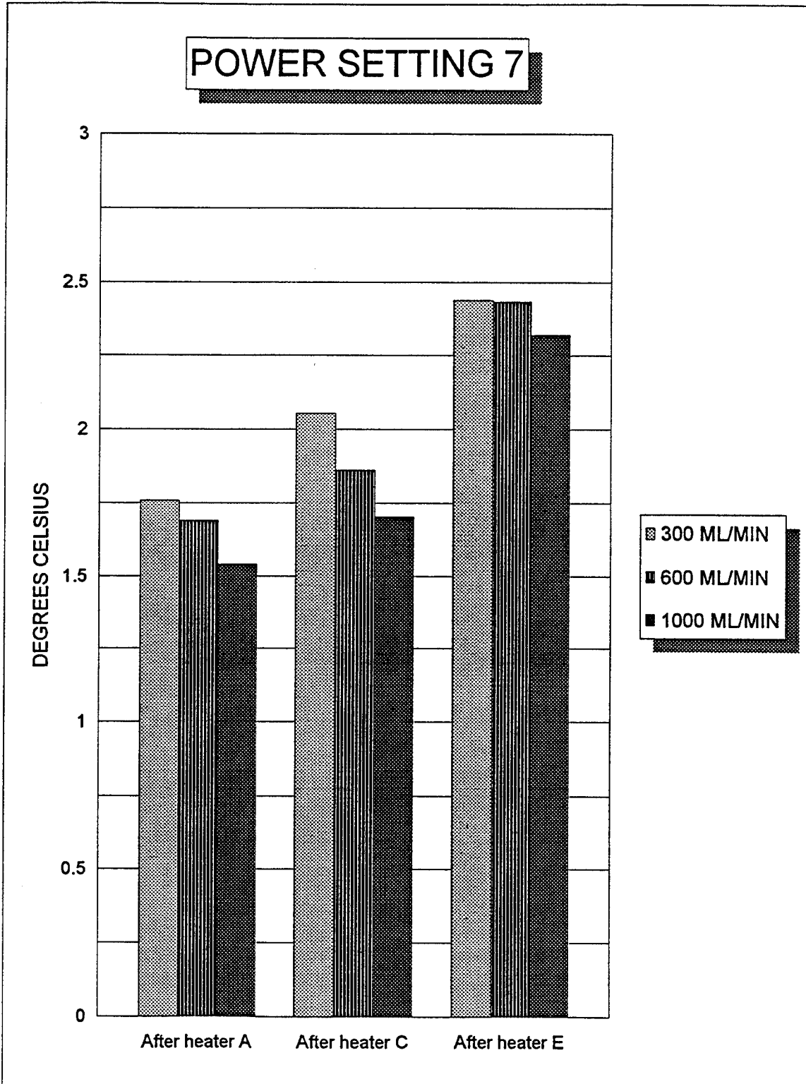
Figure 37. Mid-channel temp drops at power setting 7.
