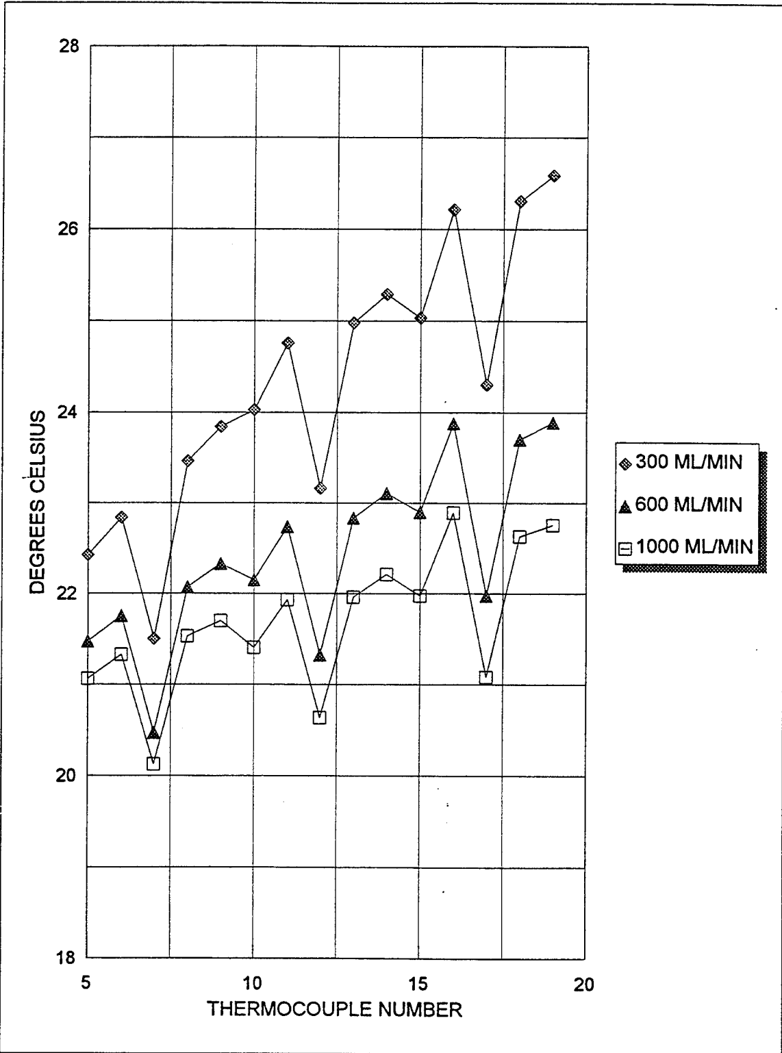
Figure 11. Module surface temperatures at power setting 5.
