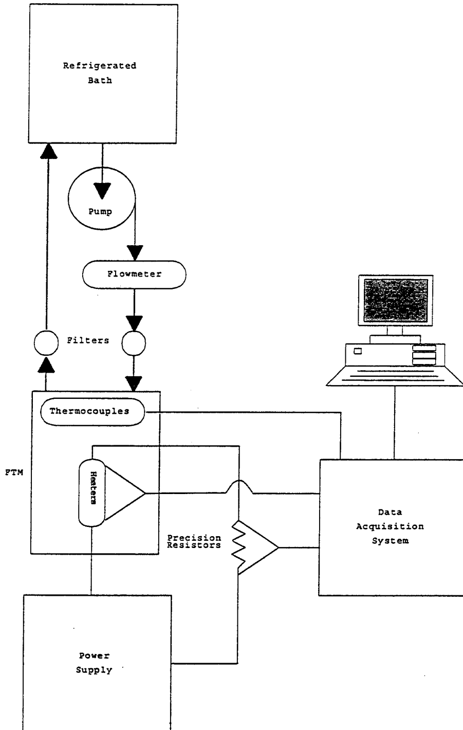
Figure 4. Diagram of experimental setup.
