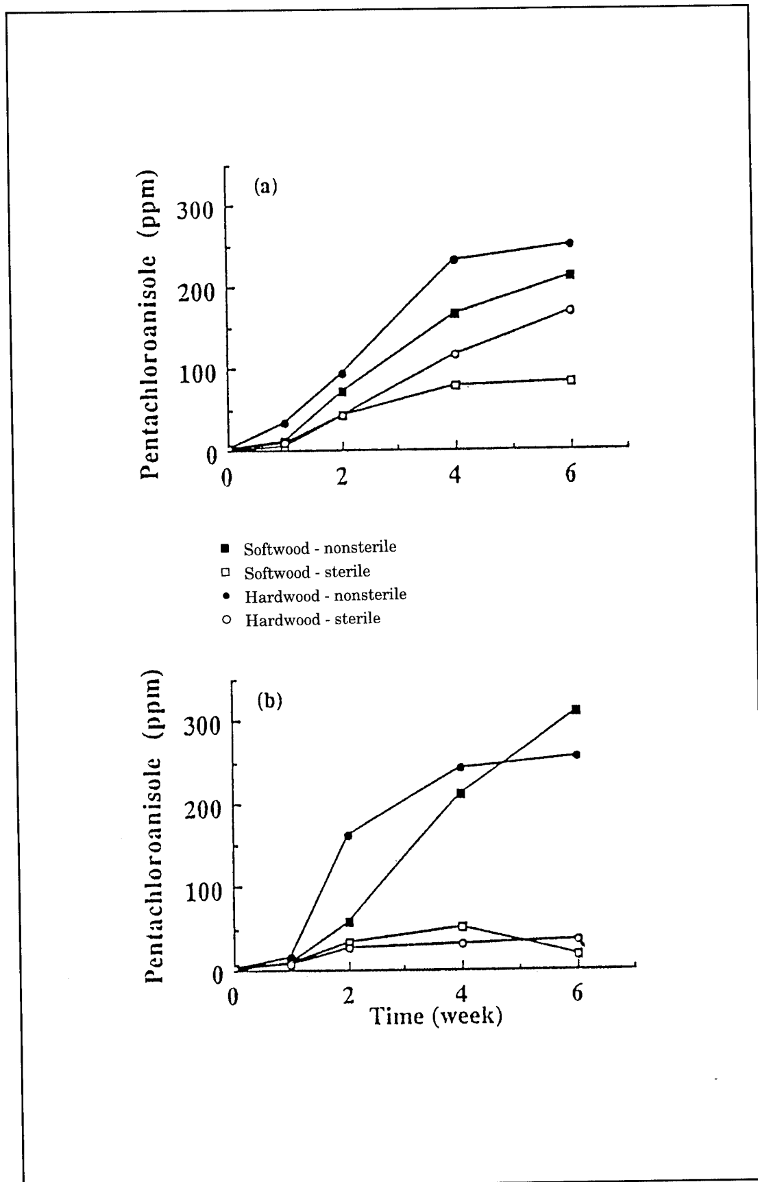
Figure 2. Accumulation of PCA in sterile and nonsterile hardwood and softwood chips inoculated with P. chrysosporium (a) or P. sordida (b).
