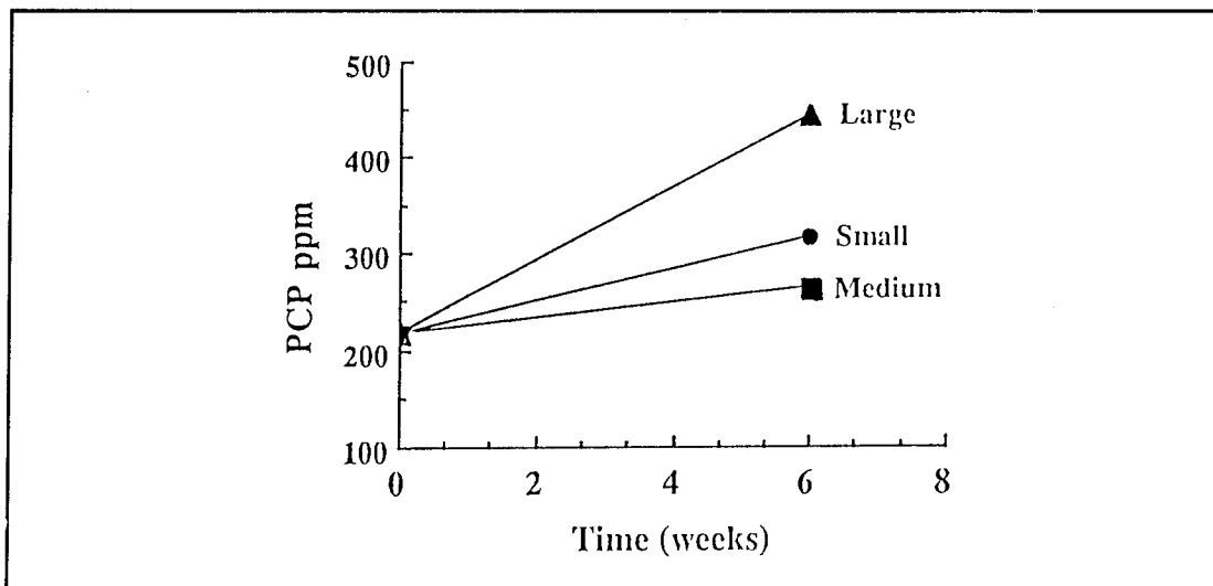
Figure 7. Initial and final concentrations of PCP in large, medium, and small control chips.
