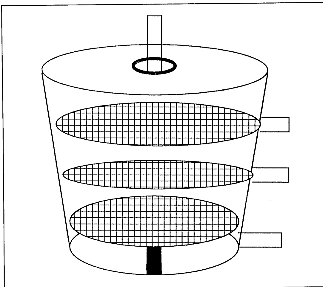
Figure 17. 8-Liter bioreactor.
