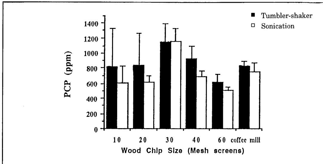
Figure 12. Effect of varying sizes of wood chips and sonication versus tumbler-shaker rotation on the extractability of PCP from wood.
