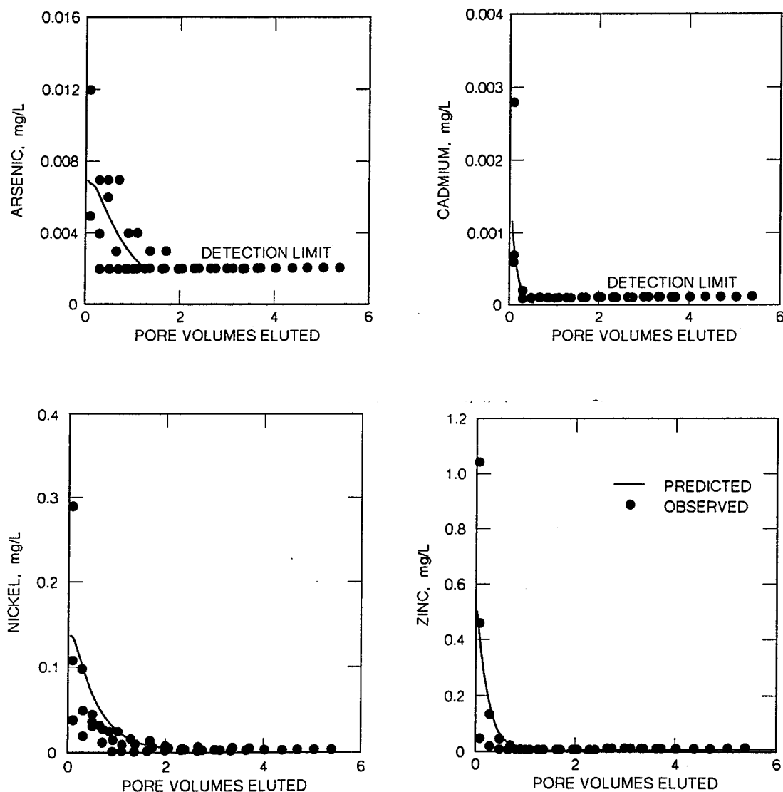
Figure 4. Predicted and observed column elution curves for Hamlet City Lake sediment
