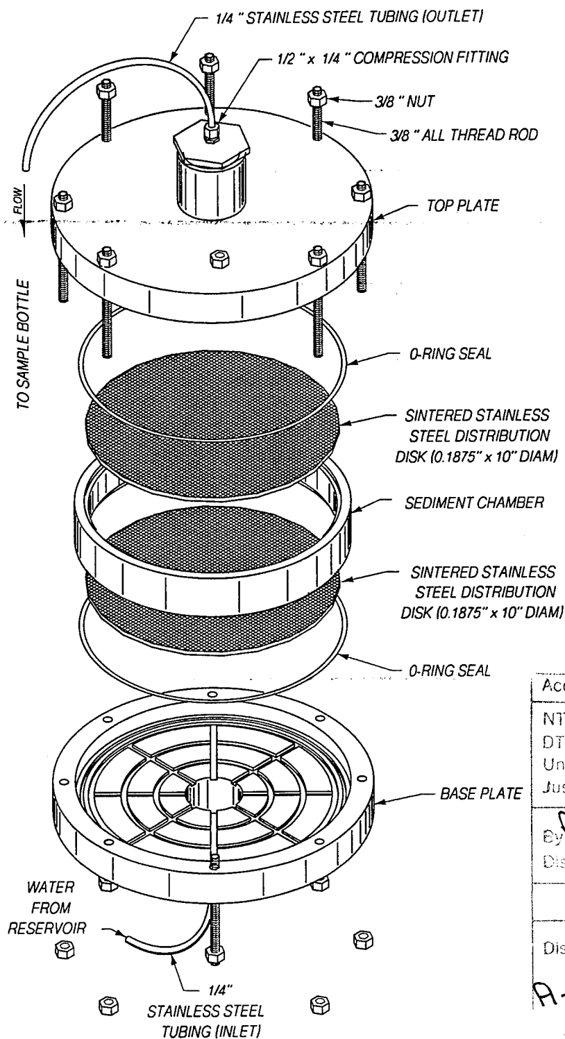
Figure 2. Schematic of column leaching apparatus for sediments
