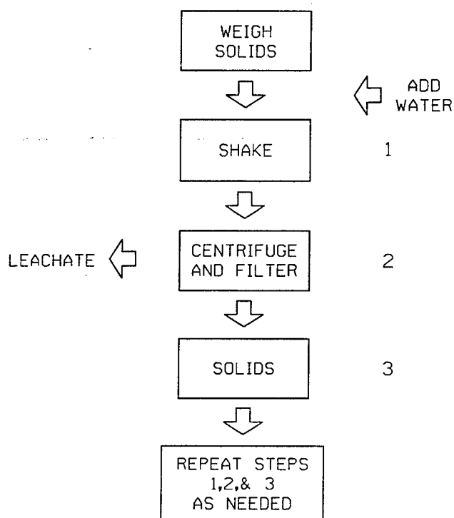
Figure 1. Schematic of WES sequential batch leach test
