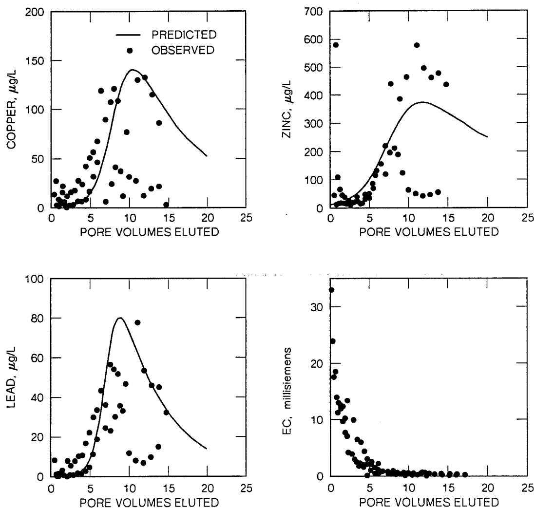
Figure 5. Predicted and observed elution curves for sediment from the West Richmond reach of J. F. Baldwin channel
