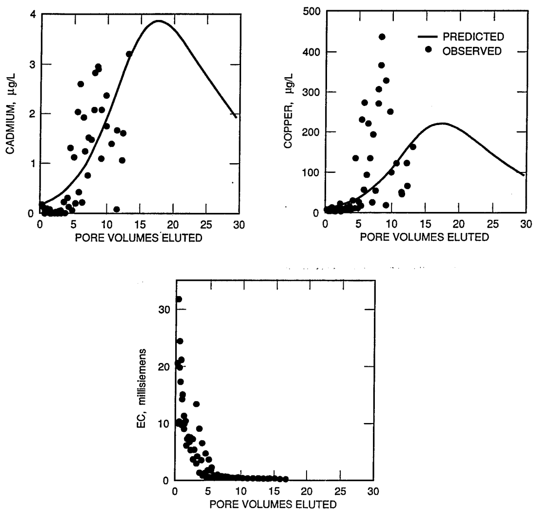
Figure 6. Predicted and observed elution curves for Richmond Harbor sediment, Santa Fe channel
