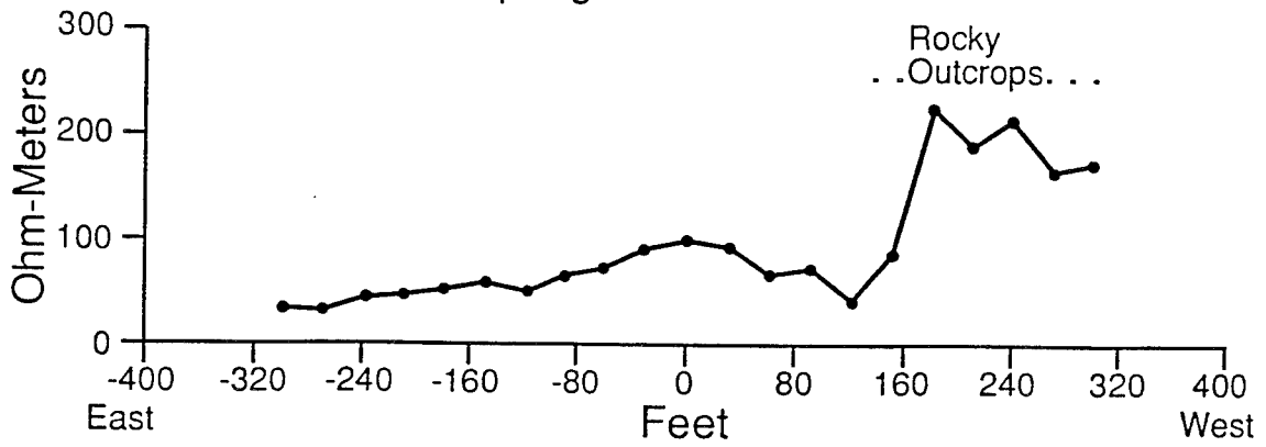
Cole Spring — Electrical Resistivity Profiles.
