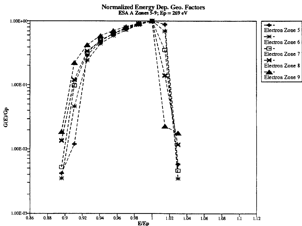
Figure 19. Normalized Electron Energy Dependent Geometric Factors Plotted vs. Normalized Energy for ESA A Zones 1-4 and 5-9 for the Channel With a Peak Response at 269 eV a) Zones 1-4; b) Zones 5-9
