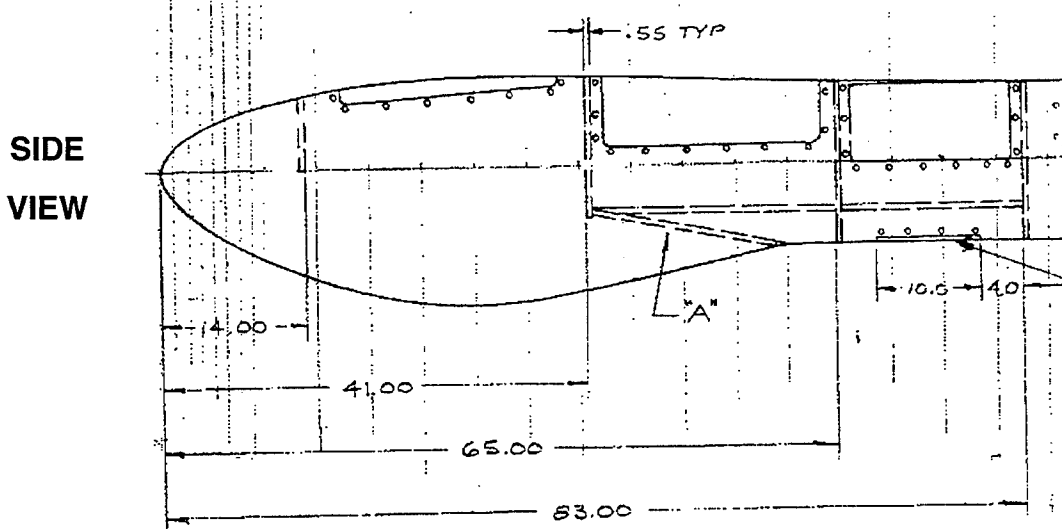
Figure D.2. UAV Drawings
