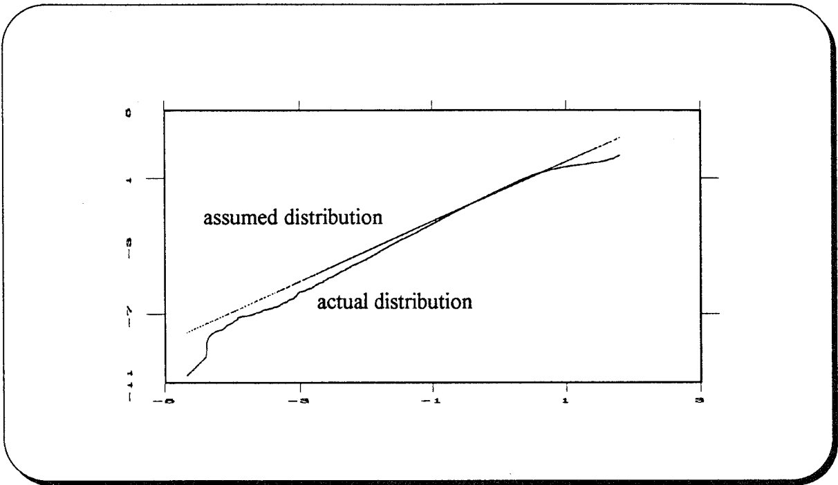
Figure 12. Plot of Fit to Weibull Distribution for Dunes Data. Perfect fit is plotted as a straight line on this plot.
