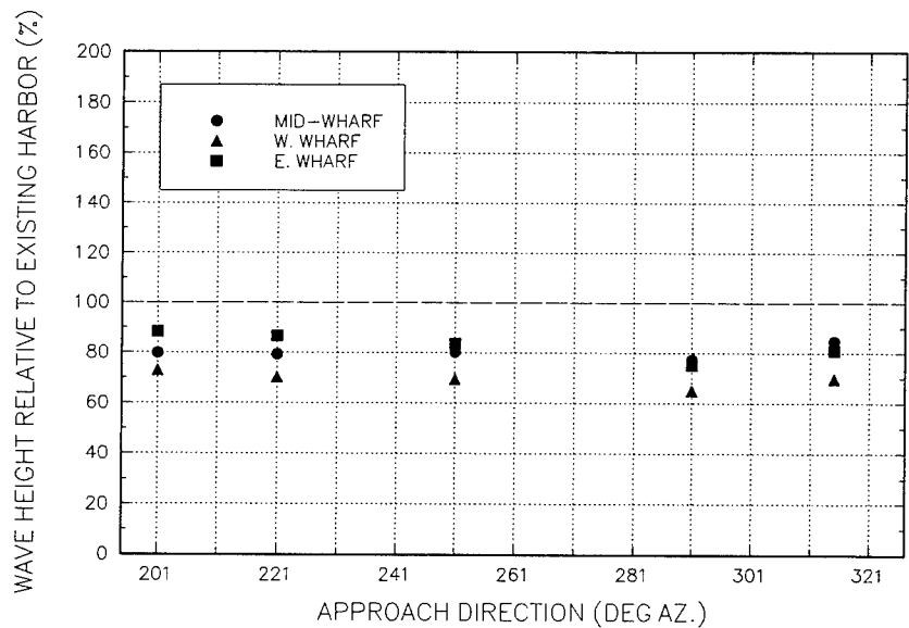
Figure 2. Evaluation of dogleg breakwater extension, T_p = 16 sec, Kaunalapau Harbor
