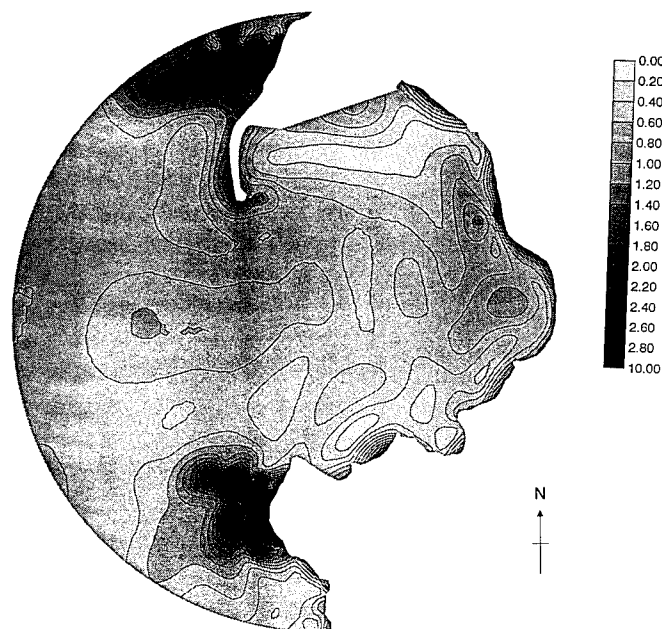
Figure 3. Amplification factor contours for existing Kaunalapau Harbor
