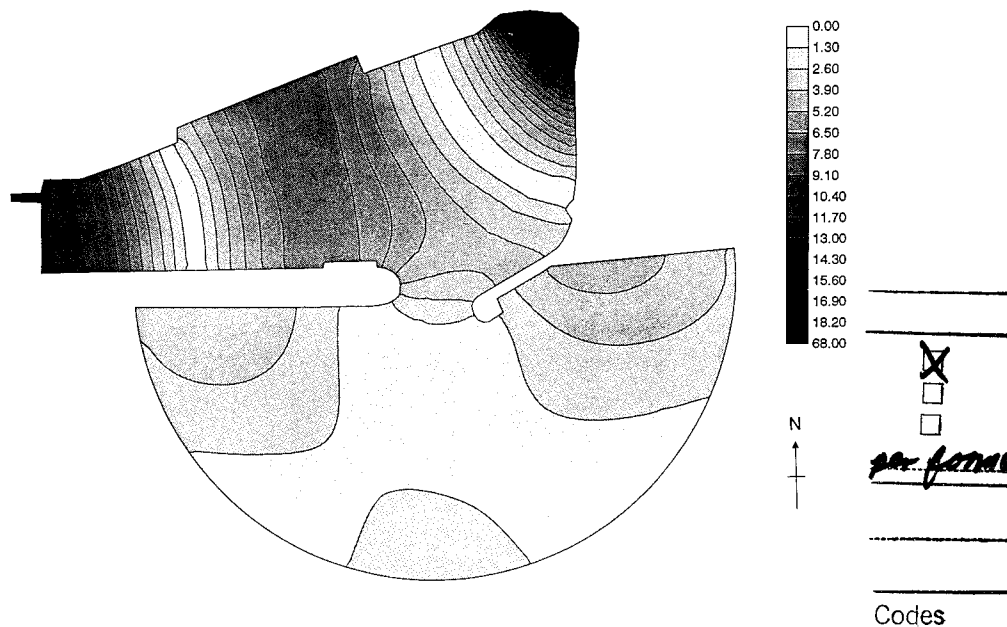
Figure 5. Amplification factor contours for resonant peak at 89.0-sec period (noted in Figure 5)
