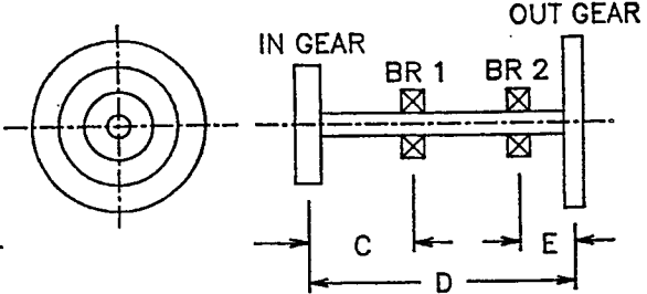
INPUT GEAR OVERHUNG
