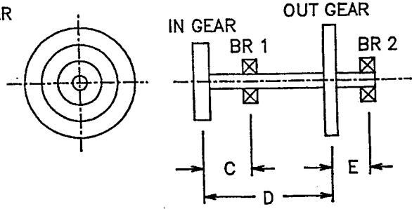
FIGURE 5 - INTERMEDIATE SHAFT BEARING CONFIGURATIONS
