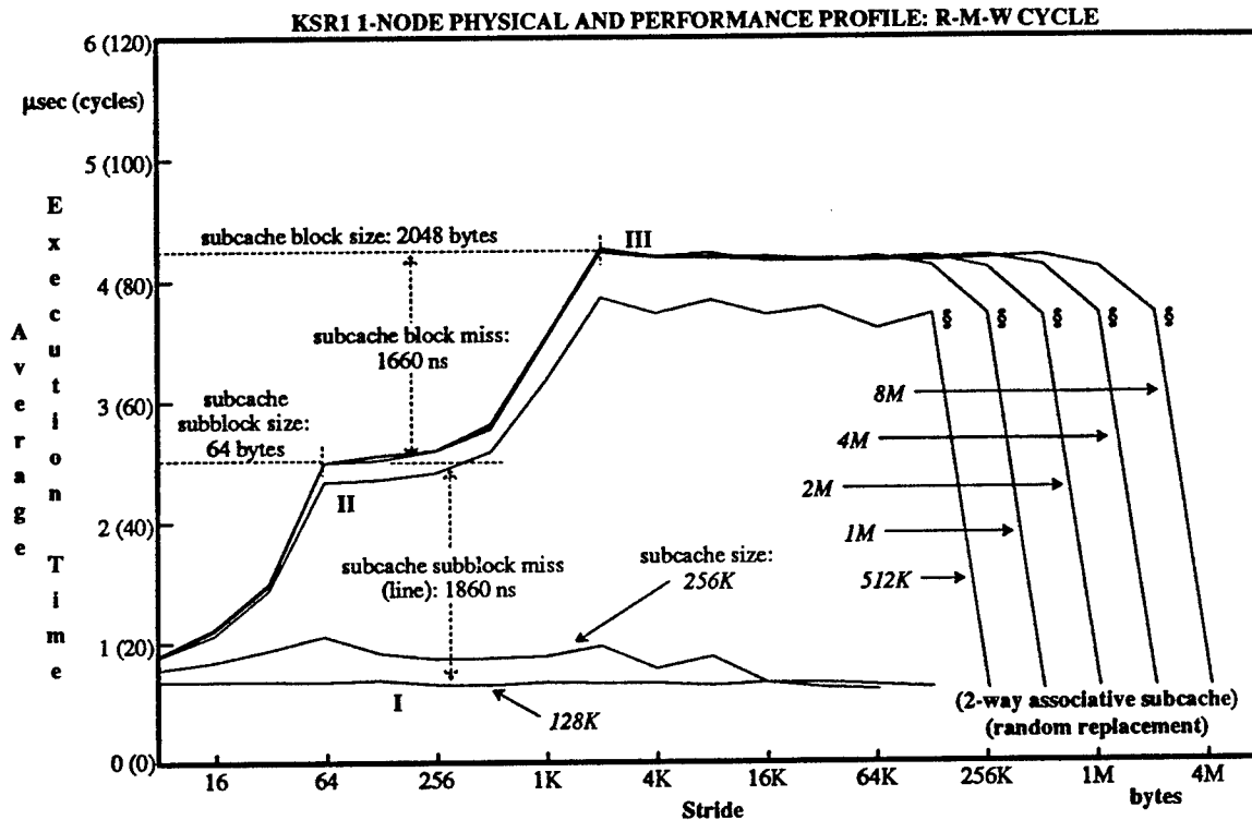
Figure 2: KSR1 single node Read-Modify-Write cycle physical and performance profile.
