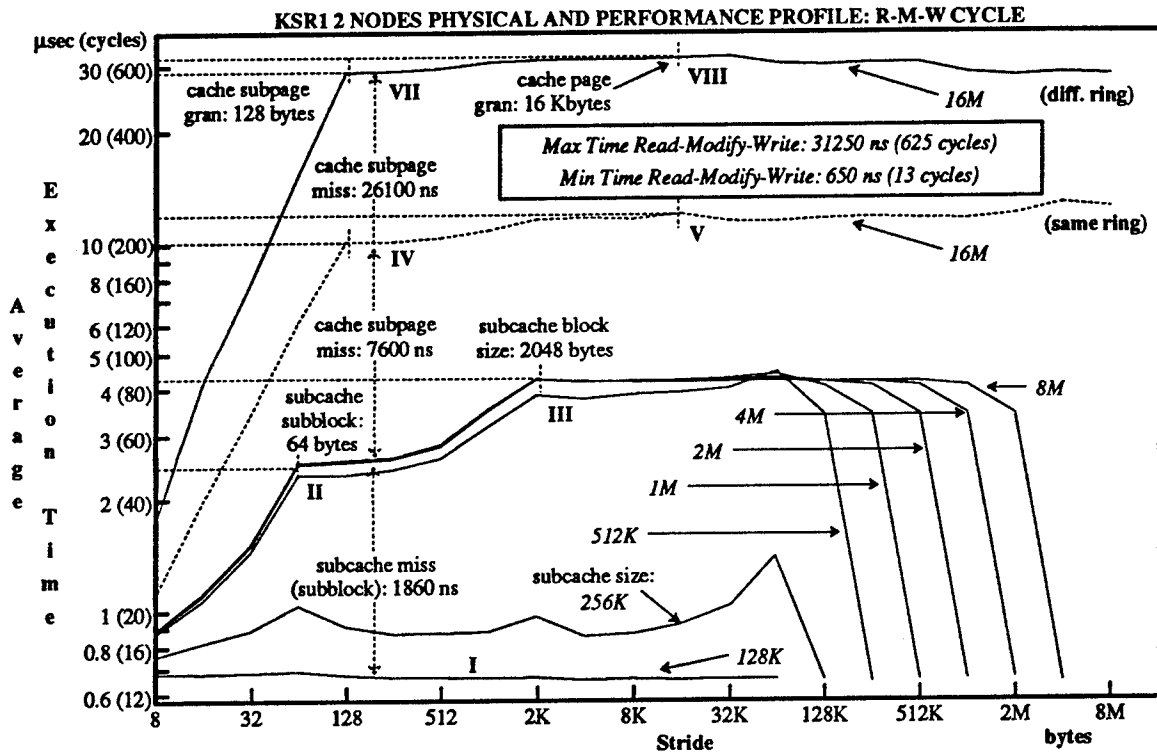
Figure 5: Physical and performance profiles of the KSR1 subcache and cache structures obtained using 2 competing nodes running R-M-W based experiments. Each regime identifies the mean execution time for a particular combination of subcache and cache miss penalties. For array sizes smaller than 16MB, there is no contention between the nodes.
