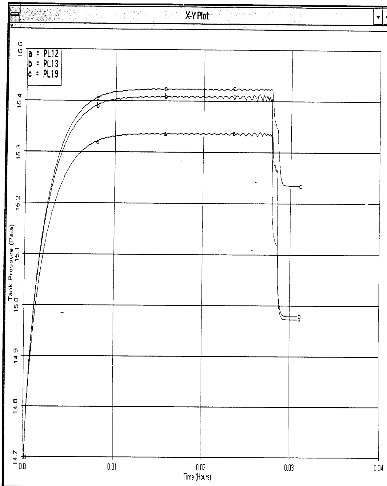
Pressure in Fuel Tanks During Refueling (a and b are side tanks, c is the center tank)
