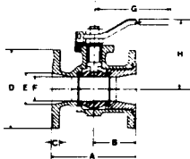
F-510 Series Configuration for 1 1/2" - 8"
