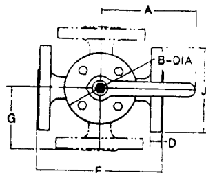
3-WAY: FLANGED
