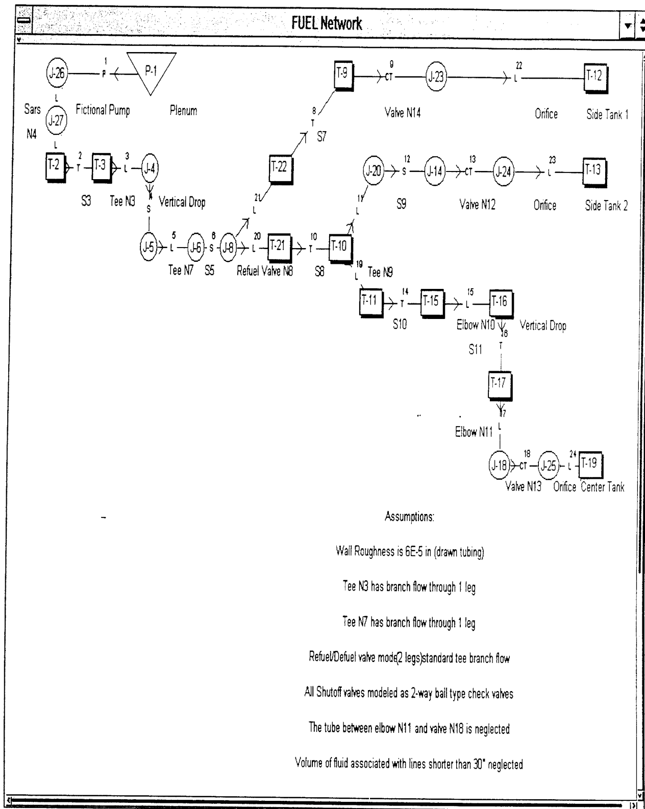
Fuel Side Scheme
