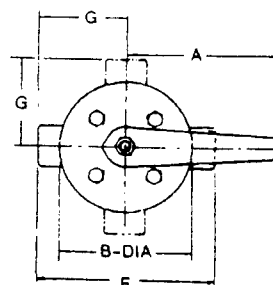
2-WAY, THREADED
