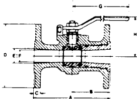
F-510 Series Configuration for 1/2" - 1"
