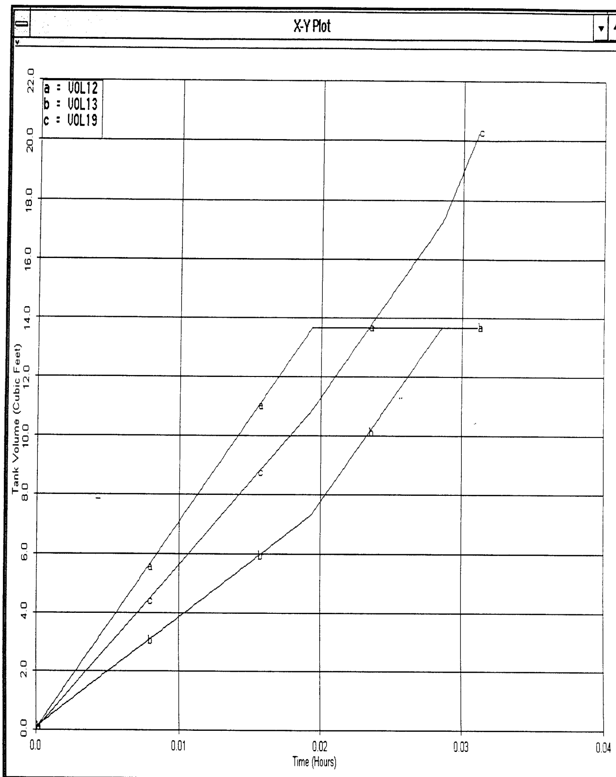
Fuel Tank Volumes as a Function of Time (a and b are side tanks, c is the center tank)
