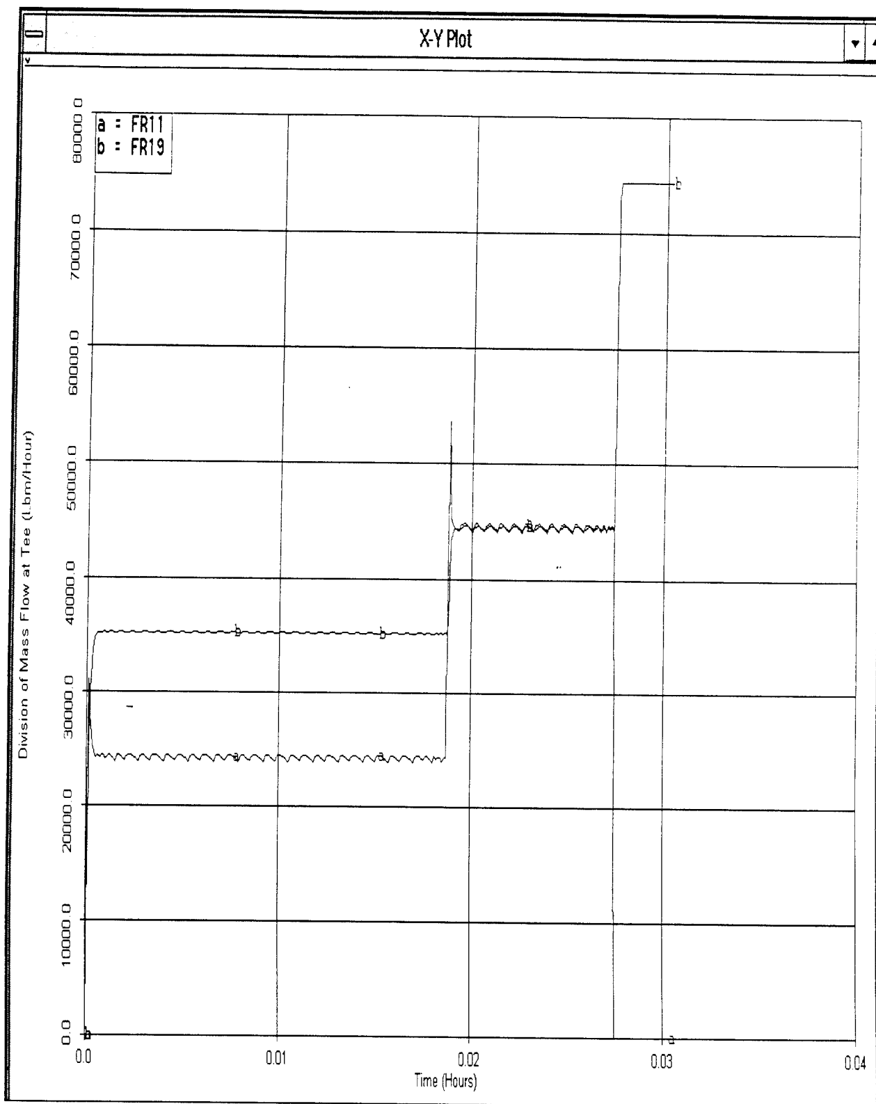
Division of Mass Flow to Side Tank 2 and the Center Tank at a Tee Fitting (a is the path to side tank 2, b is the path to the center tank)
