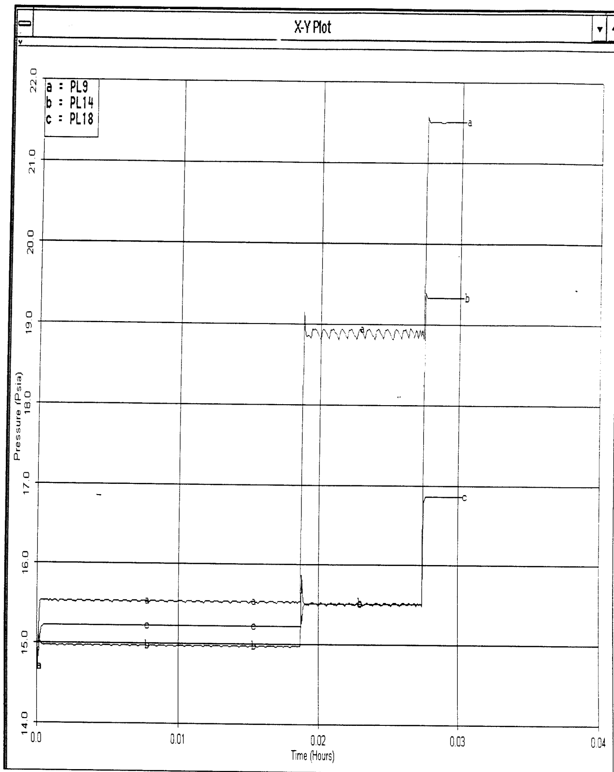
Pressure Spikes Due to Shut-off Valve Closures, Upstream Nodes (a is path to side tank 1, b is path to side tank 2 and c is path to center tank)
