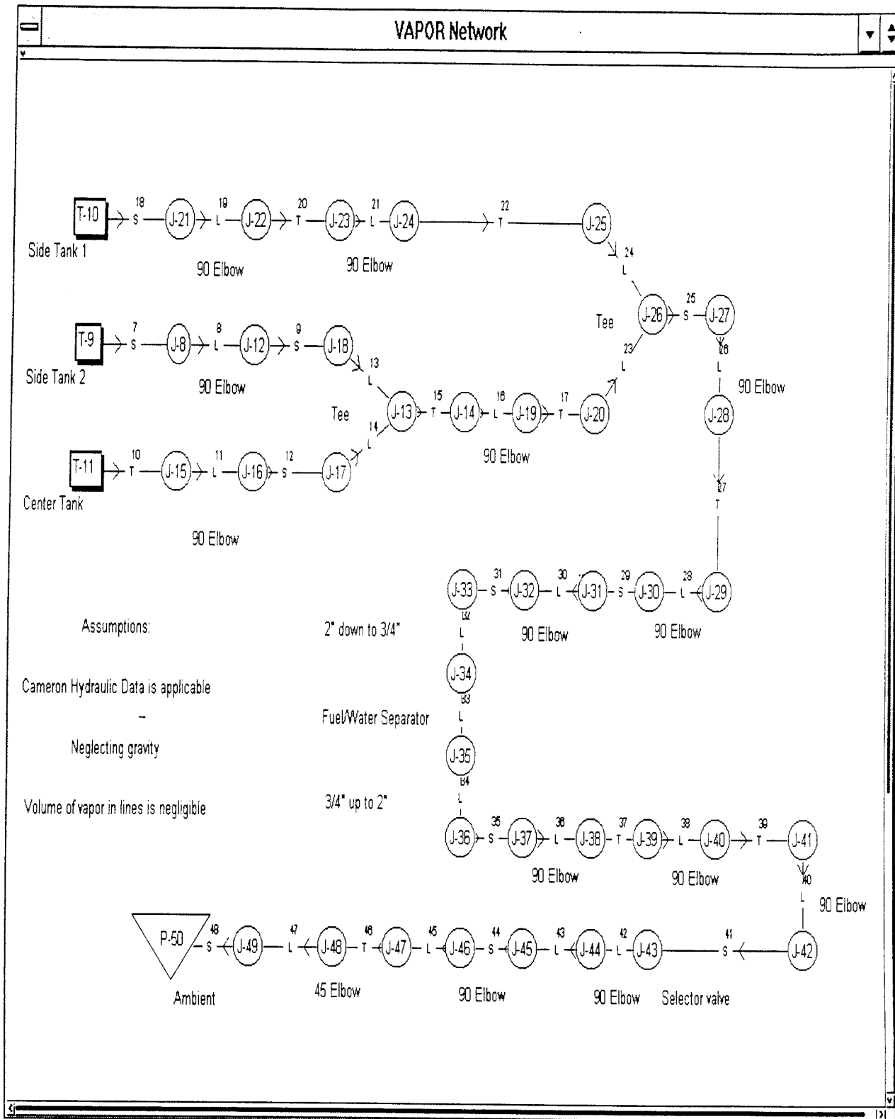
Vapor Side Scheme
