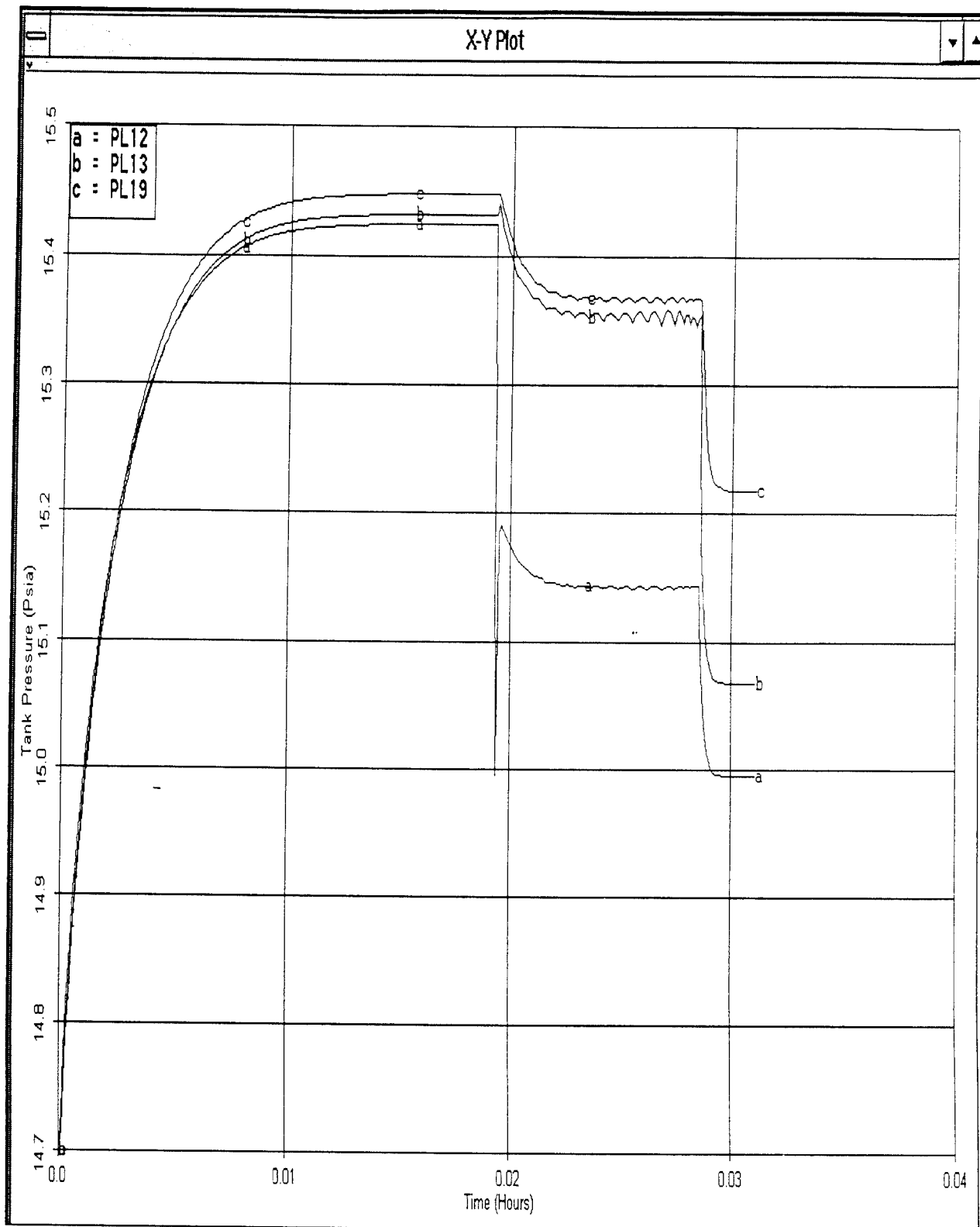
Pressure in Fuel Tanks During Refueling (a and b are side tanks, c is the center tank)
