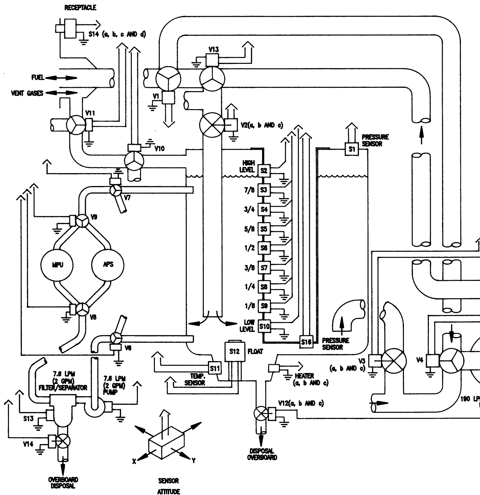
FARV FUEL SYSTEM CONTR
