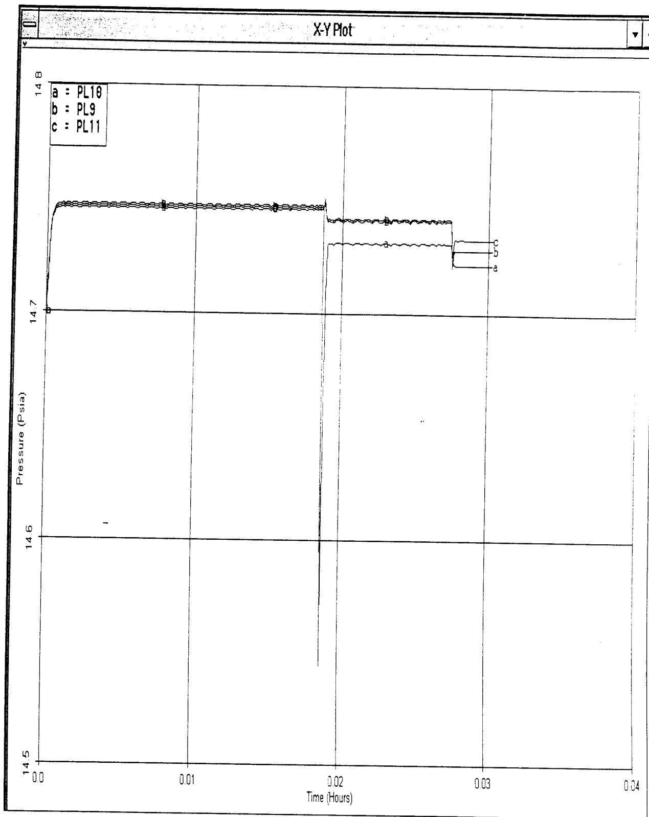
Pressure of Vapor in Tanks During Refueling (a and b are side tanks, c is the center tank)
