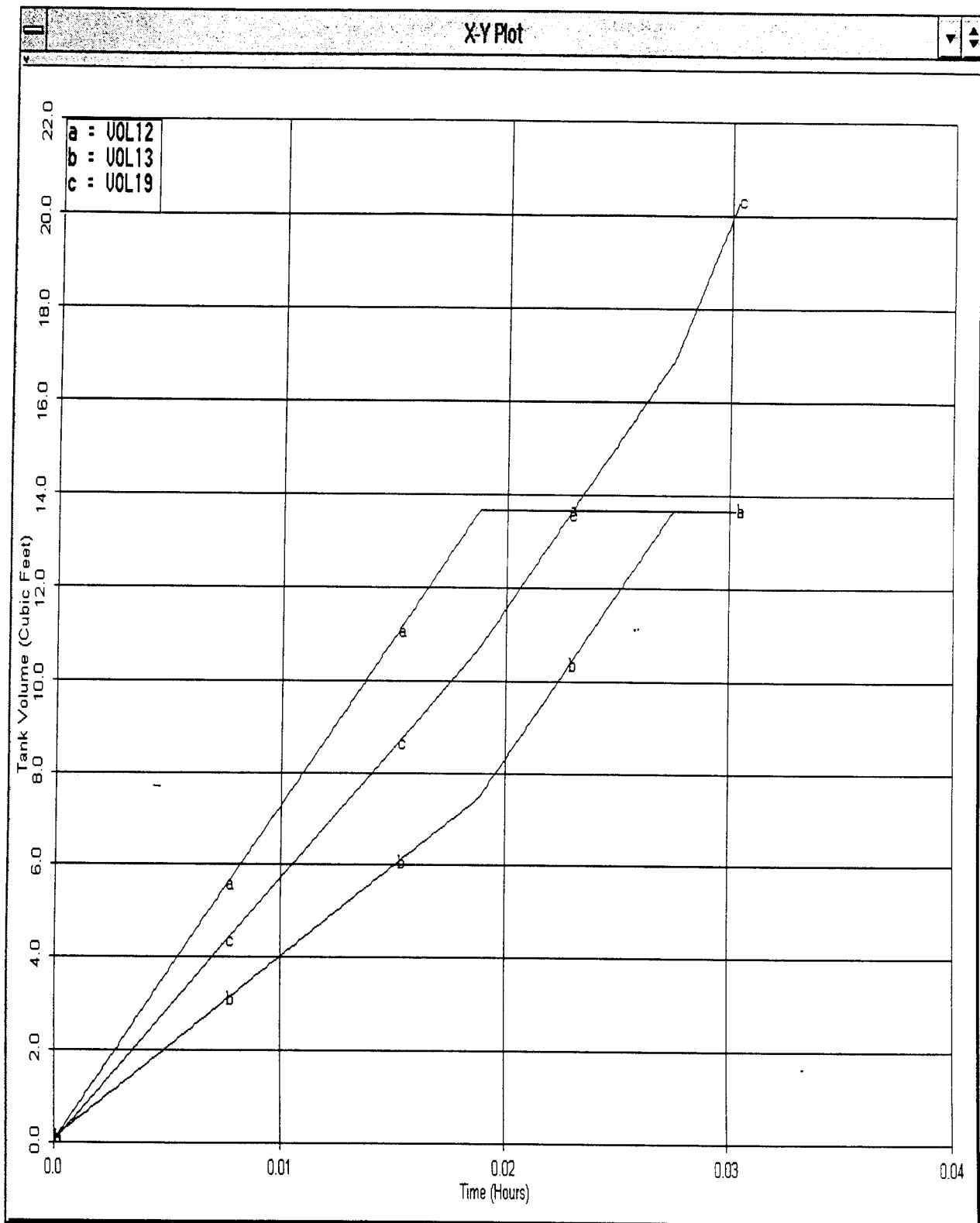
Fuel Tank Volumes as a Function of Time (a and b are side tanks, c is the center tank)
