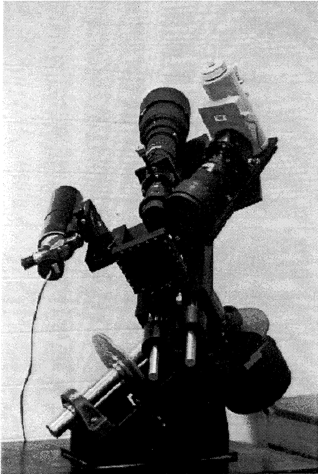
Figure 2: The wide field spectral imager ( WISPI ) with its covers removed to show the internal optical system. Light from the sky enters the large 400 mm lens at top center, is imaged on the slit, collimated by the smaller 180 mm lens, and diffracted by the grating at the bottom toward the 200 mm lens and CCD camera on the right. The Questar tracking telescope is on the left.
