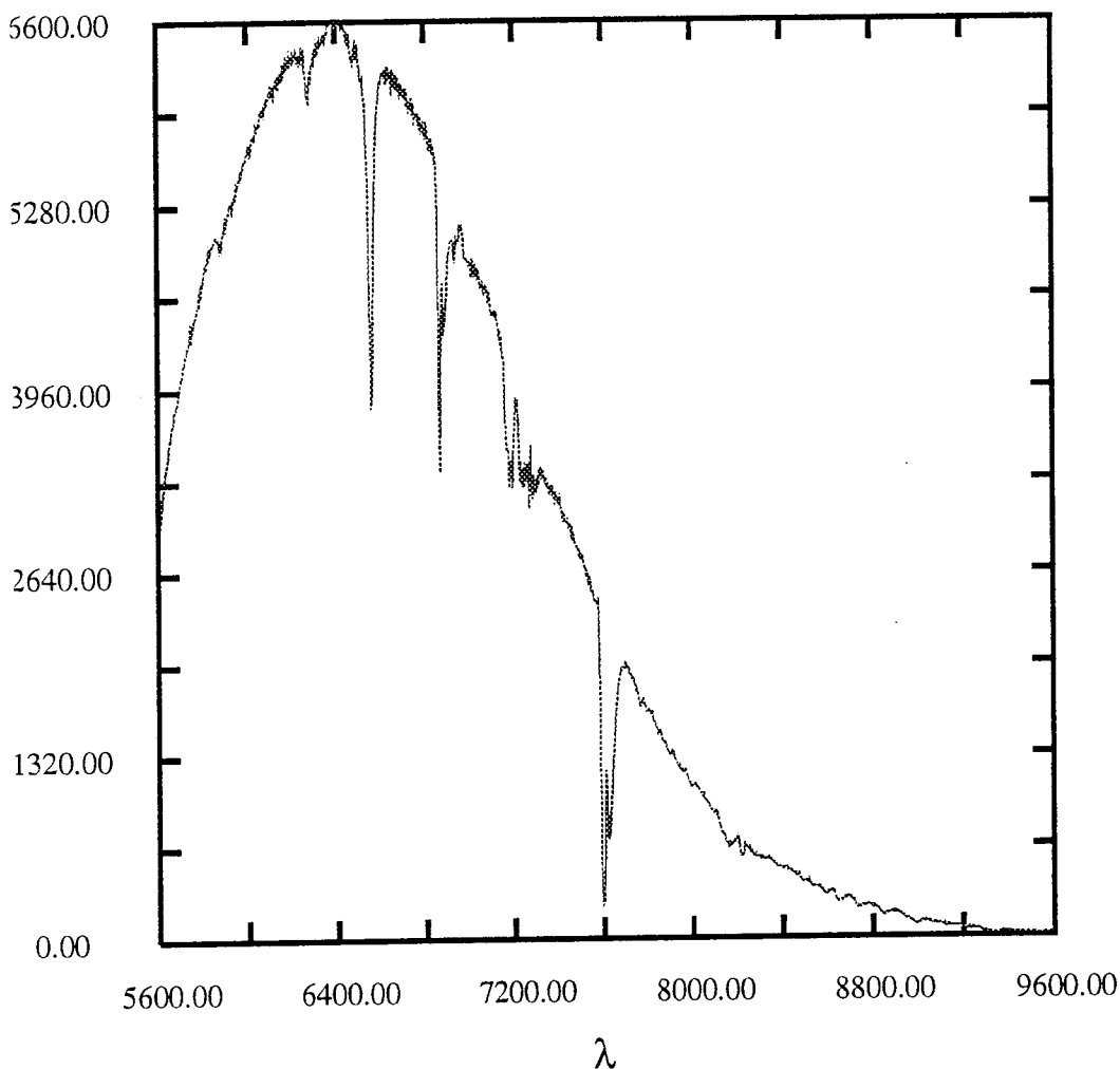
Figure 3: The spectrum of Vega recorded with WISPI . The wavelength ( \lambda ) scale is in \text{\AA} ; the raw signal is in units of (ADU's) per second. One ADU is equivalent to 6.7 detected photons.
