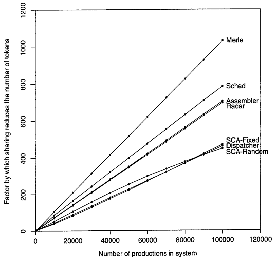
Figure 3.5: Reduction in tokens due to sharing.
