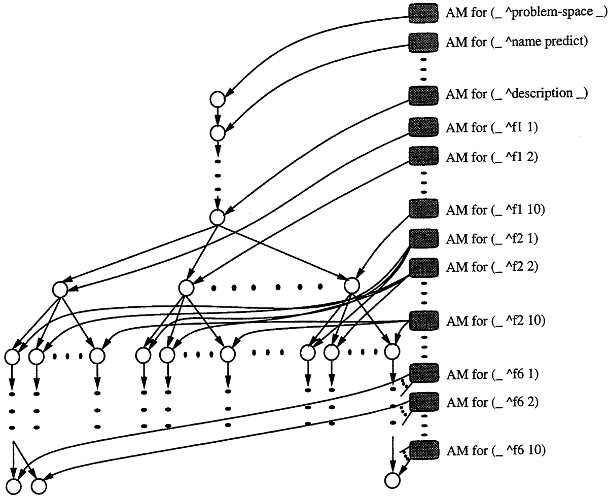
Figure 6.1: Simplified view of the Rete network for SCA-Fixed.
