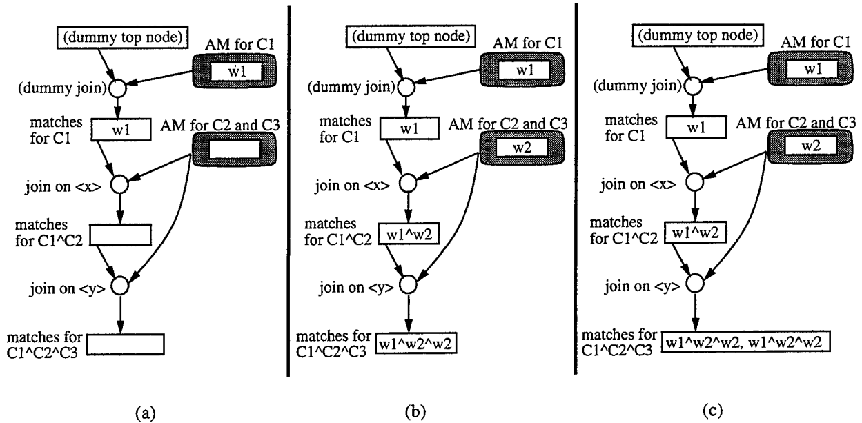
Figure 2.5: Duplicate tokens arising when join nodes are activated from the same alpha memory in the wrong order: (a) before addition of w_2 to the alpha memory; (b) after right activation of the join on \langle x \rangle and subsequent processing, but before right activation of the join on \langle y \rangle ; (c) after right activation of the join on \langle y \rangle .
