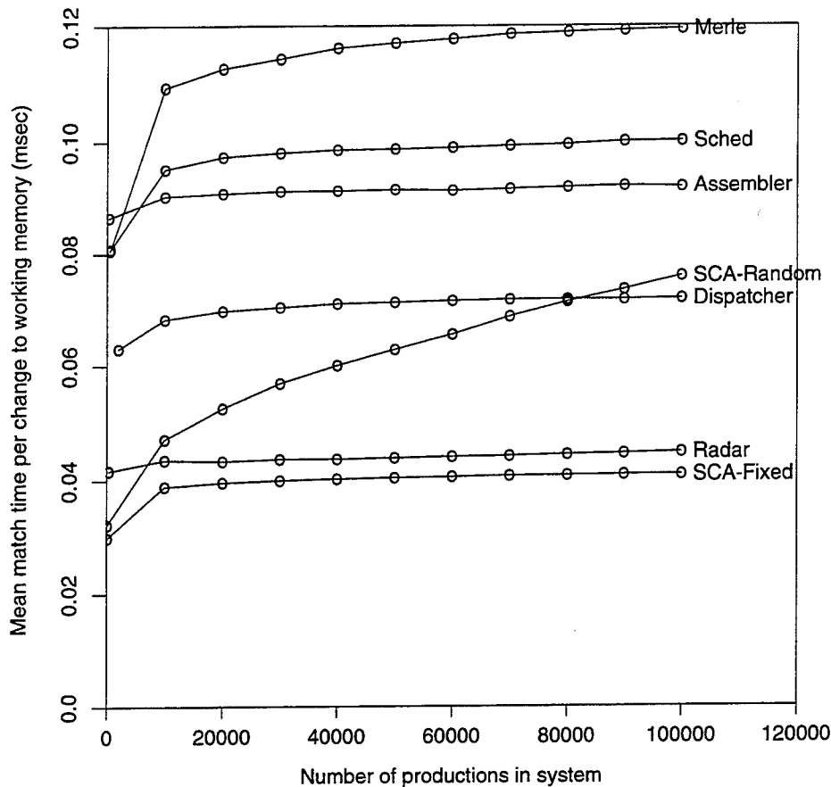
Figure 5.8: Match cost with Rete/UL.
