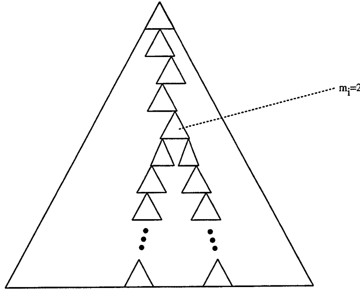
Figure 6.2: The levels and structures model. At any given time, only a few small subnetworks out of the whole beta network contain tokens.
