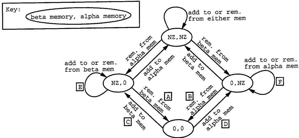
Figure 5.5: Possible states of a join node and its alpha and beta memories.
