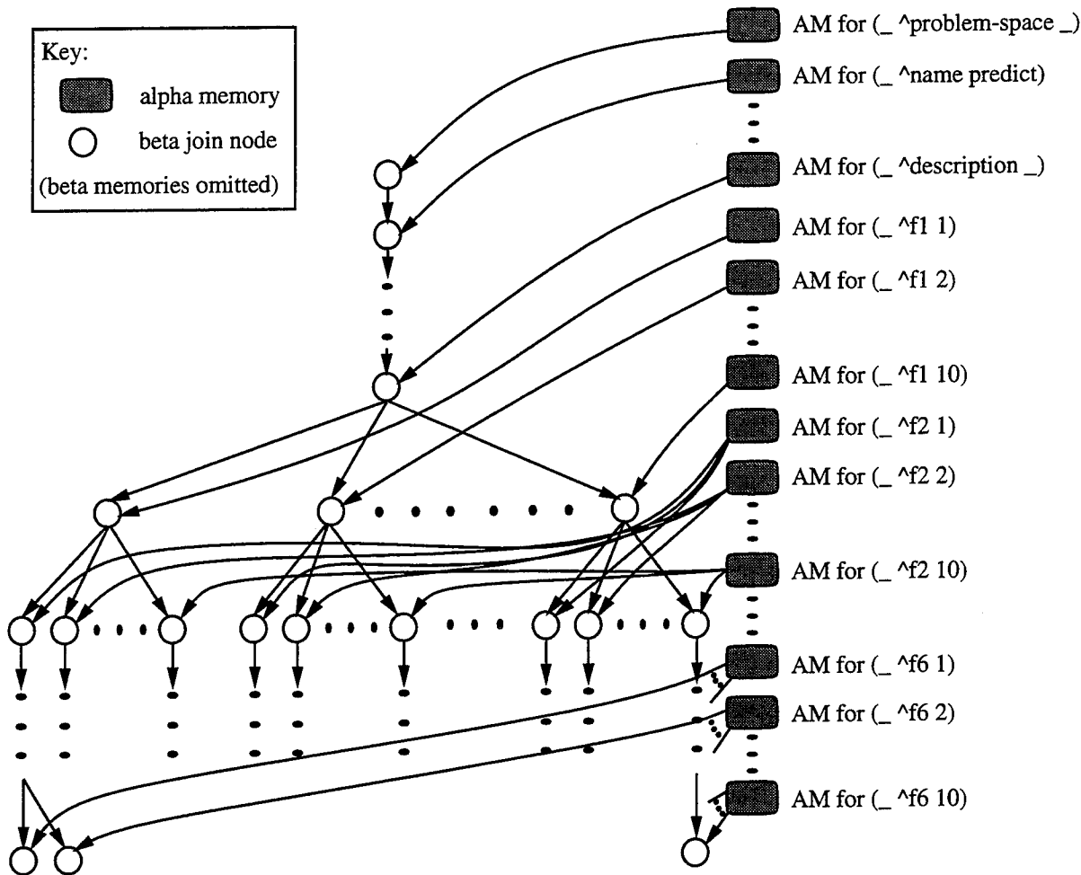
Figure 4.1: Simplified view of the Rete network for SCA-Fixed.
