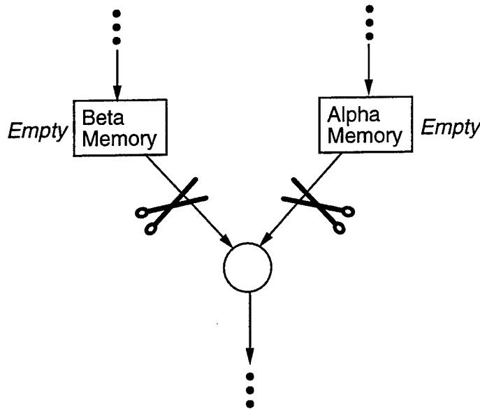
Figure 5.4: Unlinking a join node from both its alpha memory and its beta memory at the same time, destroying the correctness of the match algorithm.
