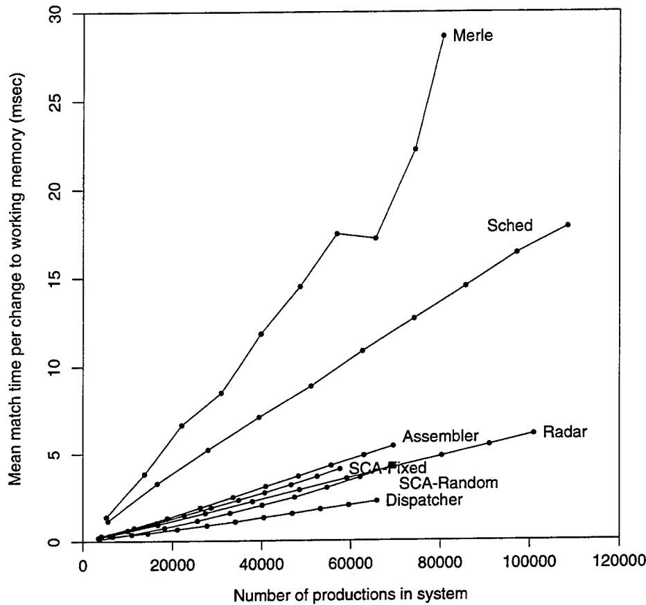
Figure 3.1: Match cost with the basic Rete algorithm.
