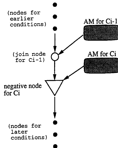
Figure 2.6: Rete network for a negative condition.
