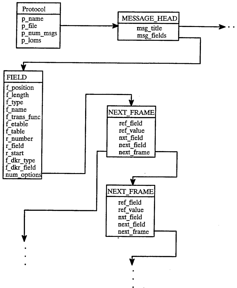
Figure 4. Translated message data structure.
