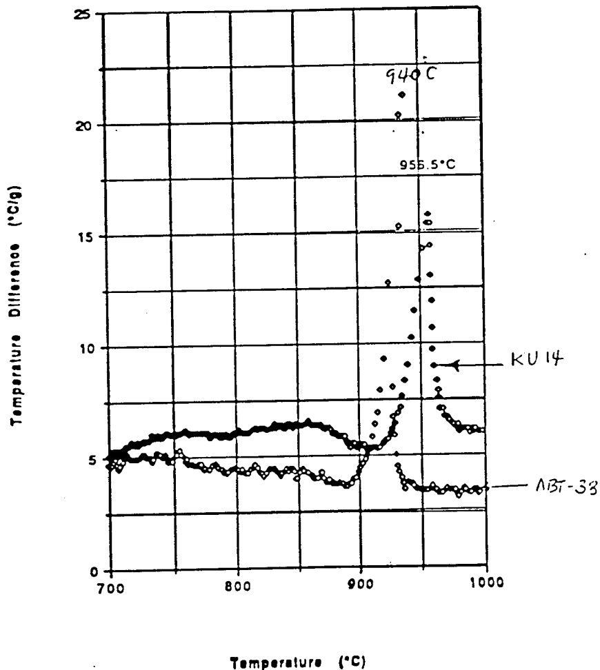
Figure II.1: DTA plot showing the effect of the reactive filler on the crystallization of KU-14 glass.
