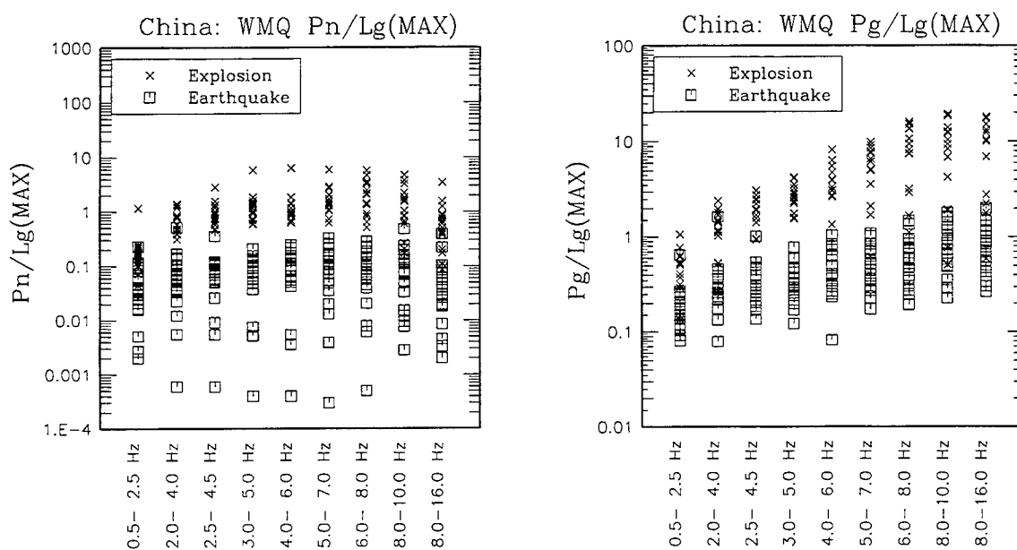
Figure 5. Scatter plots of Pn/Lg (left) and Pg/Lg (right) in nine frequency bands, after applying distance corrections, for 17 nuclear explosions and 23 earthquakes recorded by station WMQ.
