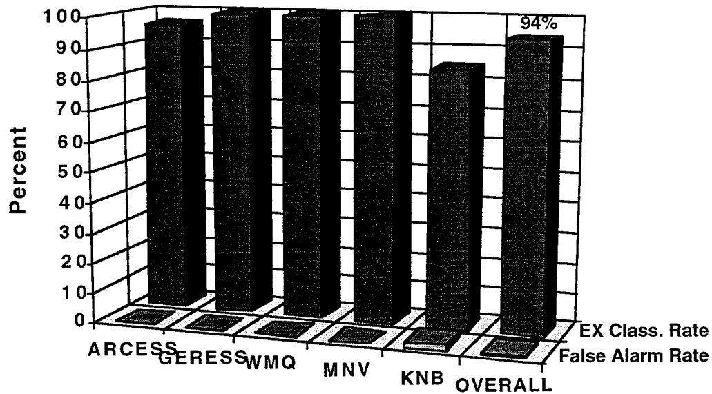
Figure 25. Summary of classification results at ARCESS, GERESS, WMQ, MNV and KNB. Results are expressed in terms of the percentage of explosions correctly classified and the false alarm rate at each station. Overall results are shown on the far right.
