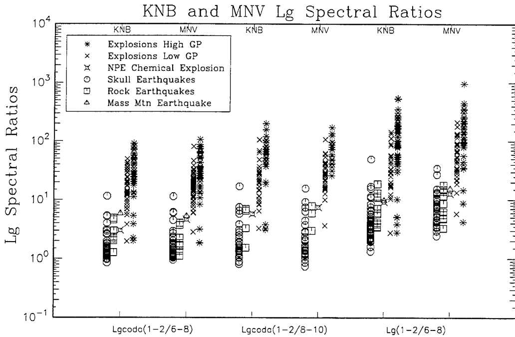
Figure 15. Scatter plots of Lg spectral ratio measurements of three different types for seismic events recorded by LNN stations KNB and MNV. Events are separated into subgroups as in Figure 13.
