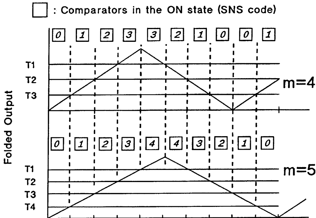
Figure 1. Optimum SNS Folding Waveforms and Output Codes for m_1 = 4 and m_2 = 5 .
