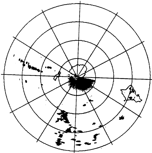
FIGURE A-7. TEST D-21, MINIMUM DETECTION VERIFICATION TEST. South Kauai provides a minimum detection capability of at least 0 dB SNR (bottom) for a -8 dBz target at 50 km. (Top plot shows detection capability of a non-zero dB SNR for same target.) Weather cell in SSE sector measures approx. 35 dBz, and is approx. 130 km from radar. Each range ring equals 30 nautical miles (approx. 55.5 km).
