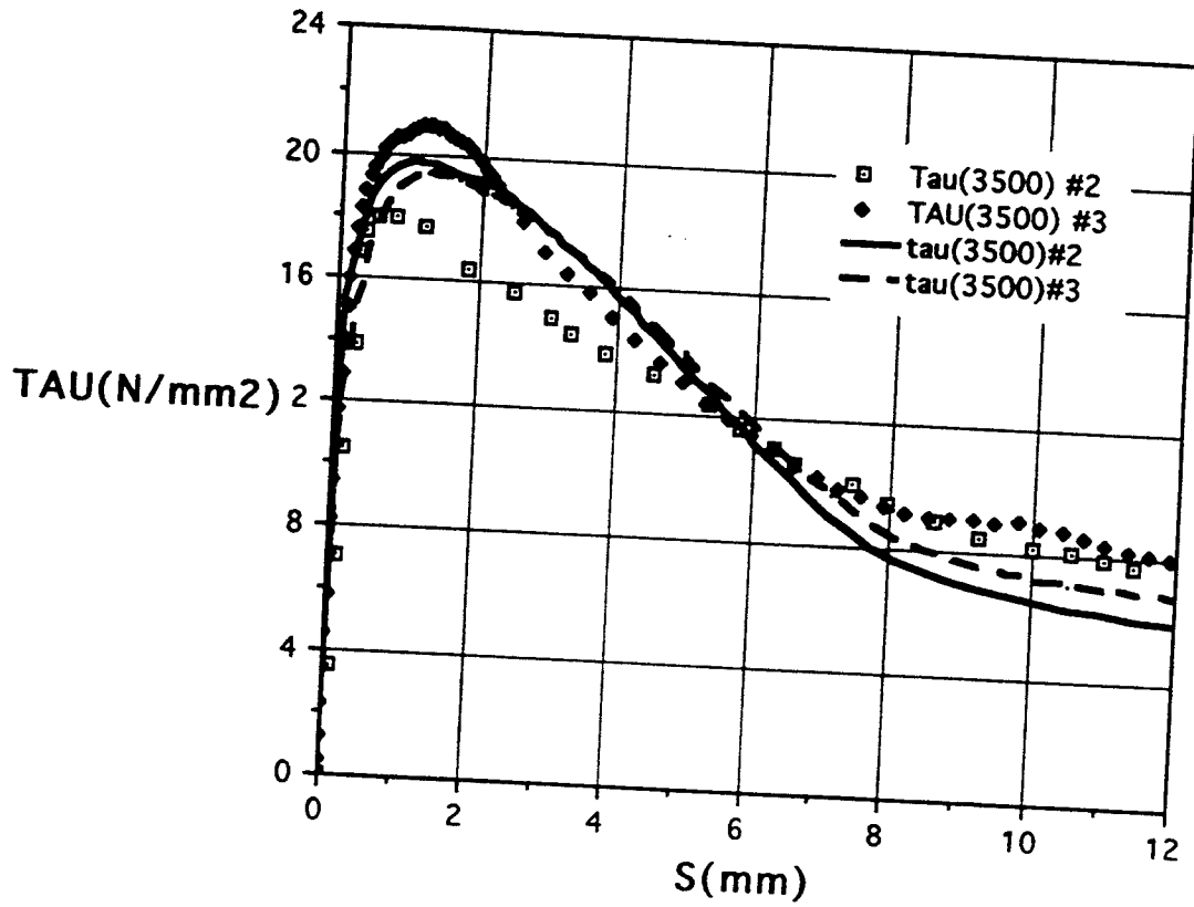
Figure 34. Model Predictions of Bond Stress vs. Slip - Malvar's Test 3500 psi Level
