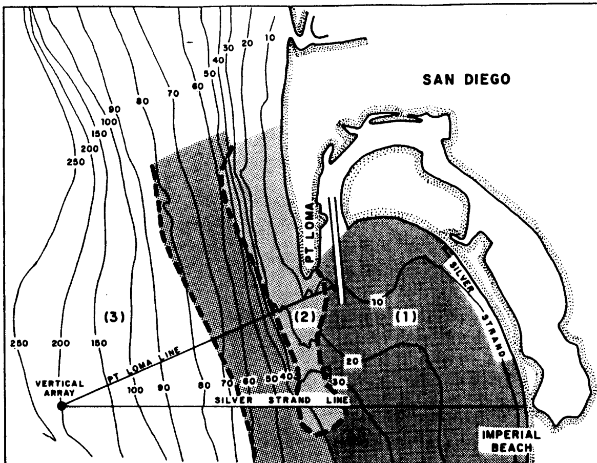
Figure 21. Paths along which propagation loss was modelled for comparison - San Diego Bight. Geoacoustic regions (from McCulloch and Greene (90)): (1) unconsolidated deposits of Quaternary age (2) undifferentiated sedimentary rocks of Late Cretaceous age, and (3) sediment and sedimentary rock of Quaternary and Tertiary (Pliocene and Miocene) age.
