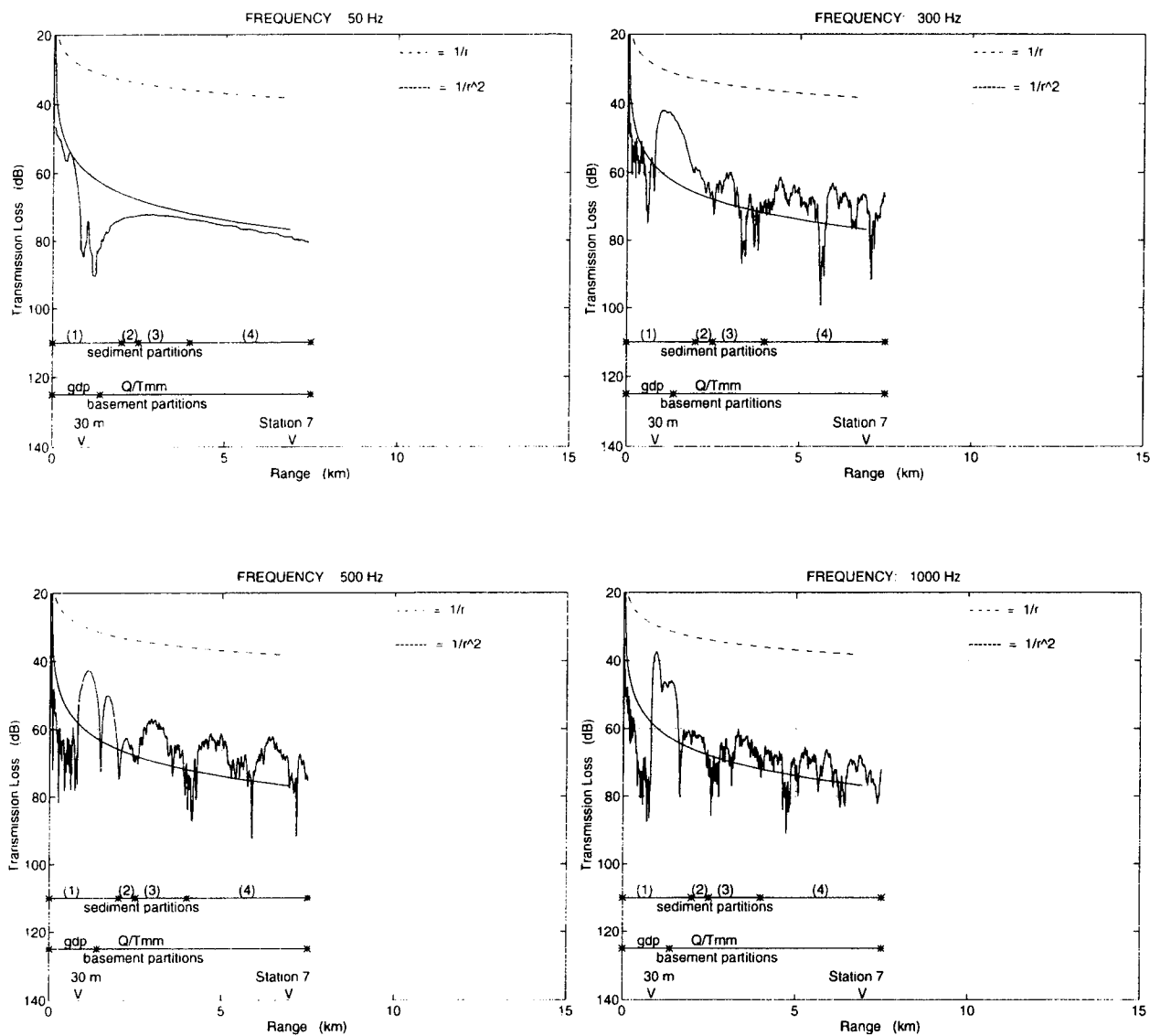
Figure 12. Transmission loss along the path from Pt Pinos to Station 7 for 50, 300, 500, and 1000 Hz. Sediment types: (1) no sediment, (2) 1 m coarse sand, (3) 1 m clayey silt, (4) 2 m clayey silt. (Receiver depth 30 m.)
