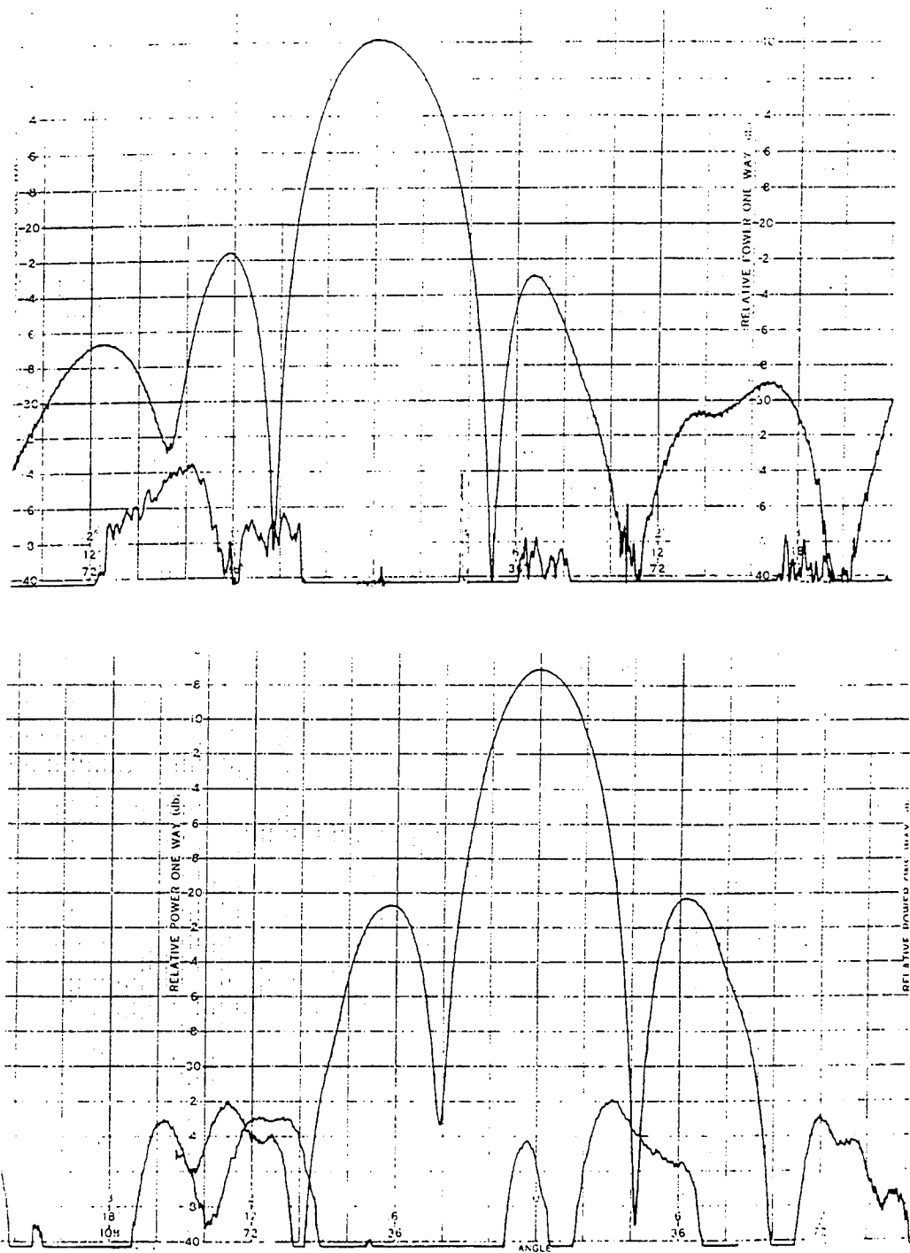
Figure 7 - The radiation patterns of the antenna shown in Figure 4. a. H-plane b. E-plane
