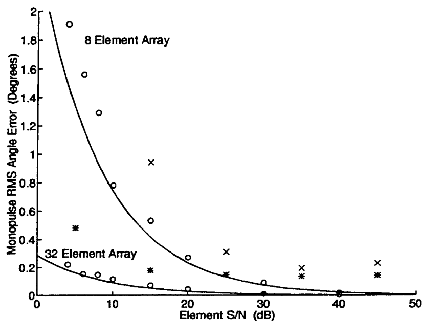
Figure 4: Monopulse DF performance for both the 8 and 32 element arrays. Circles indicate simulated data performance. Measured data performance is indicated by an x for the 8 element array and by an * for the 32 element array. The solid curves are calculated from Equation 6 for 8 or 32 elements and represent the theoretical monopulse rms error limits.
