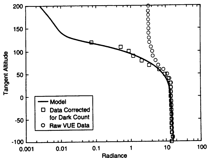
Figure 37. Comparison of Normalized VUE Radiance Data with Atmospheric Model (Excerpted from Pritt [31].)
