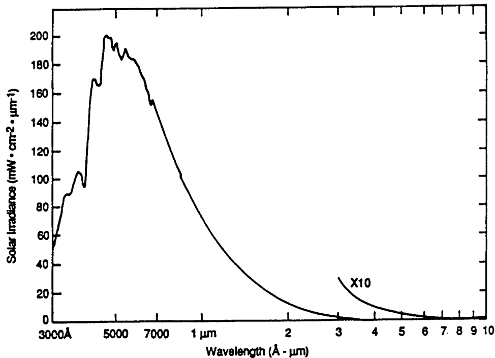
Figure 1. The Solar Spectral Irradiance for Wavelengths Longer than 3000Å. The data between 3000Å and 3 \mu\text{m} are from Labs and Nickel and from Thekaekara above 3 \mu\text{m} . These data are from a summary given by Pierce and Allen [5]. (Excerpted from Hall et al. [1]).
