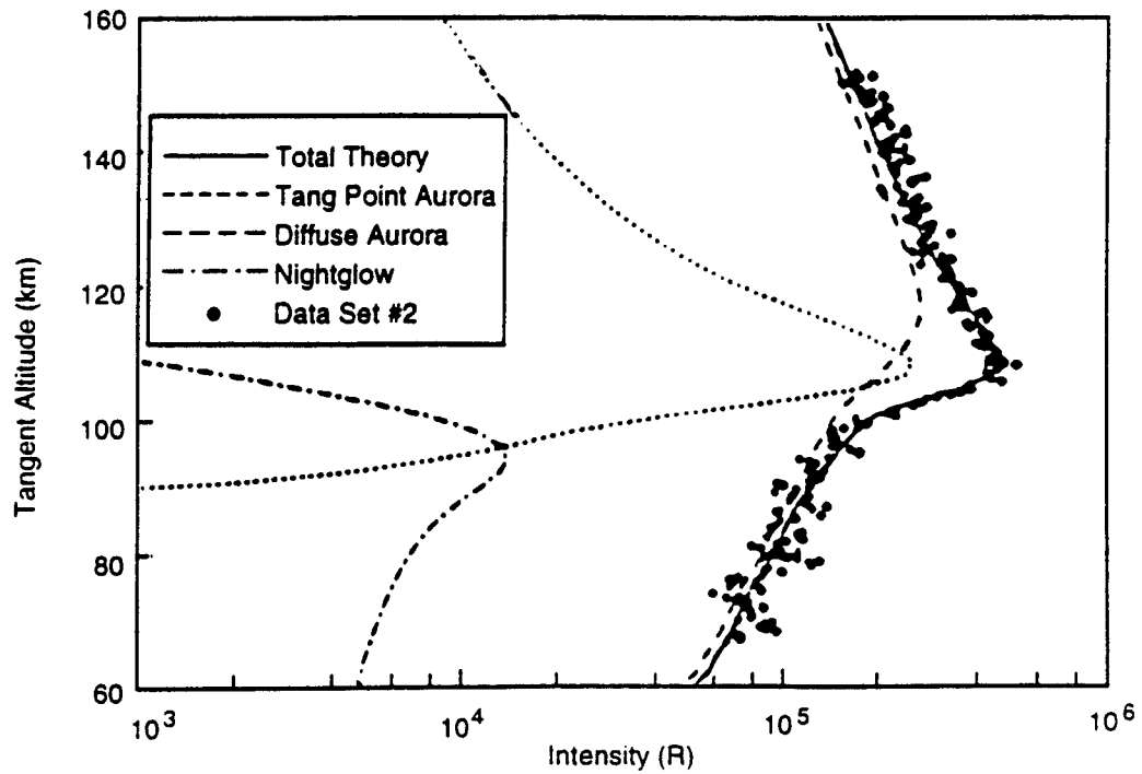
Figure 40. Vertical Emission Profiles from an Auroral Image. (a) Auroral profile #1 for orbit 2570, filter TC; (b) Auroral profile #2 for orbit 2570, filter TC. (Excerpted from Smathers et al. [5].)
