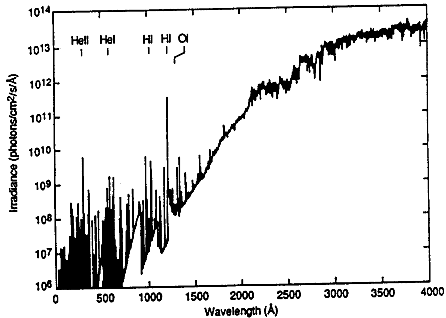
Figure 3. Composite Solar Spectral Irradiance for Solar Minimum Conditions. SUSIM data at 1.5Å resolution [8] are used from 1207 to 4000Å. These data were obtained during the Spacelab 2 mission in July 1985. From 18 to 1100Å, the Hinteregger et al. [9] quiet-Sun reference spectrum (SC No. 21REF) appropriate to July 1976 is used after binning into 1Å intervals. The Donnelly and Pope [10] representation of weak lines, superimposed on strong lines from the SC No. 21REF tabulation is used to fill the gap between 1100 and 1207Å. (Excerpted from Meier [3].)
