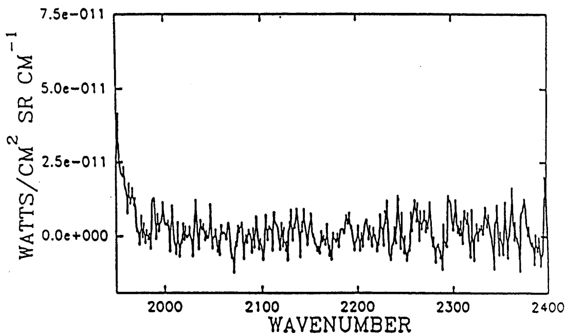
Figure 6b. Spectrum of Quiescent Night Sky Taken Just After The Spectrum Shown in Figure 6a.
