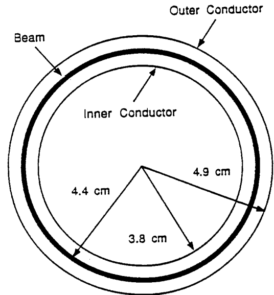
Fig. 1. Cross section of the coaxial drift space.
