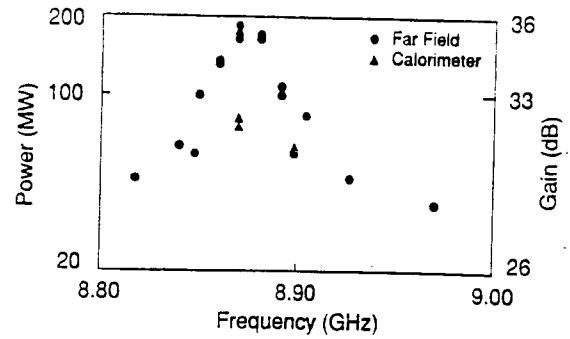
Fig. 5. Measured frequency response of the two stage amplifier. The triangles indicate calorimetric data and the circles data obtained from the far field measurements. The calorimeter output saturates at about 65 MW. Gain measurements \pm 1 dB.
