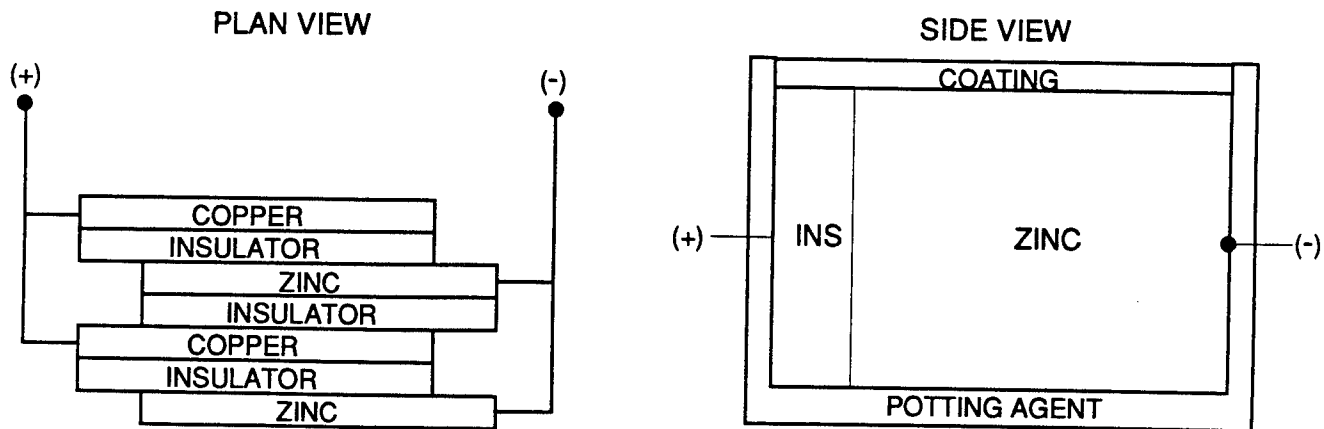
a) Bimetallic TOW approach per Mansfield, et al. 7
