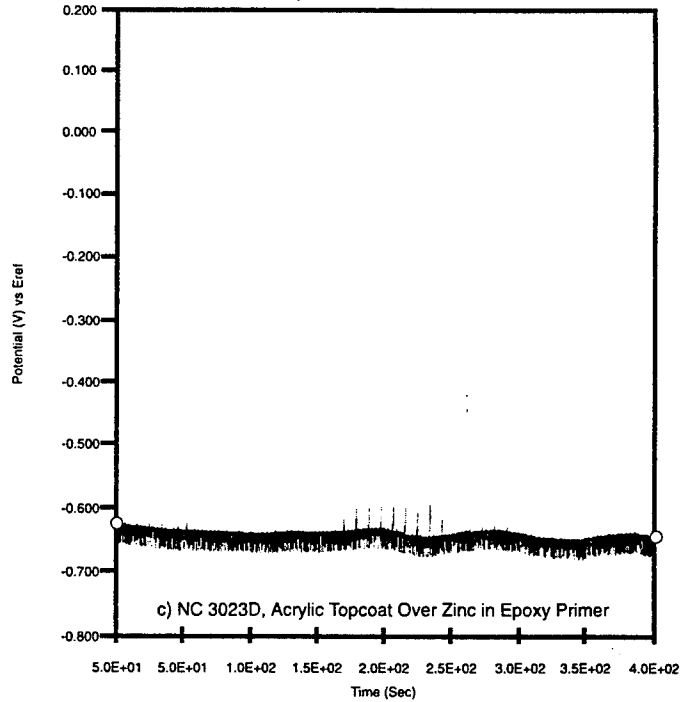
Figure 9. Potential-time runs from NCEL coatings—4.2 years continuous immersion exposure,
