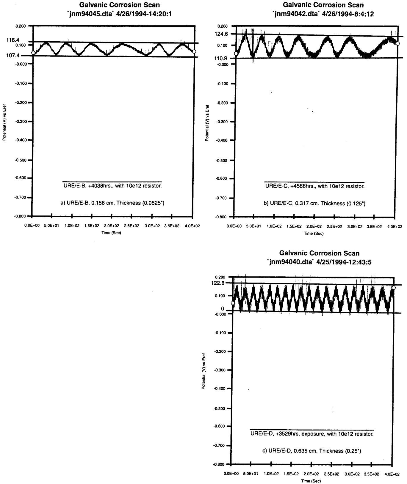
Figure 10. Potential-time runs from cast urethane coatings—0.5 years continuous immersion exposure
