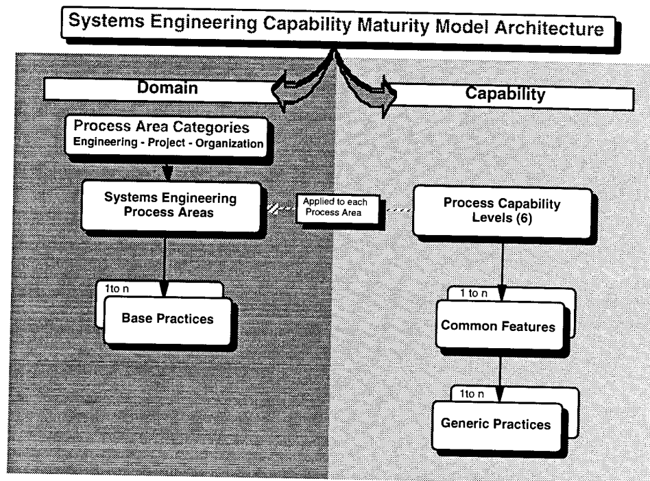
Figure 2-2. Model Architecture
