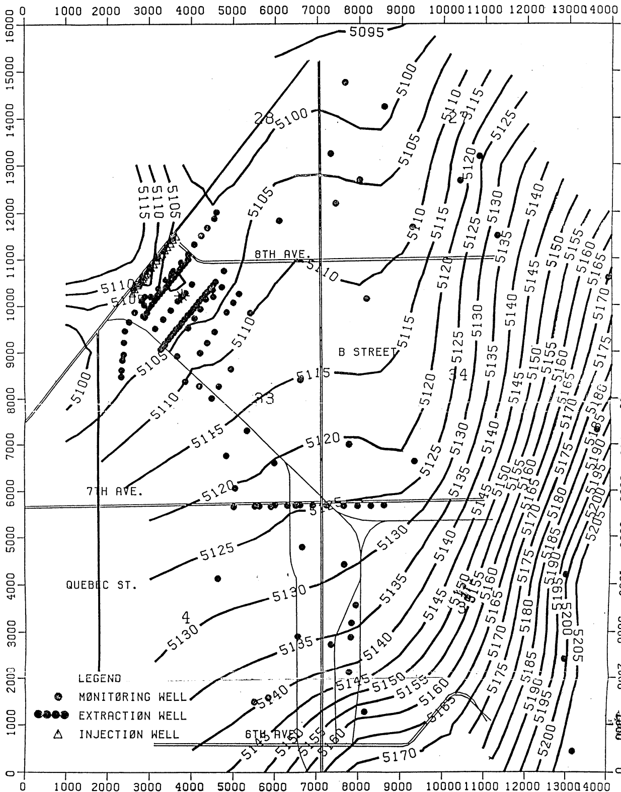
Fig. 4: Irontdale Water Level Contours 10/86 (feet above MSL)
