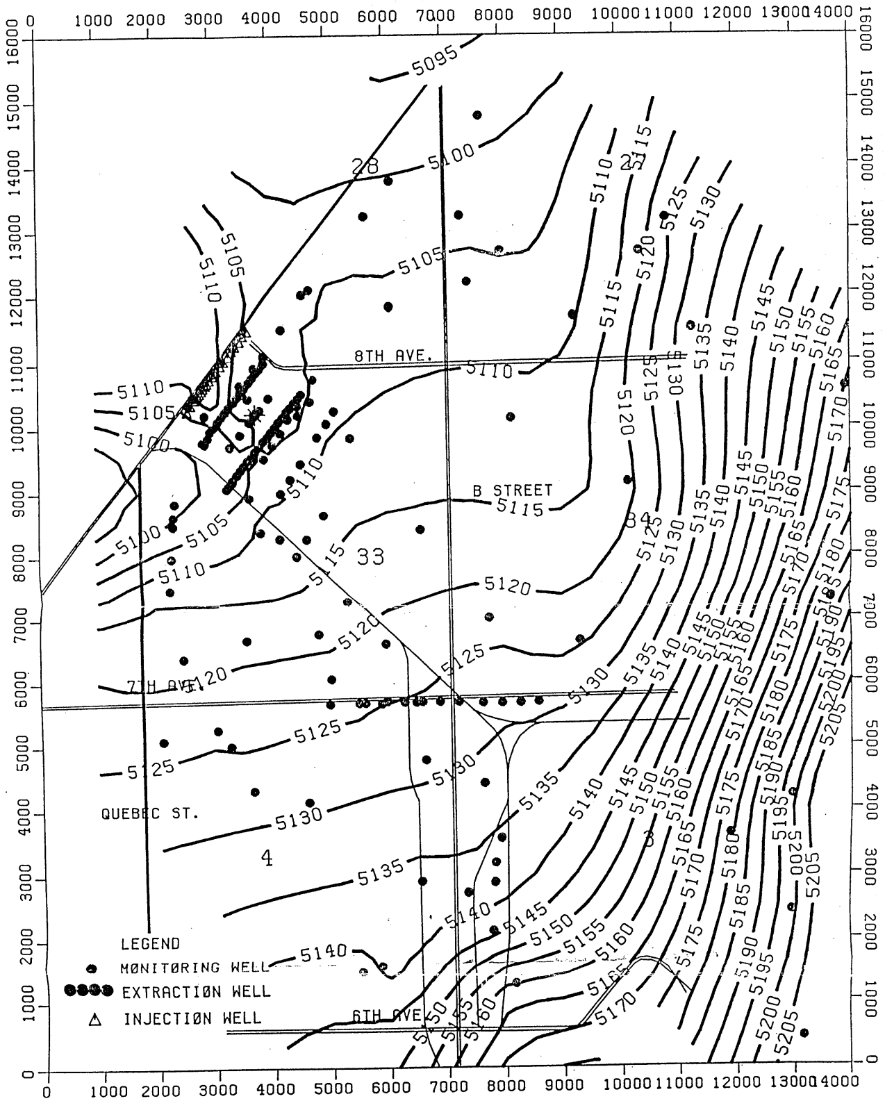
Fig. 3: Irondale Water Level Contours 7/86 (feet above MSL)
