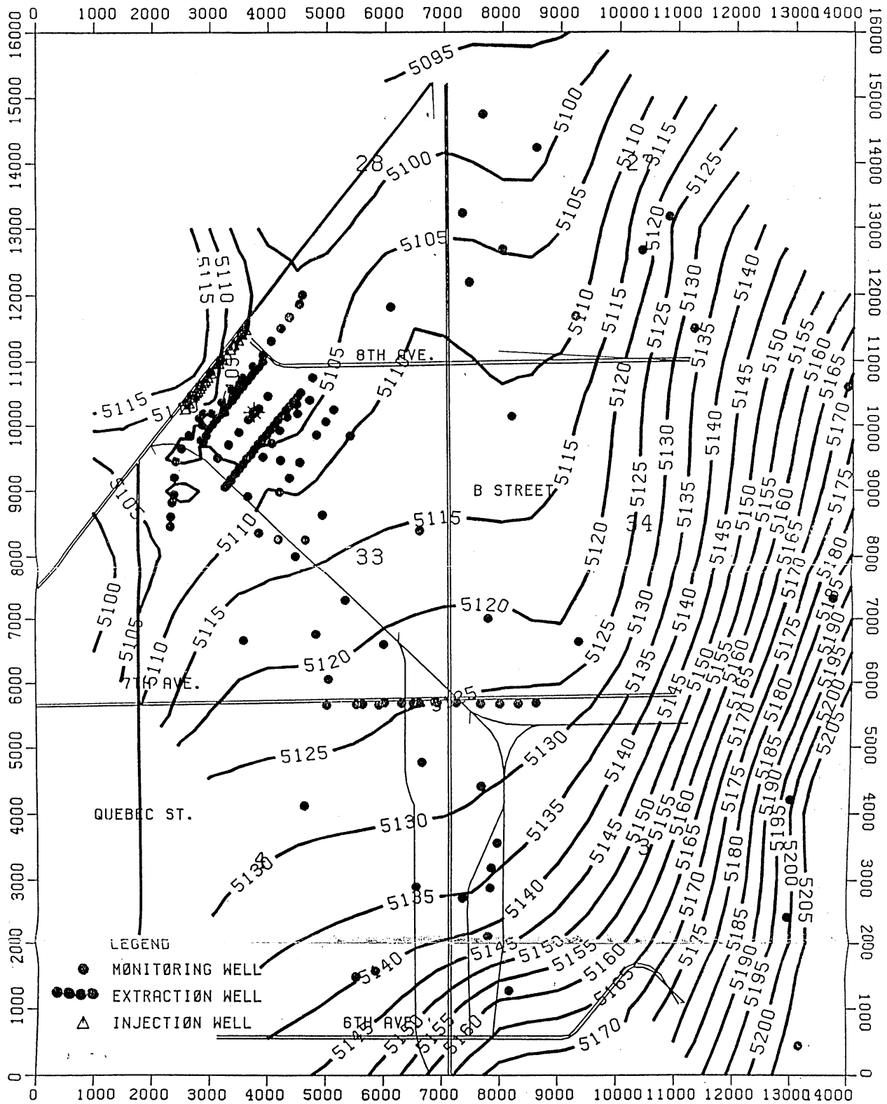
Fig. 2: Irondale Water Level Contours 4/86 (feet above MSL)
