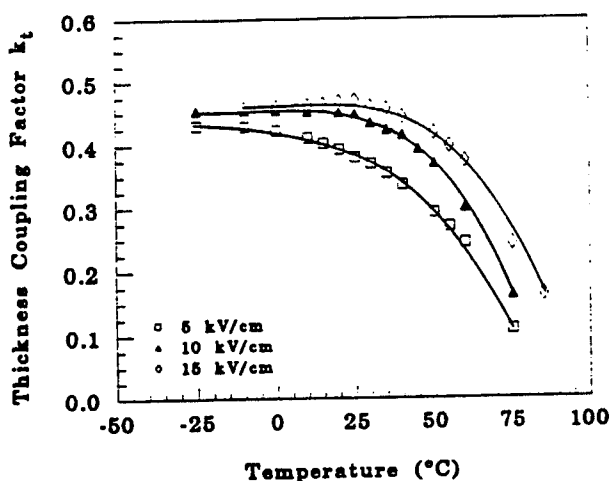
Figure 5. Temperature dependence of induced k_t at several field levels for a) 0.875PMN-0.125PT and b) 0.85PMN-0.15PT-1%La specimen.
