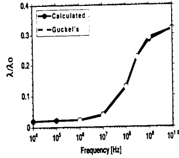
Fig. 4. Comparison of wavelength ratios \lambda/\lambda_0 for the same MIS microstrip line described in Fig. 3.
