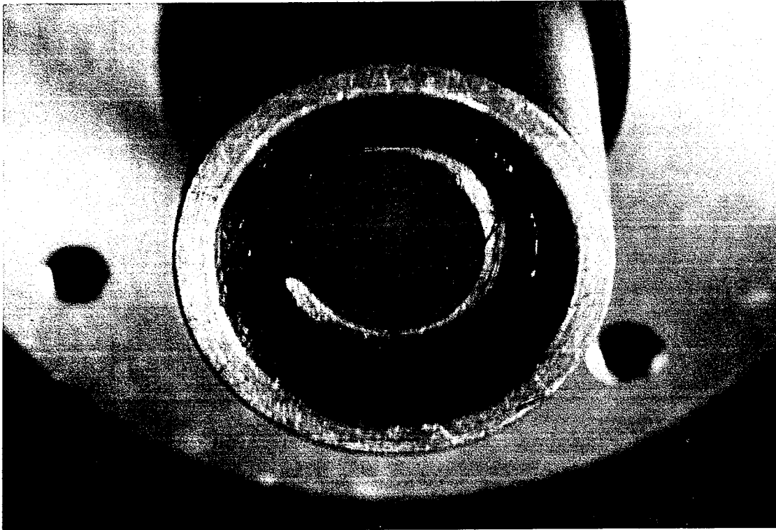
Figure 11 Circular Reed Valve with Retaining Ring
