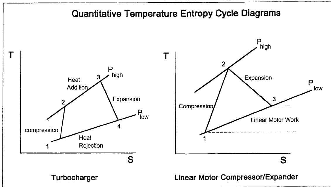
Figure 6 Comparison of Turbochargers and LMFC's on a TS Plane
