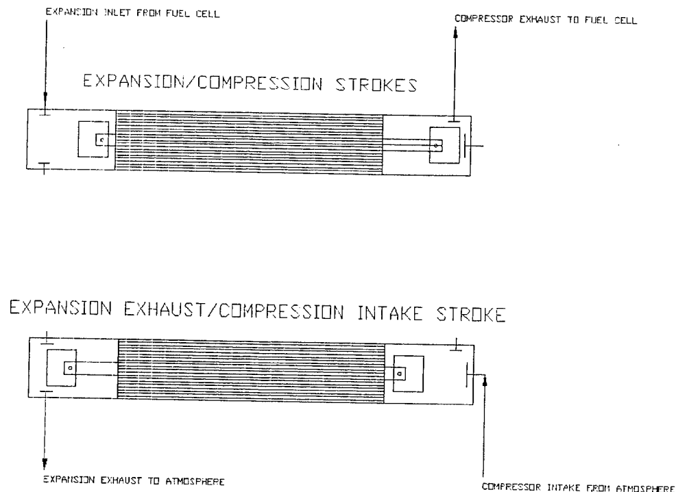
Figure 7 Cycle Schematic of LMFPC using Pressure Recovery
