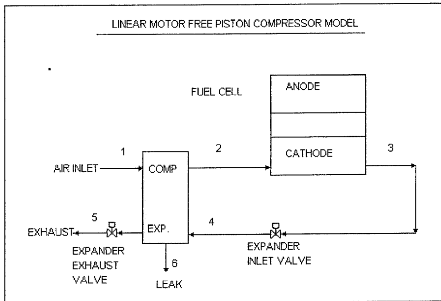
Figure 3 Linear Motor Free Piston Compressor Schematic Installation
