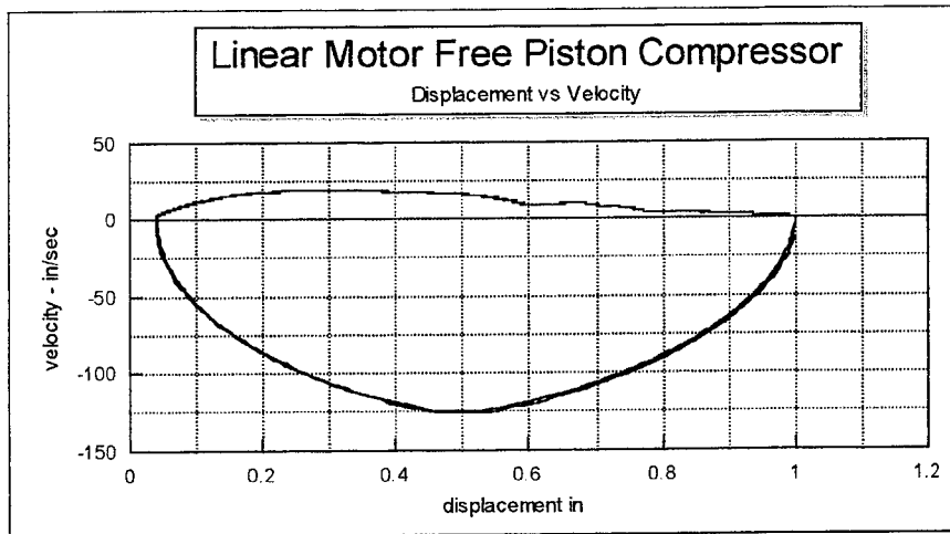
Figure 19 Phase Diagram of the LMFPC from the Simulation Code
