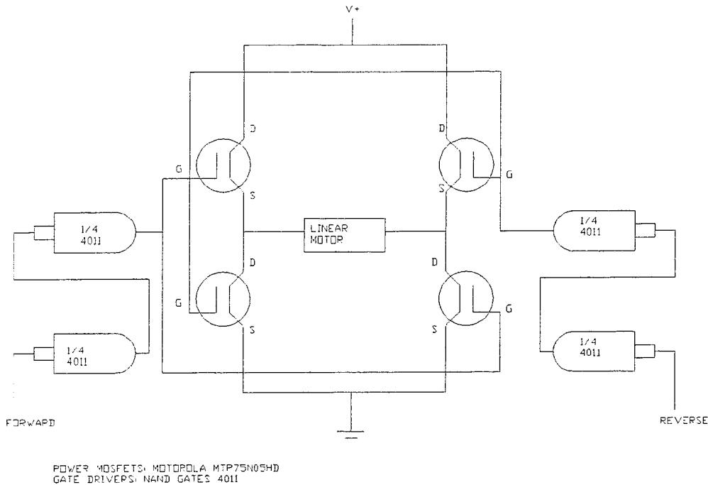
Figure 16 H Solenoid Power Circuit
