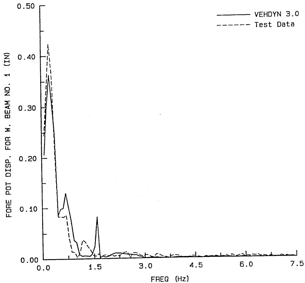
Figure A-70. Relative displacement frequency plot (frequency scale = 1.5 Hz/inch) of the forward-most axle with respect to the frame for a fully loaded HEMTT traveling at 1.81 miles per hour encountering a 3.00-inch-high obstacle.
