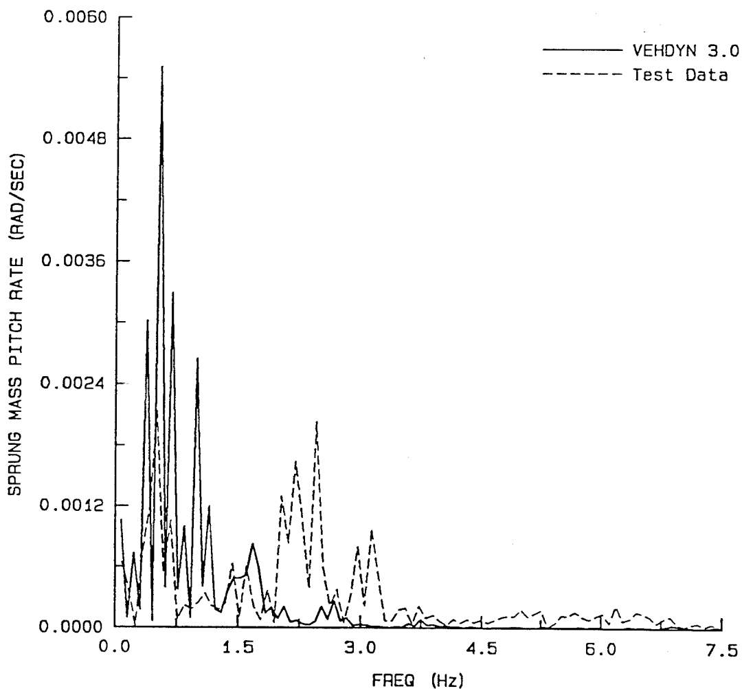
Figure A-51. Sprung mass pitch rate frequency plot for a fully loaded HEMTT traveling at 1.82 miles per hour encountering a 2.00-inch-high obstacle.
