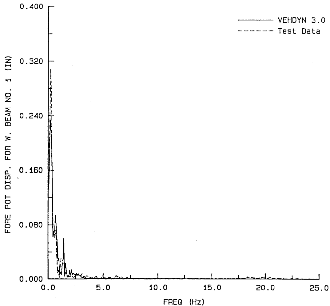
Figure A-115. Relative displacement frequency plot (frequency scale = 5.0 Hz/inch) of the forward-most axle with respect to the frame for an empty HEMTT traveling at 1.80 miles per hour encountering a 2.00-inch-high obstacle.
