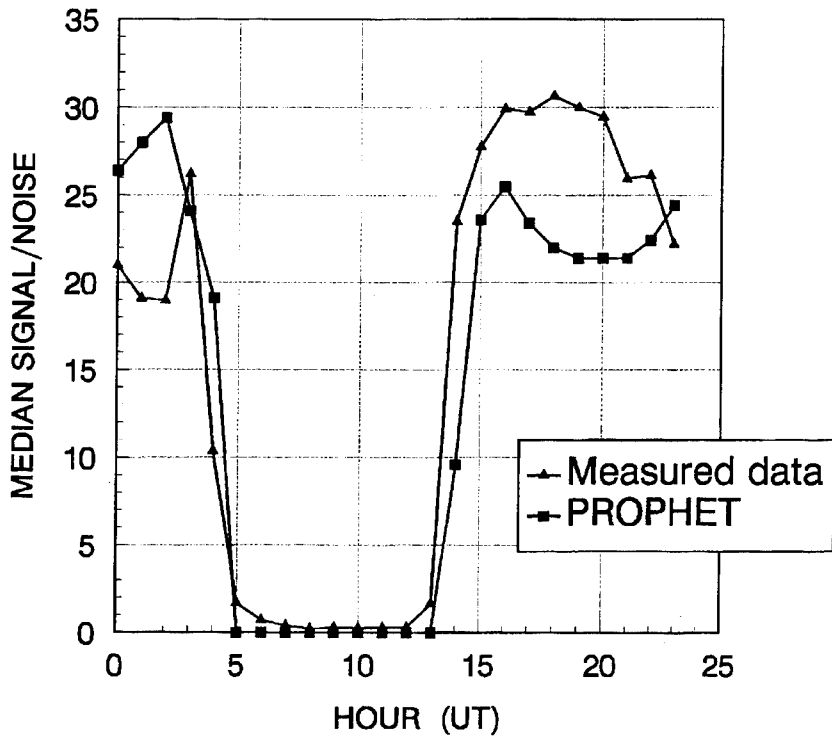
Figure 9. Median signal-to-noise ratio at 14.4 MHz for April (top) and May (bottom) 1994. Also shown are PROPHET predictions for the same period.
